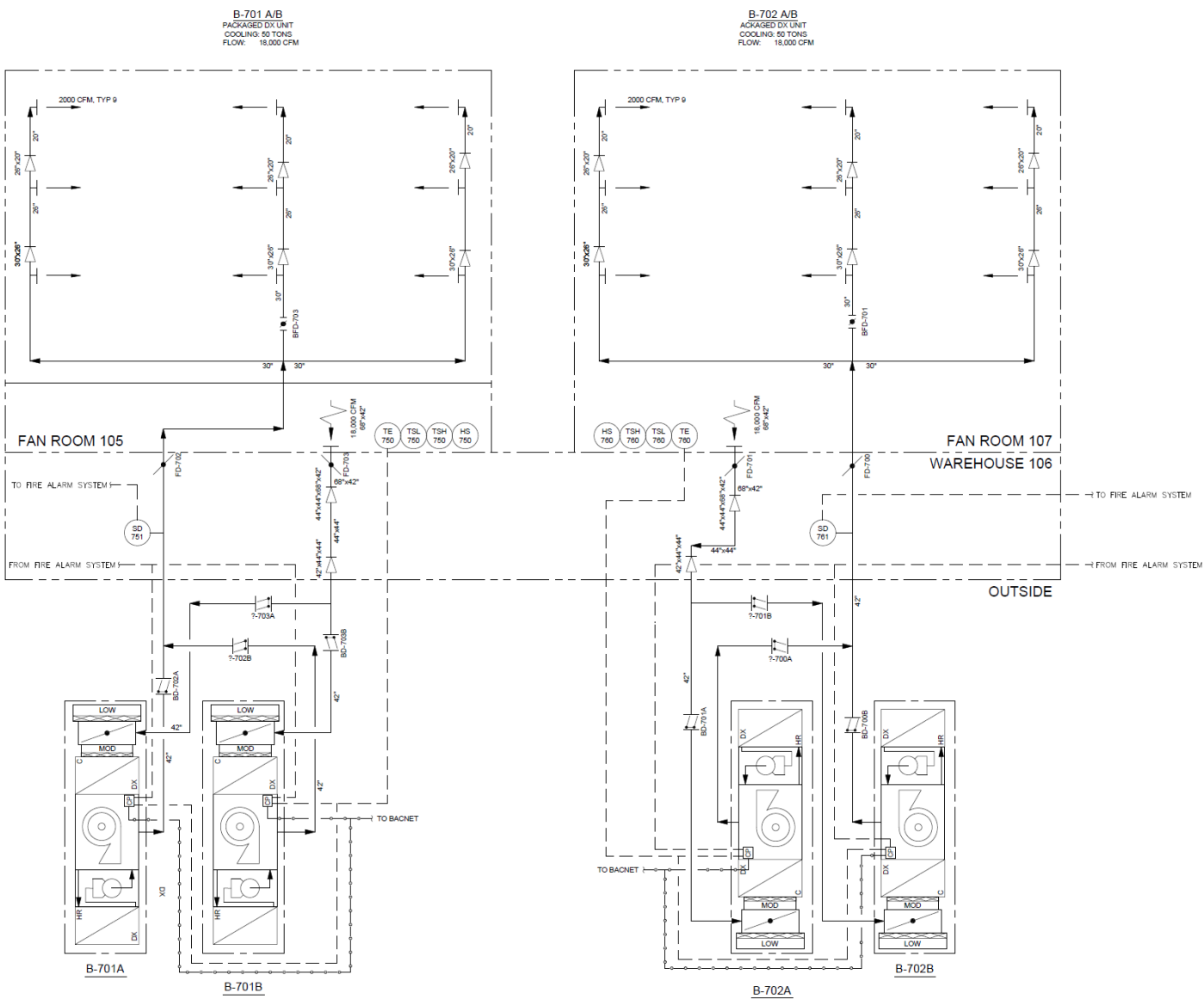
Figure 2.7-5. New Filter Building Heating, Ventilation, and Air Conditioning Flow Diagram (Sheet 1 of 4)
