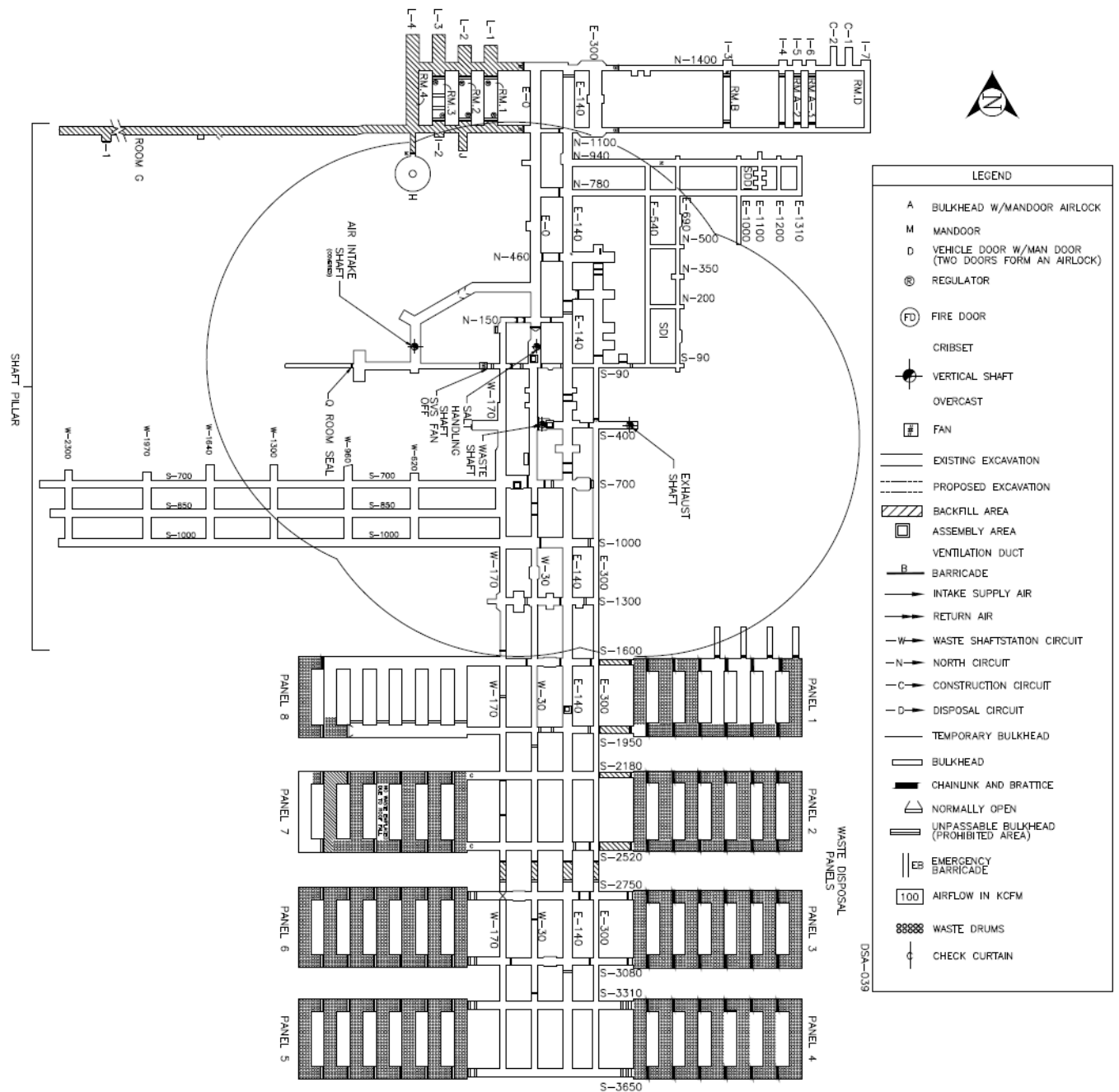
Figure 2.4-15a. Shaft Pillar
