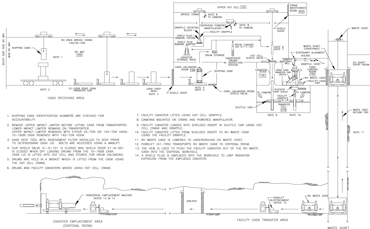
Figure 2.5-3. 10-160B Remote-Handled Waste Handling Process
