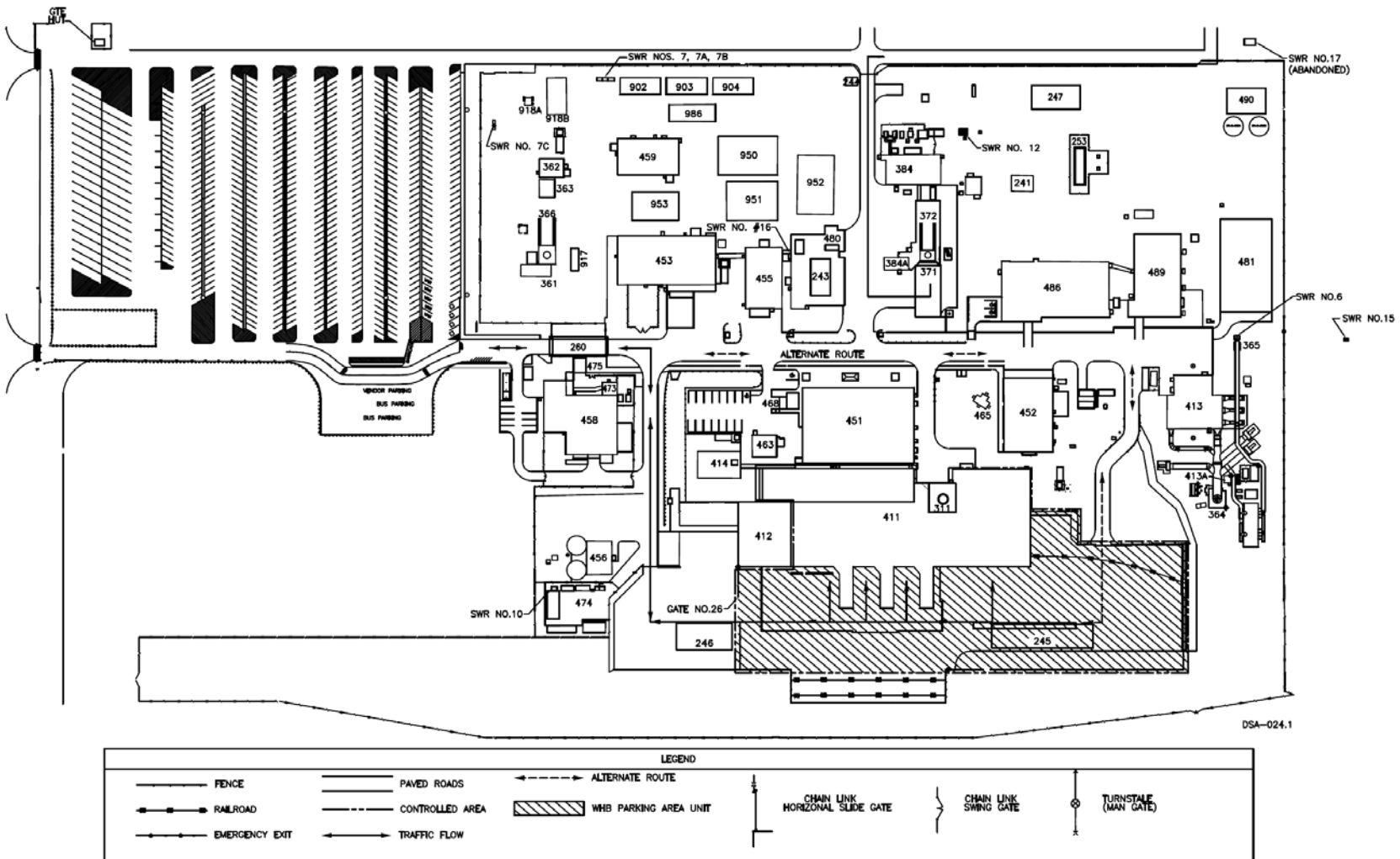
Figure 2.4-1. WIPP Surface Structures (Sheet 1 of 3)
