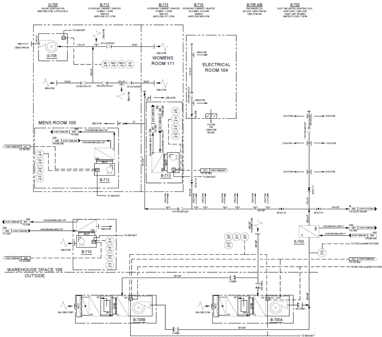
Figure 2.7-5. New Filter Building Heating, Ventilation, and Air Conditioning Flow Diagram (Sheet 2 of 4)
