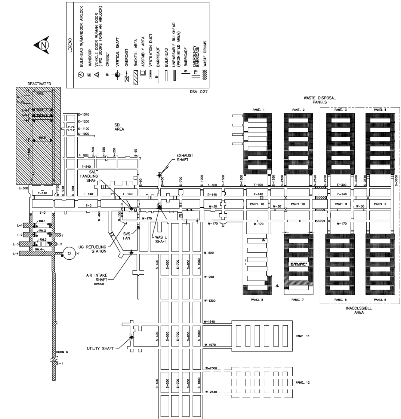
Figure 2.4-2. Underground Facility
