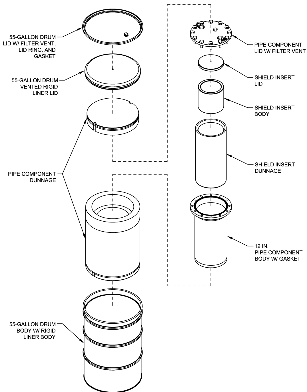
Figure 2.6-13. S200 Pipe Overpack (Pipe Overpack Sheet 2 of 2)
