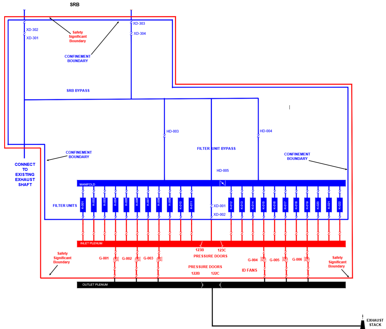
Figure 4.4.5-1. SS Confinement Boundary and SS Pressure Boundary
