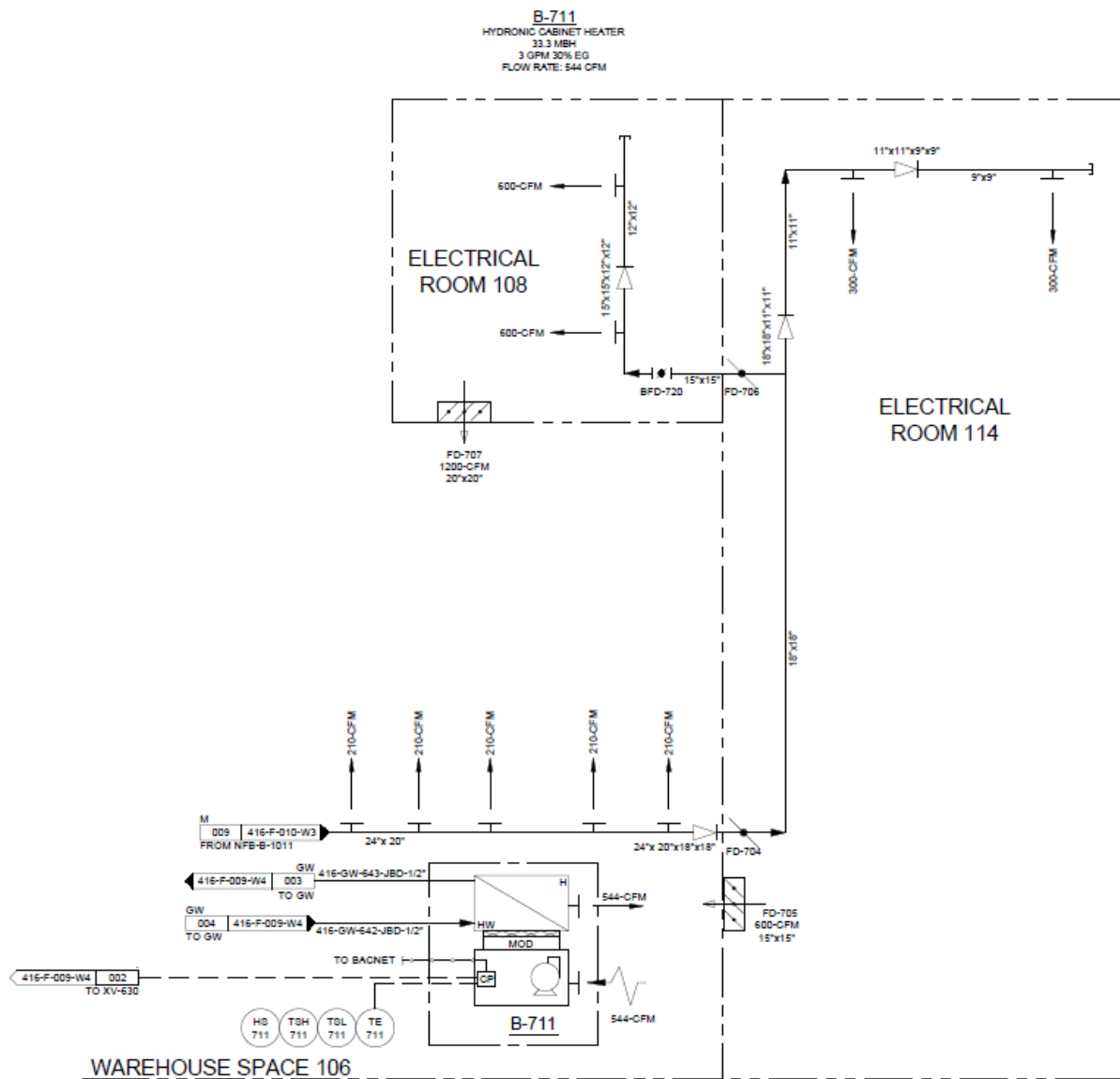
Figure 2.7-5. New Filter Building Heating, Ventilation, and Air Conditioning Flow Diagram (Sheet 3 of 4)
