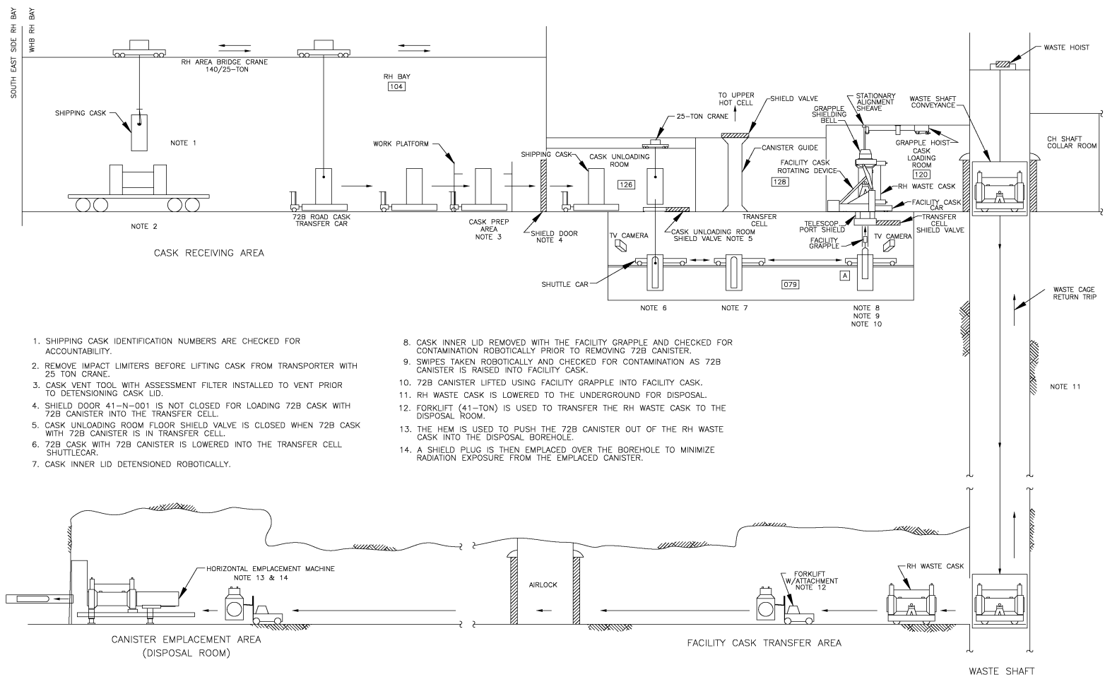
Figure 2.5-2. Remote-Handled Transuranic 72-B Remote-Handled Waste Handling Process
