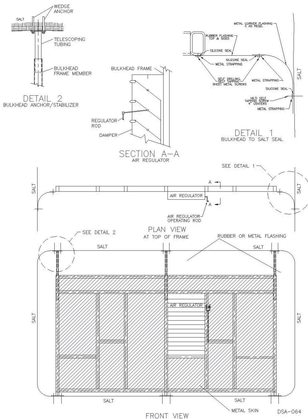
Figure 2.7-7. Typical Bulkhead Design and Components
