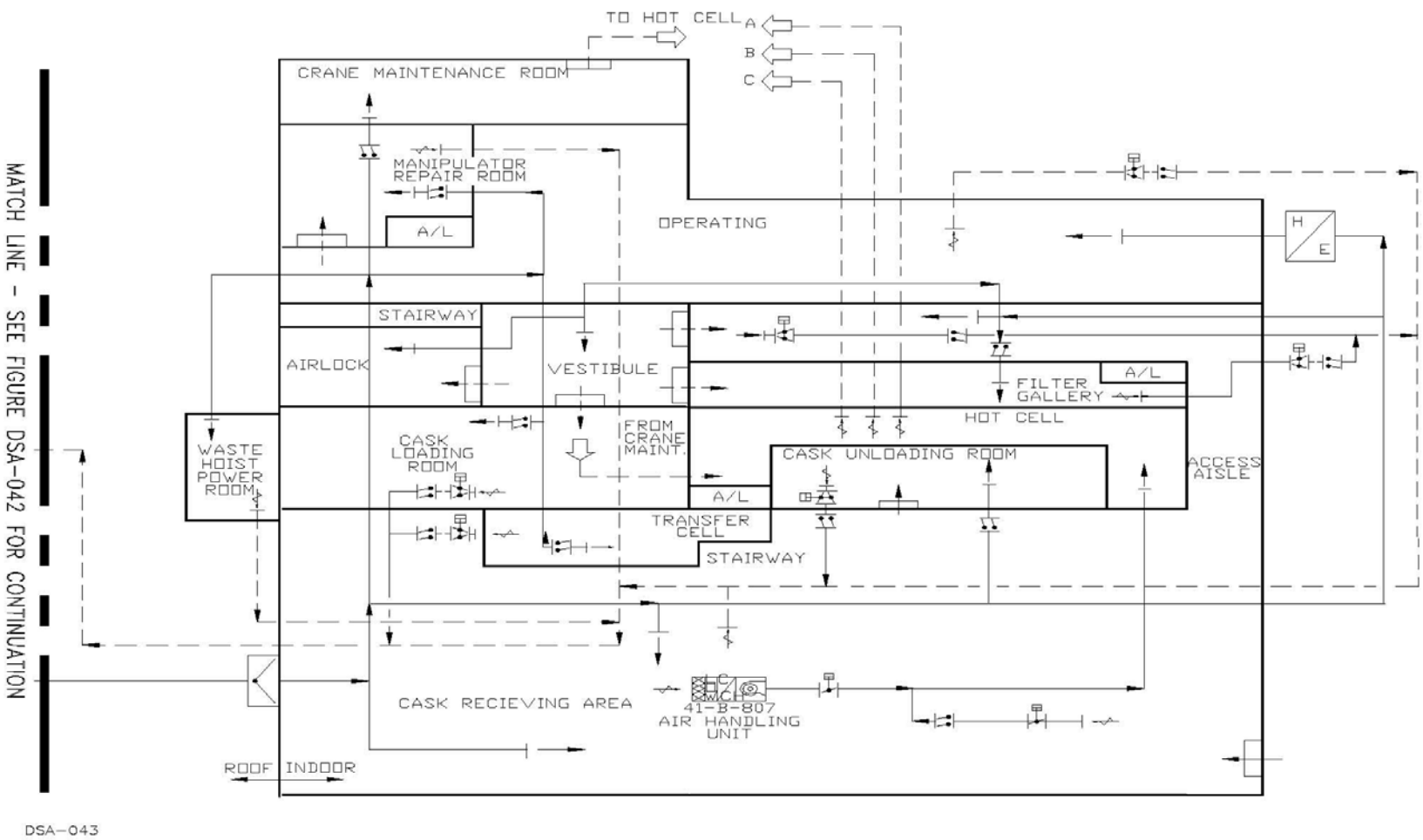
Figure 2.7-3. Waste Handling Building Remote-Handled HVAC Flow Diagram (Sheet 2 of 2)
