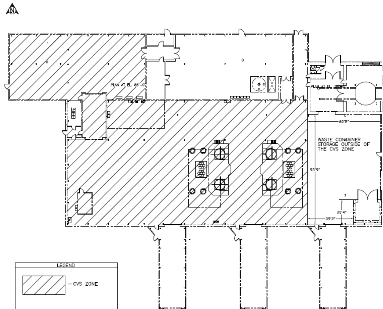
Figure 5.5.3-1. CH Bay Diagram Depicting the CVS Zone
