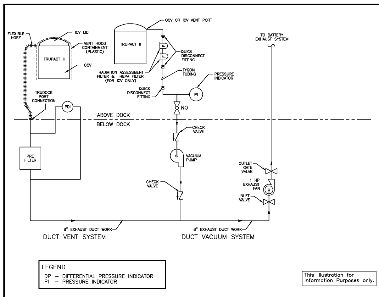
Figure 2.6-18. TRUDOCK Vent Hood System
