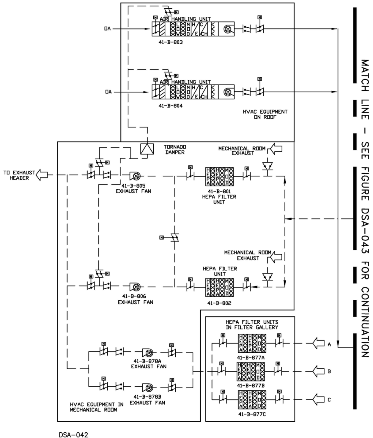
Figure 2.7-3. Waste Handling Building Remote-Handled HVAC Flow Diagram (Sheet 1 of 2)
