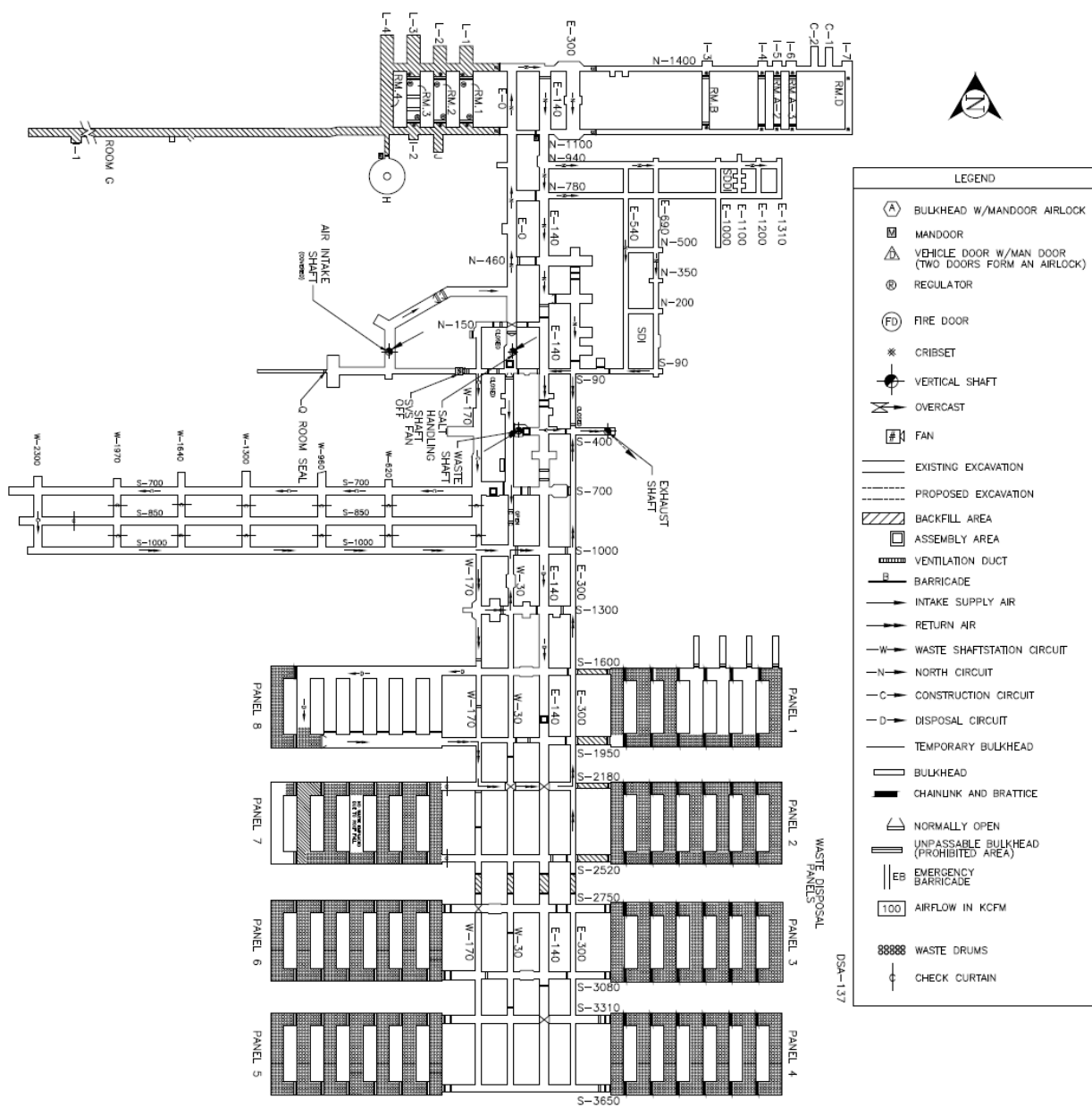
Figure 2.4-15c. Underground Layout and Ventilation Flow: IVS/UVS without SVS Operating
