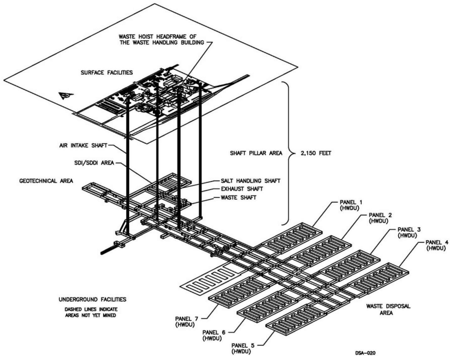
Figure 2.4-3. Spatial View of the WIPP Underground Facility
