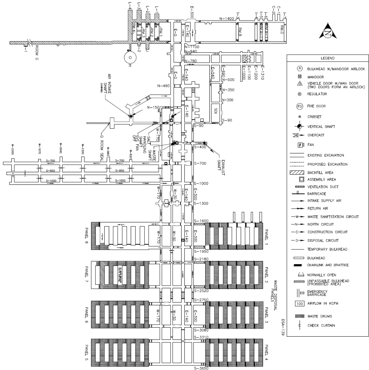
Figure 2.4-15d. Underground Layout and Ventilation Flow: Unfiltered Ventilation
