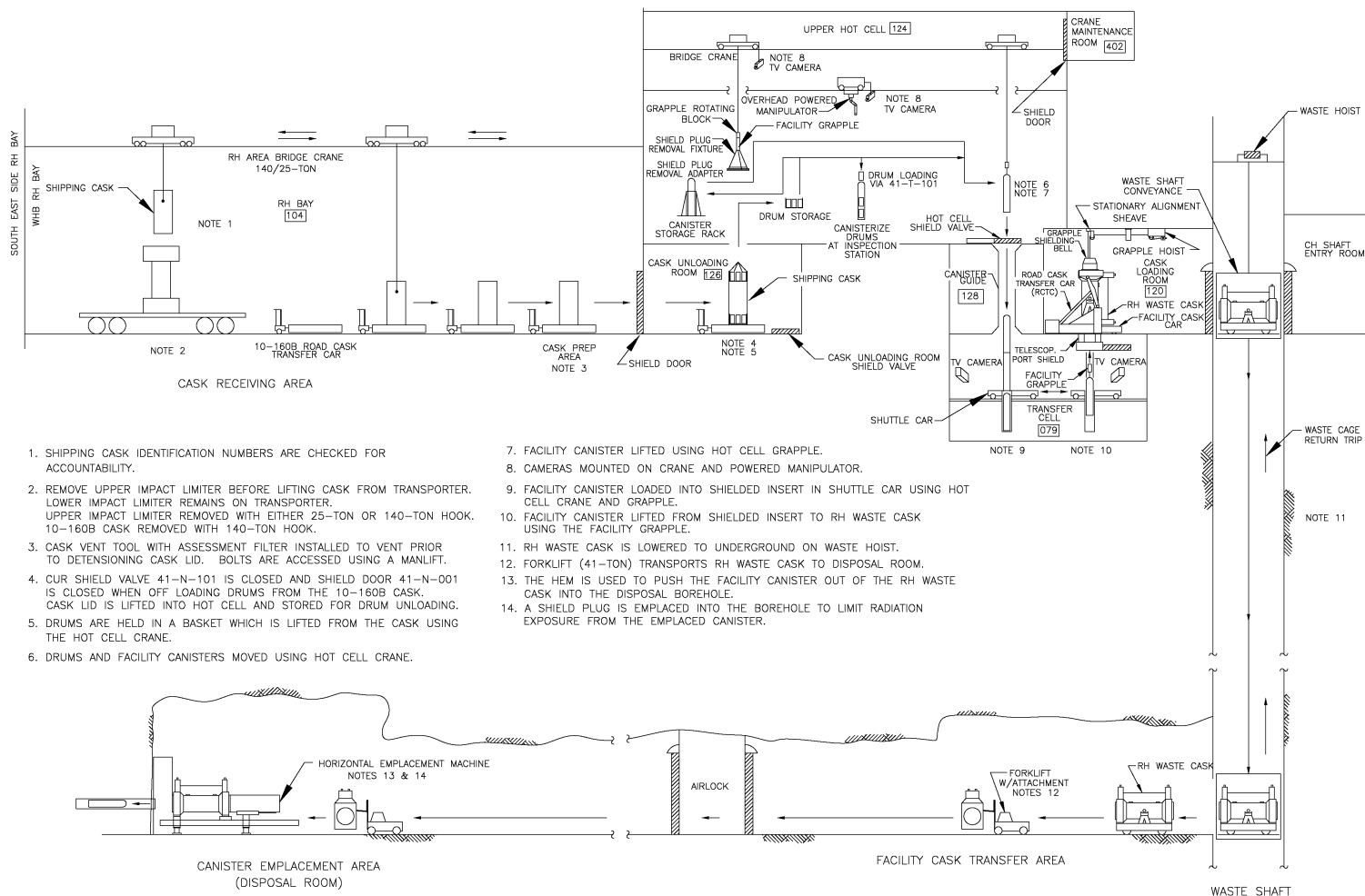
Figure 2.5-3. 10-160B Remote-Handled Waste Handling Process
