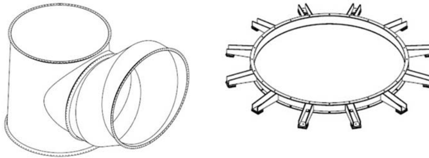
Figure A.2.7.3.9-1 The Wye Assembly and Riser Base Stand
