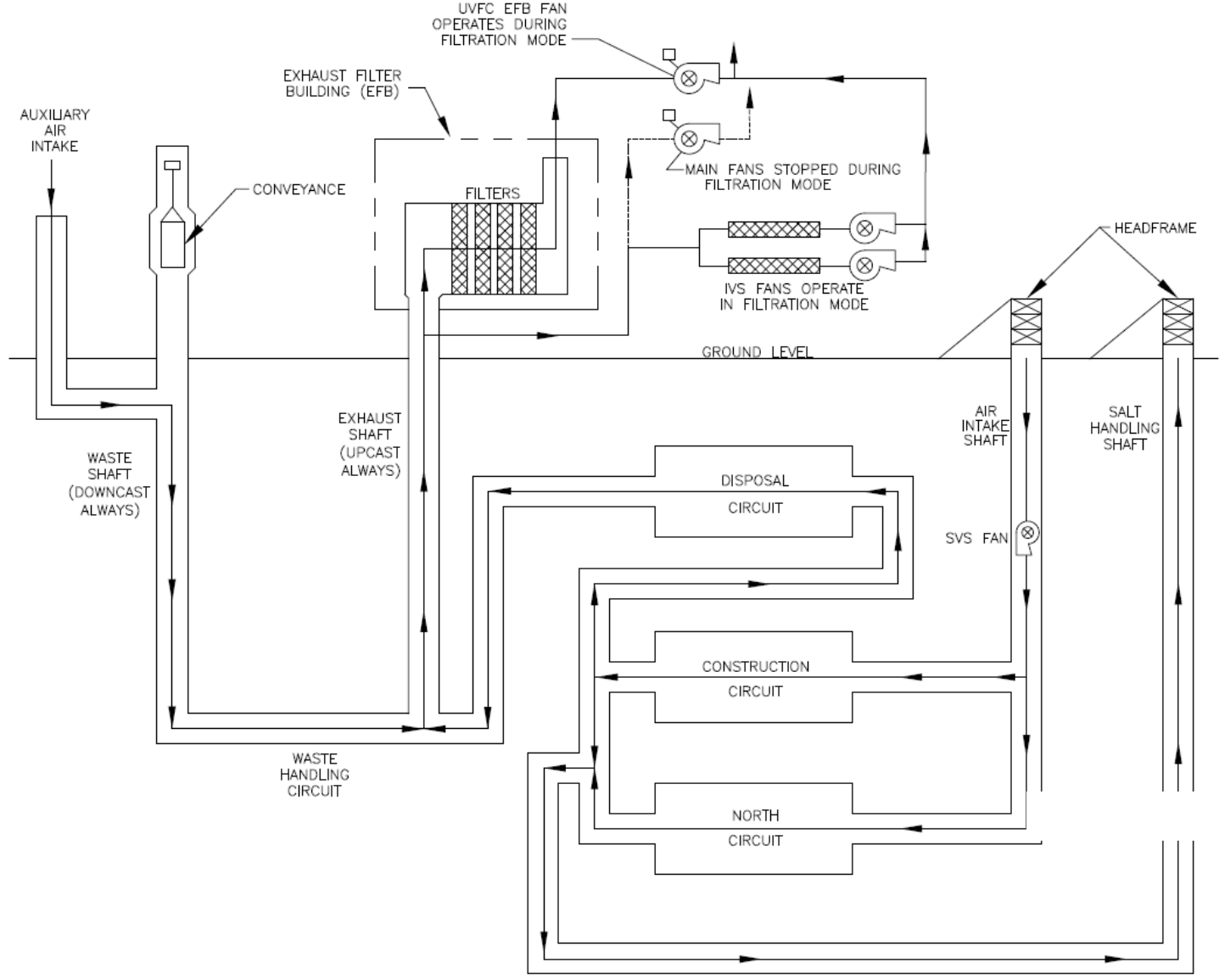
Figure 2.7-7. Underground Ventilation Airflow Diagram with SVS
