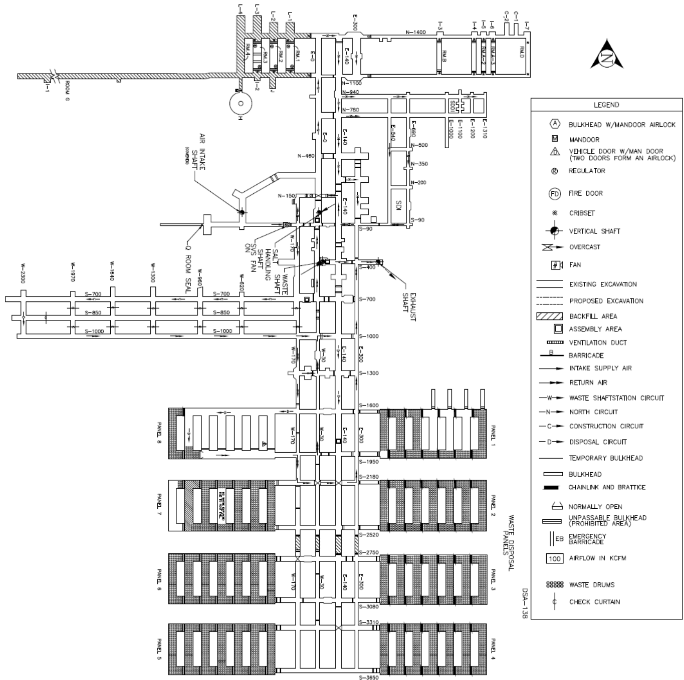
Figure 2.4-15b. Underground Layout and Ventilation Flow IVS/UVS with SVS Operating
