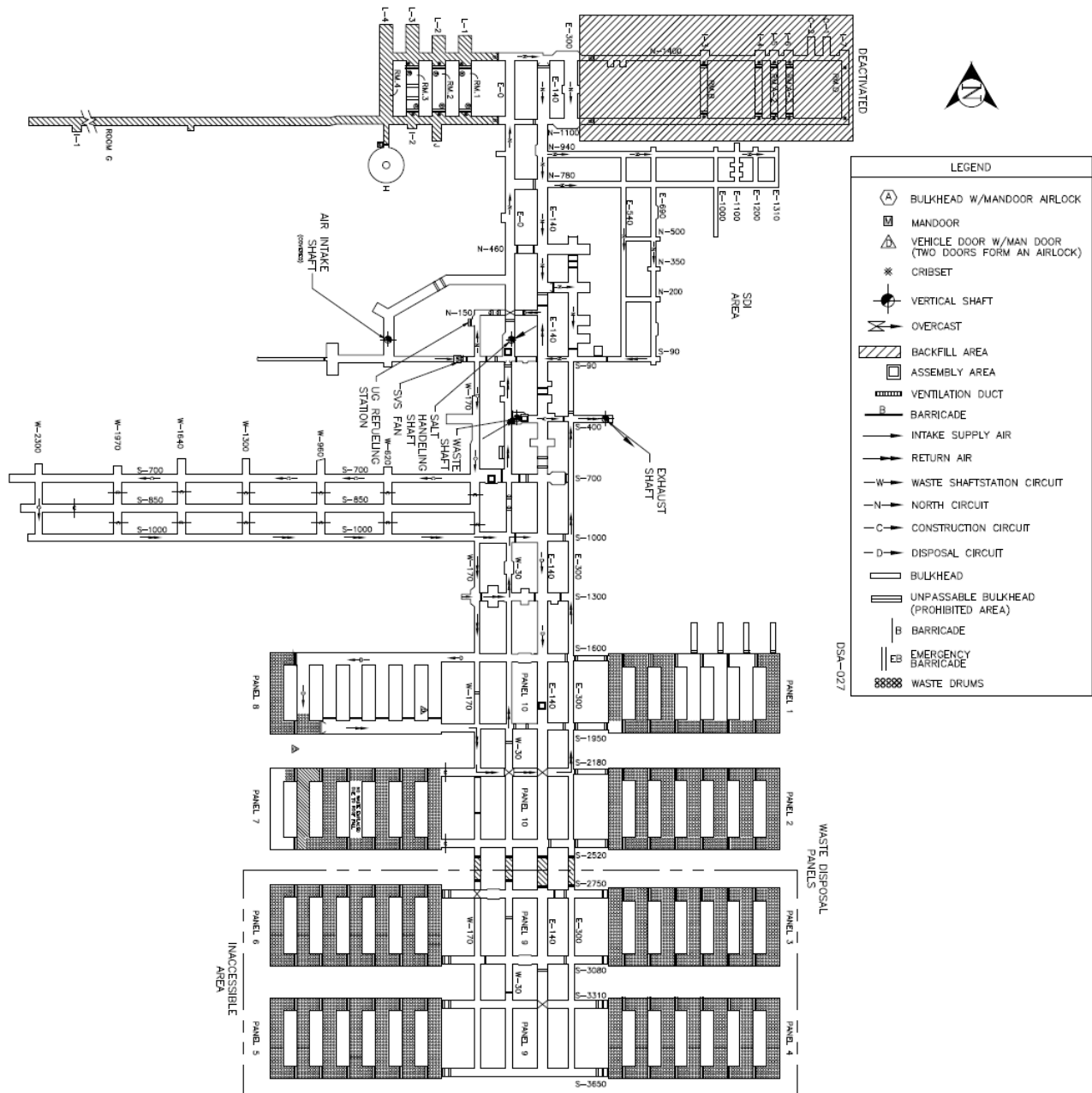
Figure 2.4-2. Underground Facility
