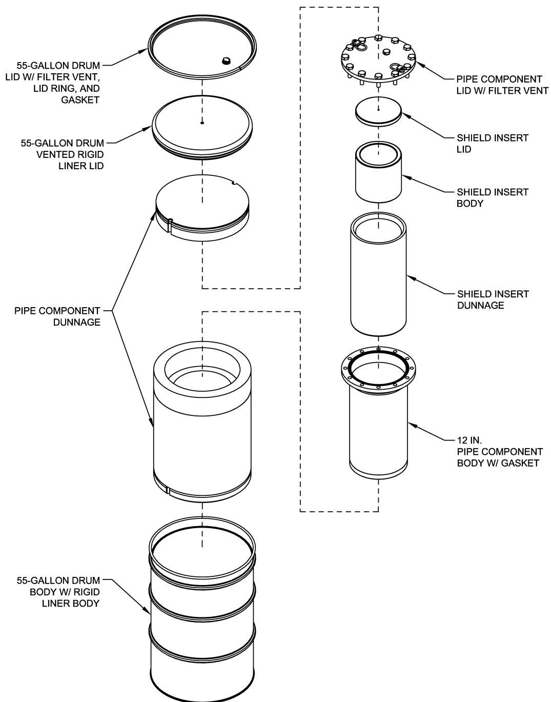
Figure 2.6-13b. S200 Pipe Overpack
