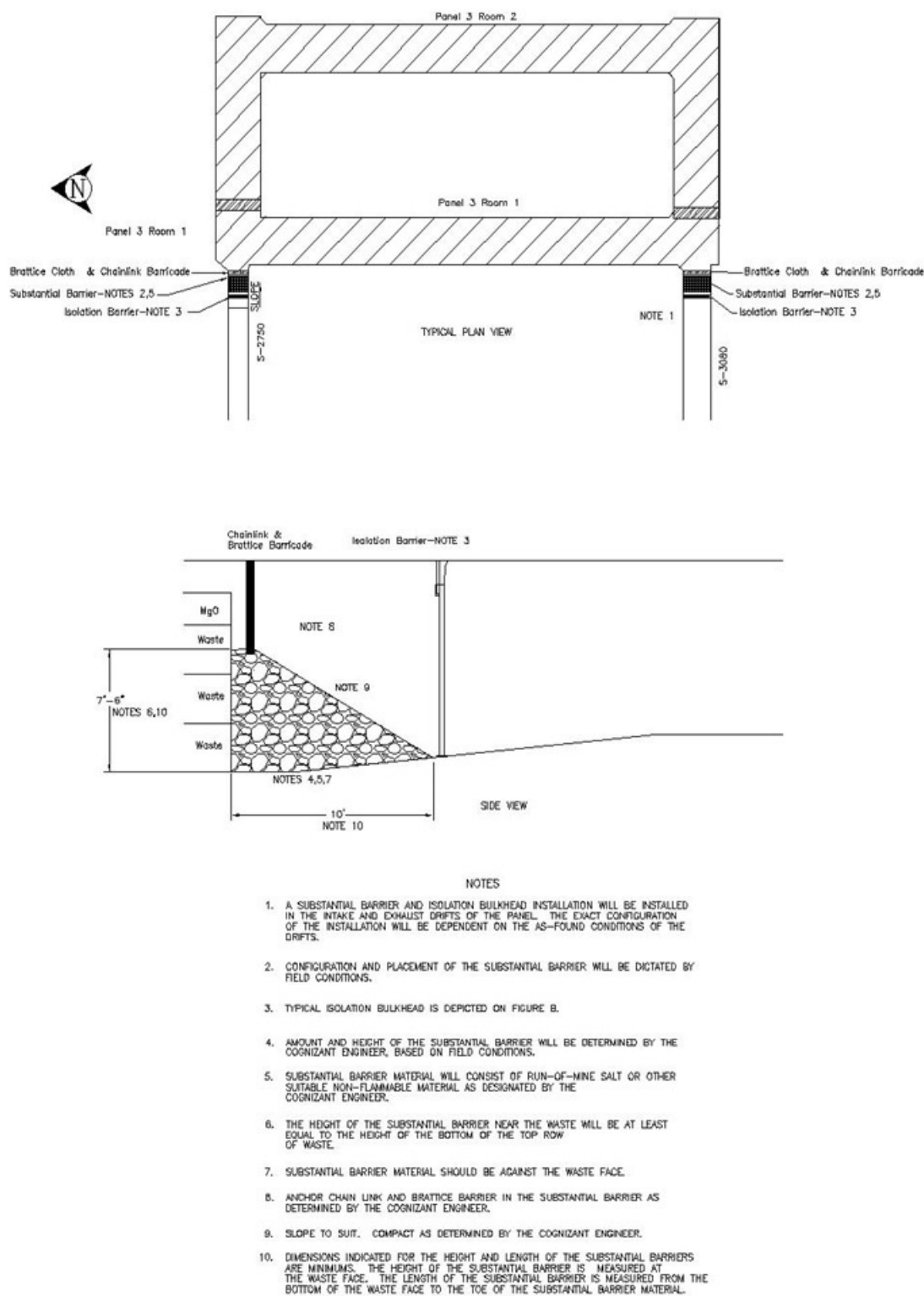
Figure 2.4-18. Substantial Barrier and Isolation Bulkhead
