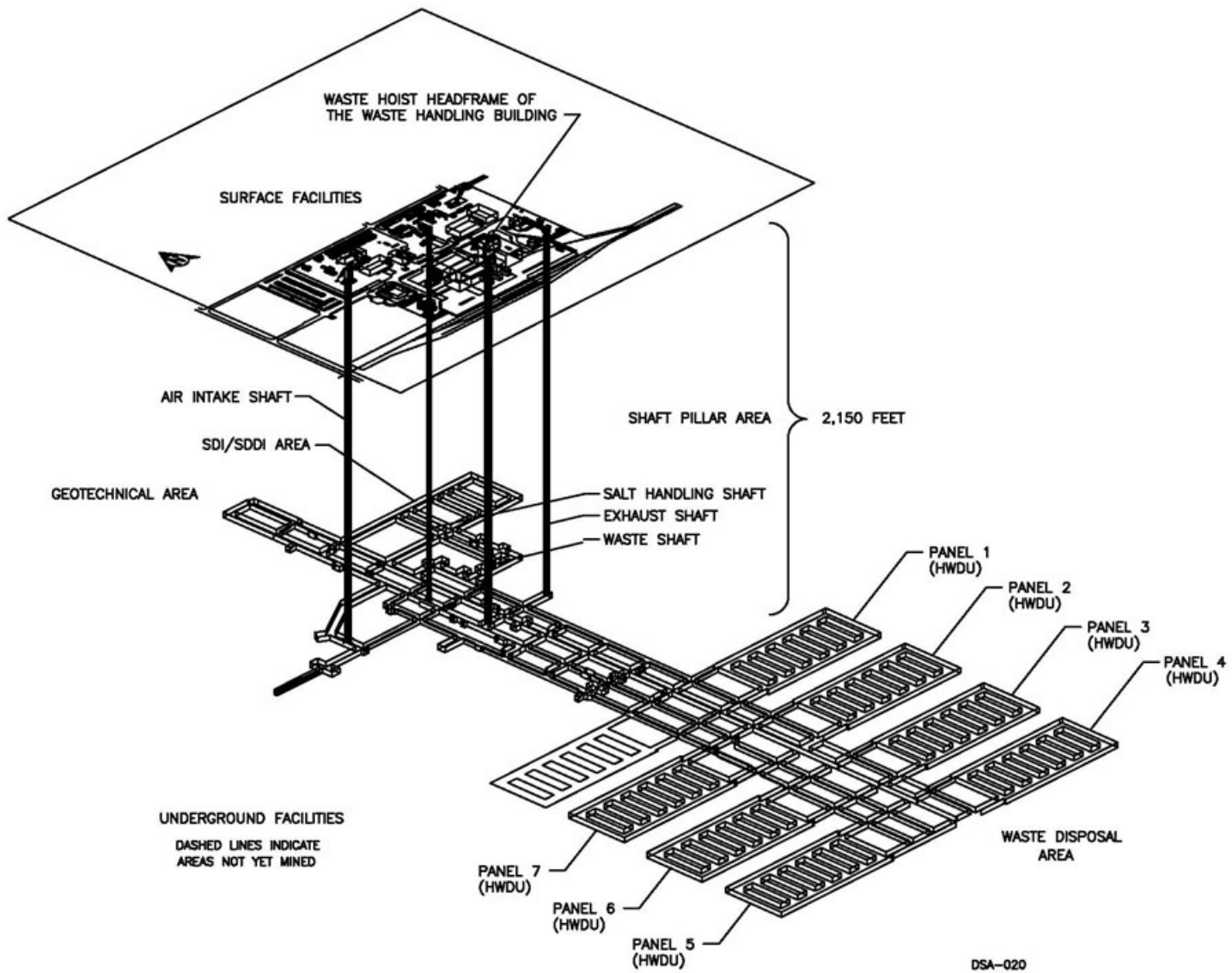
Figure 2.4-3. Spatial View of the WIPP Underground Facilities
