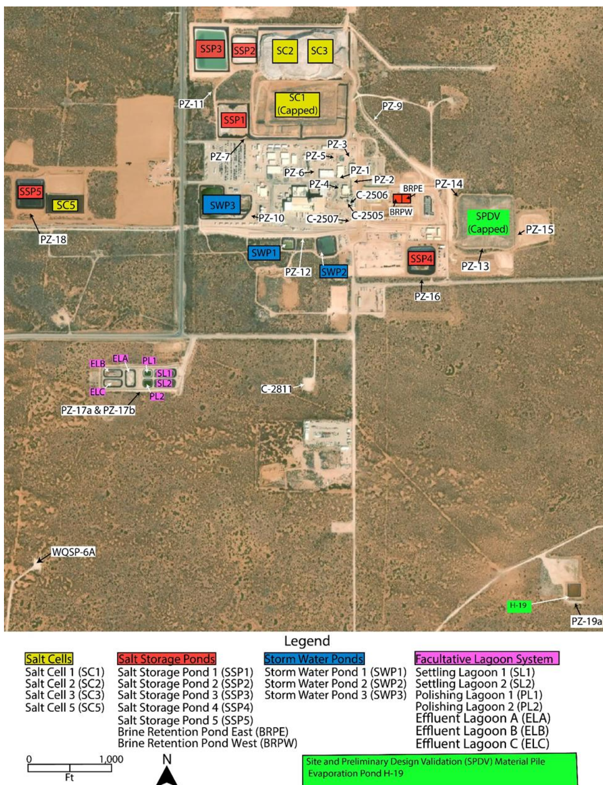
Figure 5.8 – Monitoring Wells and Surface Impoundment Locations
