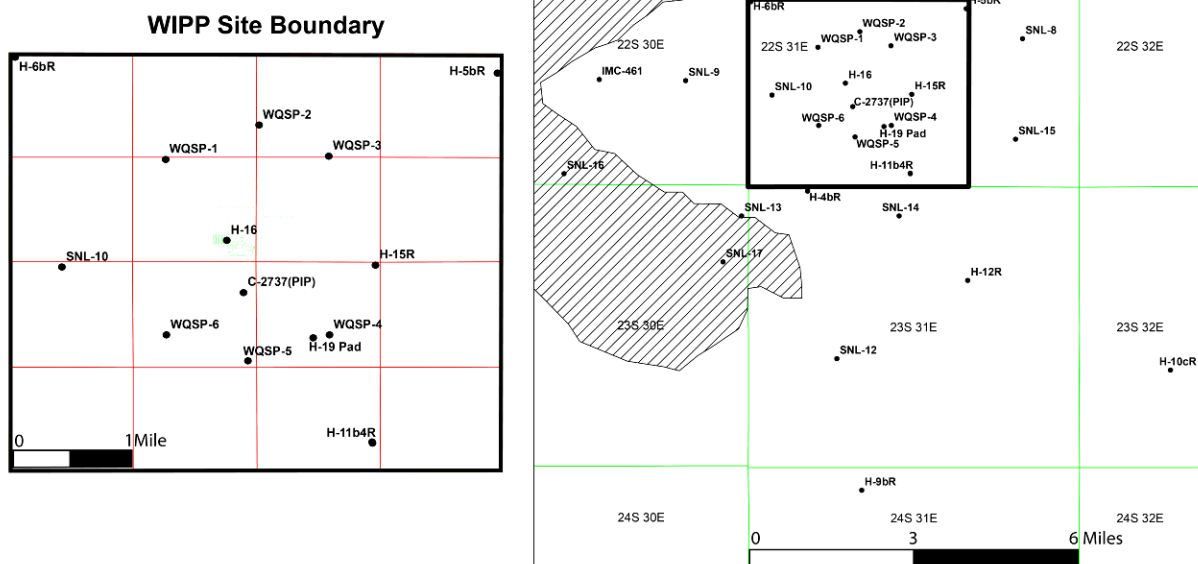
Figure 5.5 – Groundwater Level Surveillance Wells
