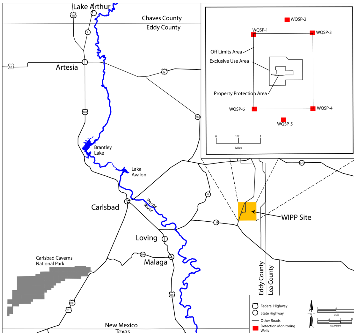
Figure 5.6 – Detection Monitoring Program Wells
