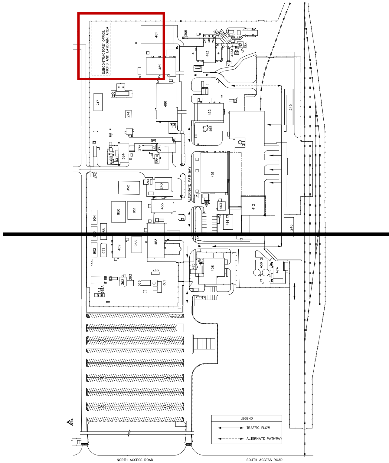
Figure A4-2 WIPP Traffic Flow Diagram
