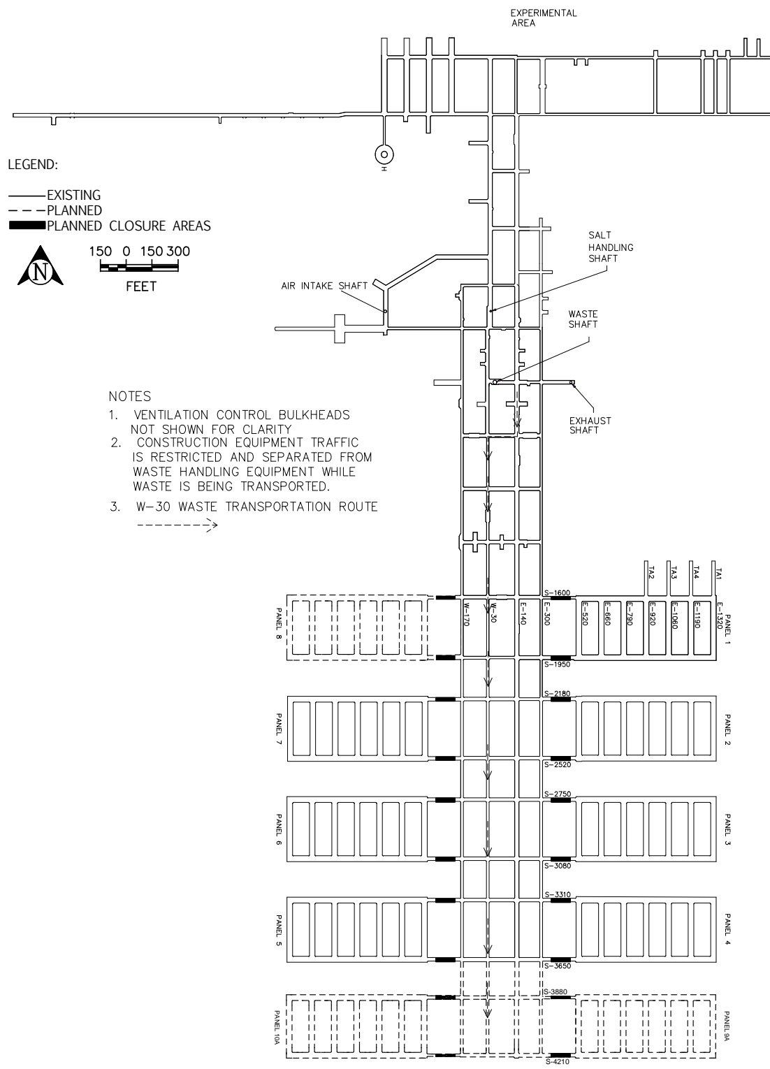
Figure A4-4a Typical Underground Transport Route Using W-30
