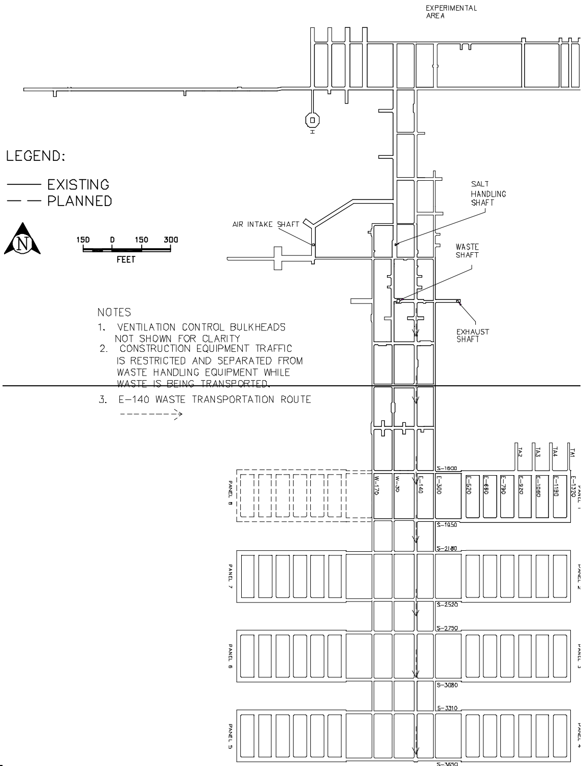
Figure A4-4 Typical Underground Transport Route Using E-140
