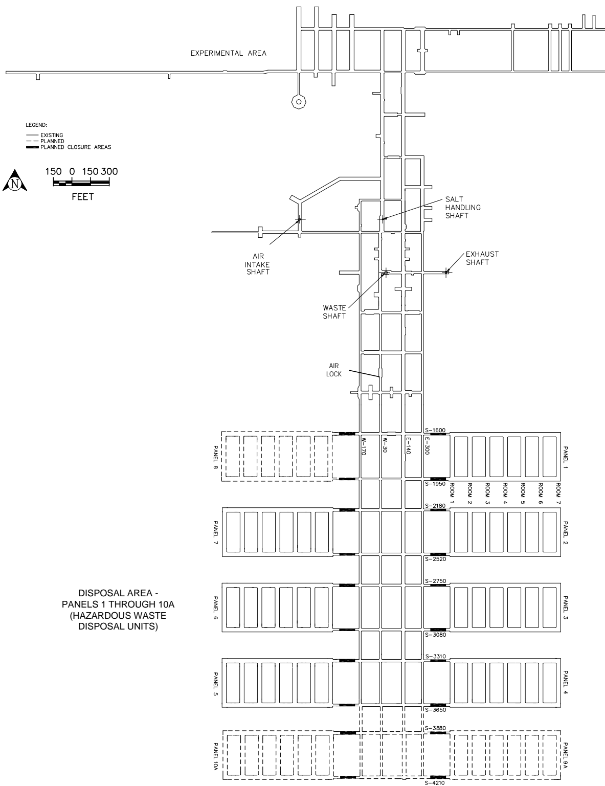
Figure D-3 WIPP Underground Facilities
