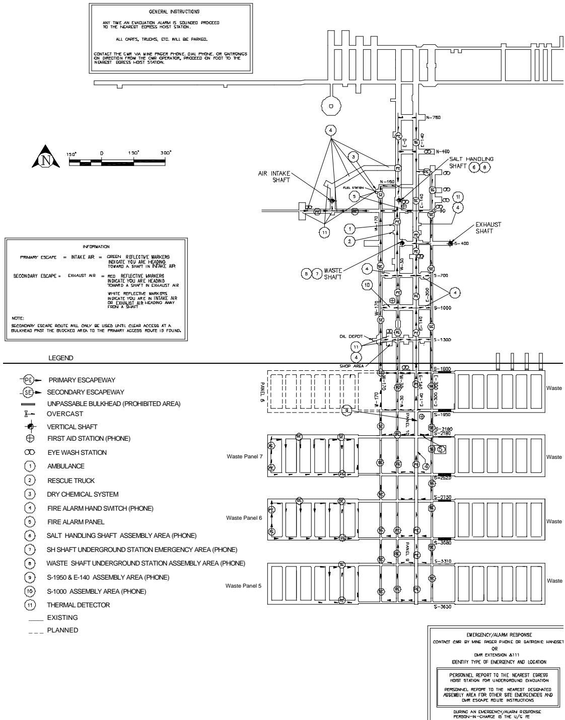
Figure D-5 Underground Emergency Equipment Locations and Underground Evacuation Routes
