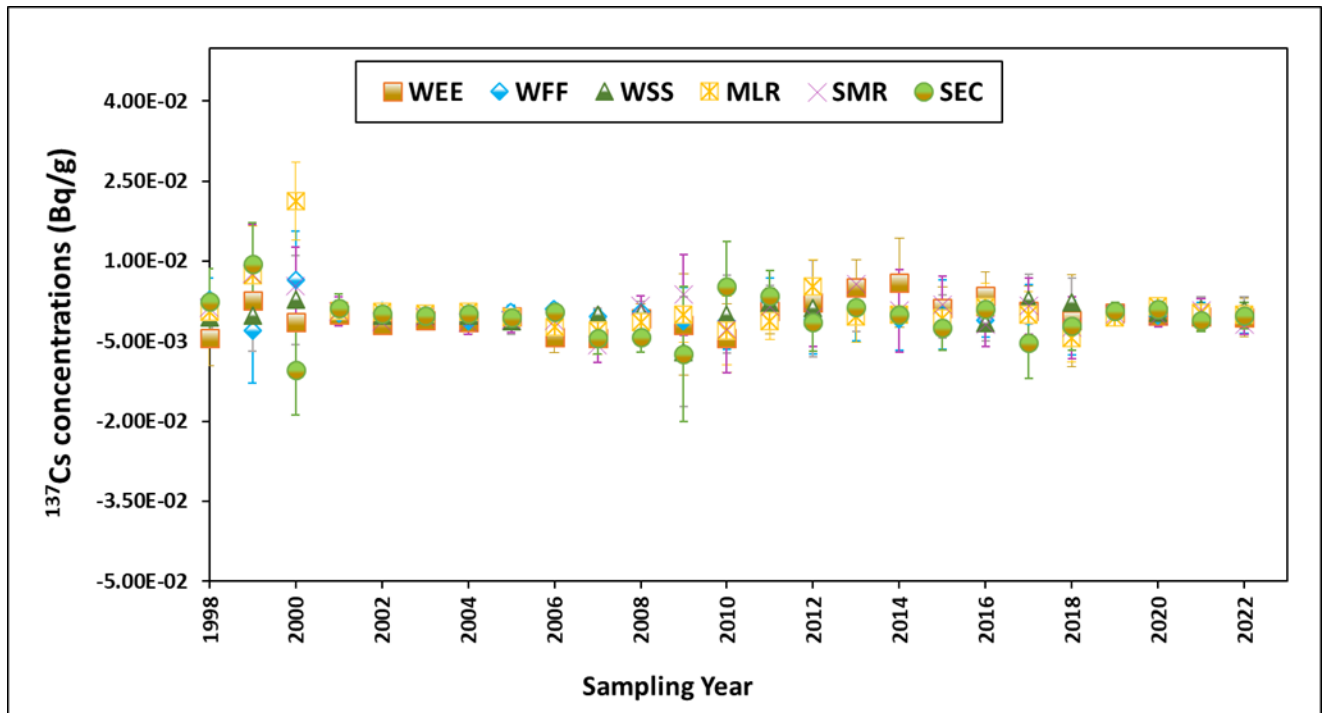
Figure 4.15 – Historical Concentrations of ^{137}\text{Cs} in Vegetation Samples Collected from Six Sampling Locations
