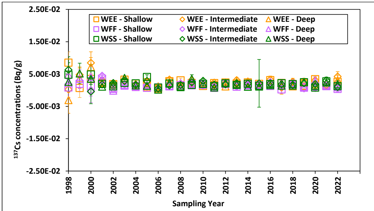
Figure 4.12a – ^{137}\text{Cs} Concentrations in Soil Samples Collected from WIPP Site
