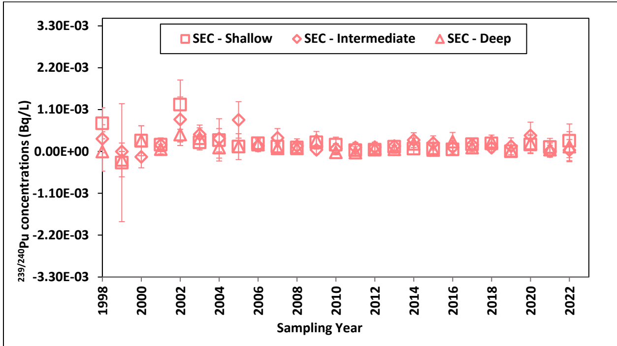
Figure 4.10c – ^{239/240}\text{Pu} Concentrations in Soil Samples Collected from Outer Sites
