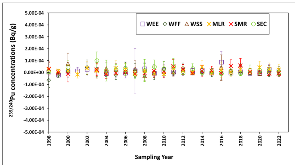
Figure 4.13 – Historical Concentrations of ^{239/240}\text{Pu} in Vegetation Samples Collected from Six Sampling Locations
