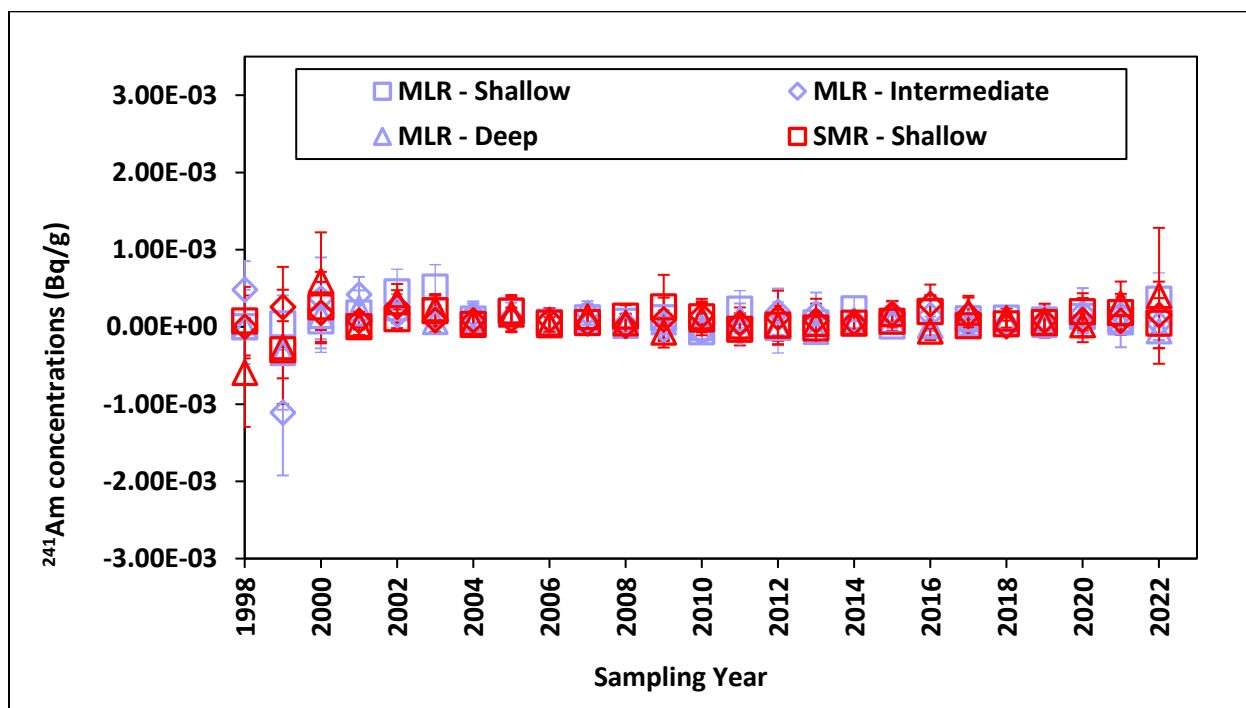
Figure 4.11b – ^{241}\text{Am} Concentrations in Soil Samples Collected from 5-mi Ring
