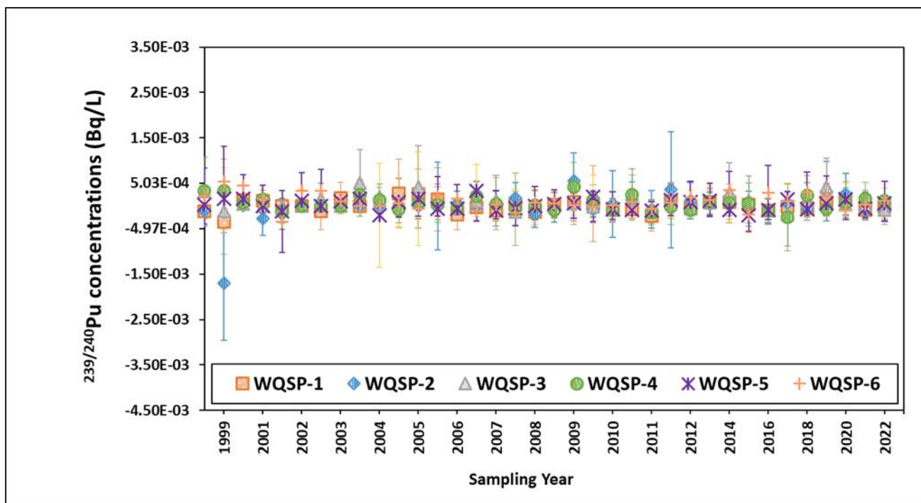
Figure 4.4a – Historical Concentrations of ^{239/240}\text{Pu} at Six DMP Wells
