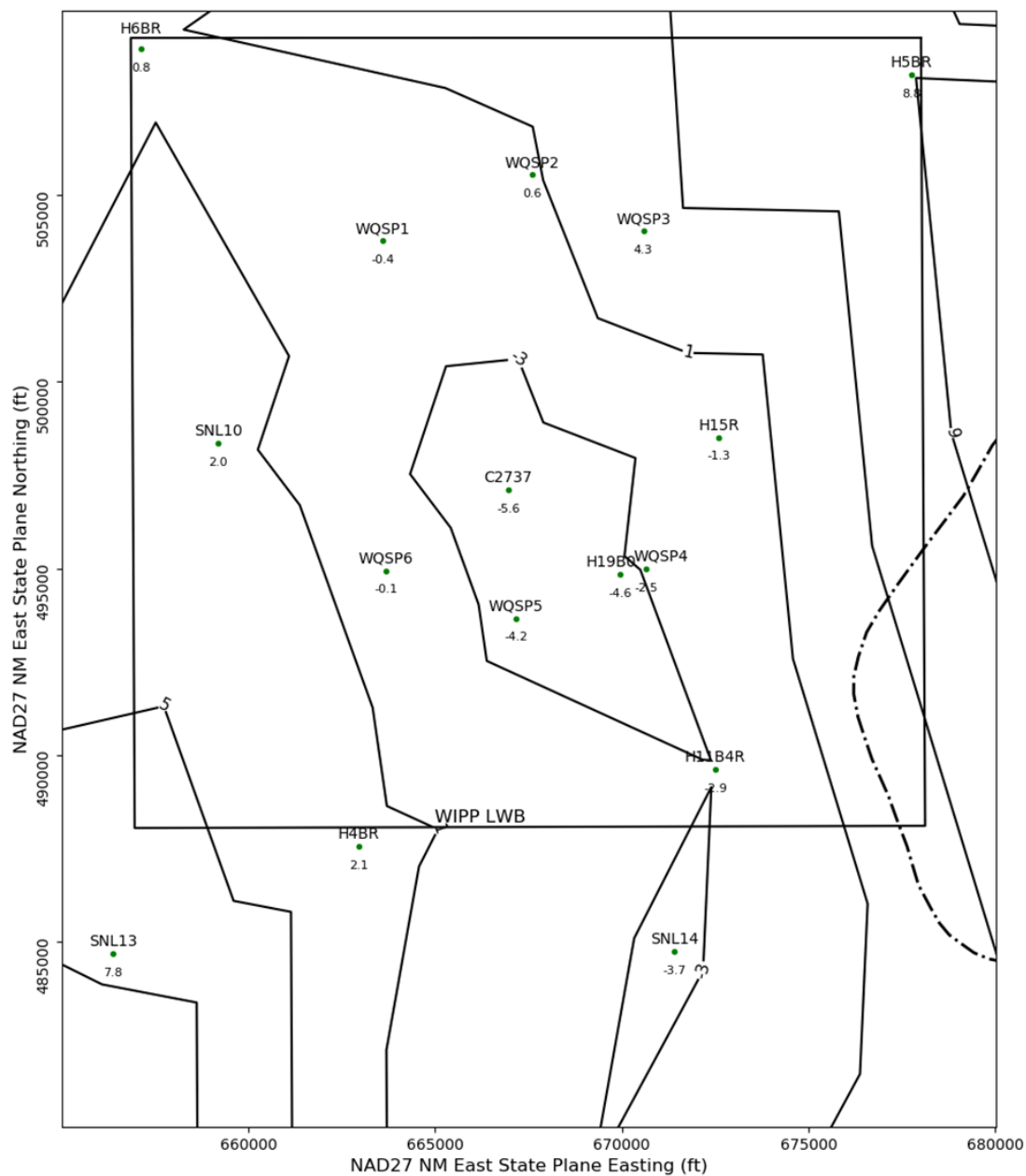
Figure 6.5 – Triangulated Contours (in 5-ft intervals) for Measured Minus Modeled Culebra Freshwater Head
