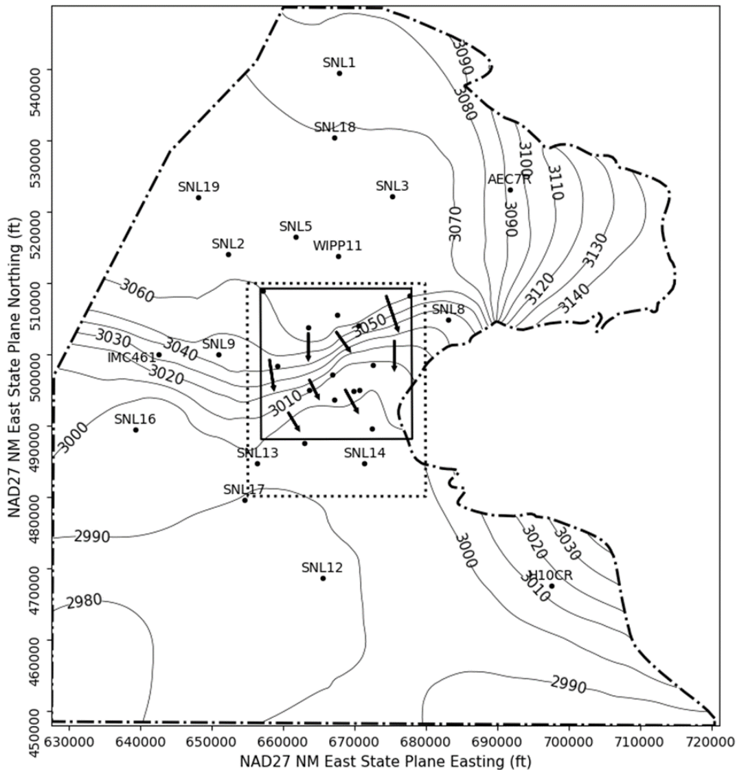
Figure 6.3 – Model-Generated 2022 Culebra Freshwater Head Contours in the Model Domain (Contour interval 10 feet, contour in feet above mean sea level). The dotted rectangle corresponds to the region contoured in Figure 6.4. The black square corresponds to the WIPP LWB. Wells inside the WIPP LWB are not labeled; refer to Figure 6.4 for identification of these wells. The black arrows indicate the groundwater flow direction inside the WIPP LWB.
