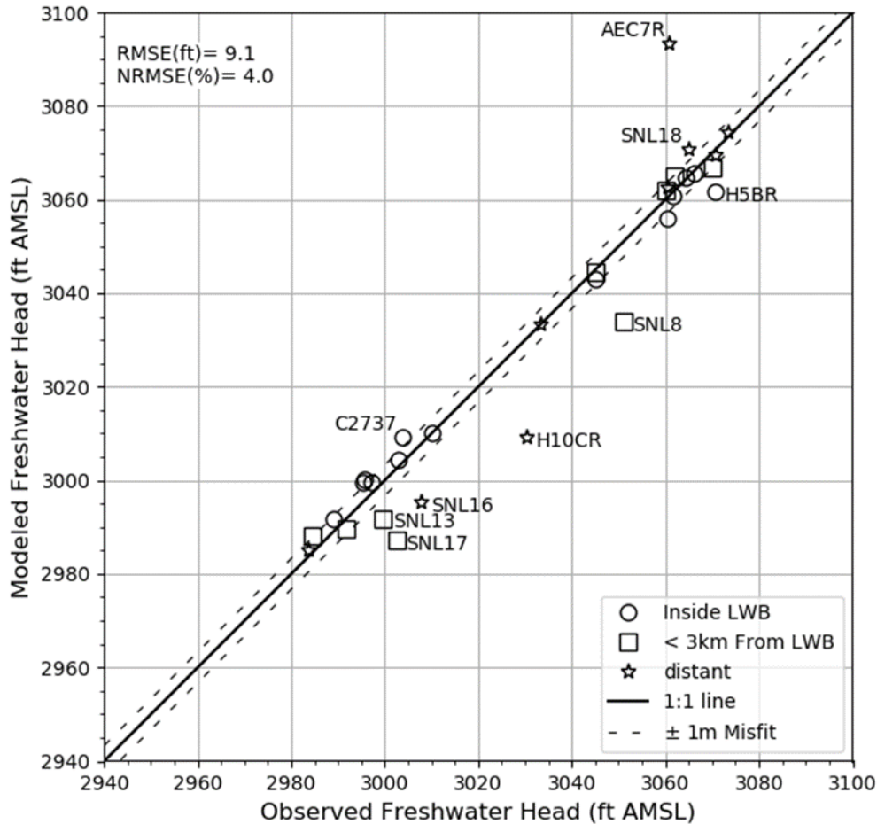
Figure 6.6 – Modeled Versus Measured Scatter Plot for Parameter Estimation Tool-Calibrated MODFLOW 2000 Generated Heads and December 2021 Culebra Freshwater Heads
