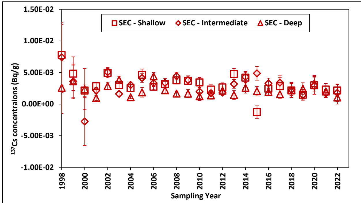
Figure 4.12c – 137 Cs Concentrations in Soil Samples Collected from Outer Sites
