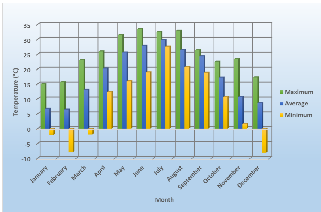
Figure 5.3 – WIPP Site Average Temperatures (°C) for 2022
