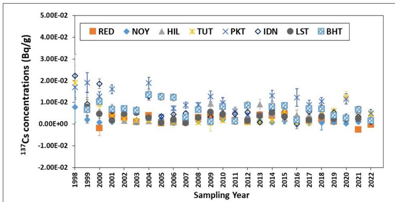
Figure 4.8 – Historical Concentrations of ^{137}\text{Cs} in Sediment Samples at Tanks and Tank-like Structures
