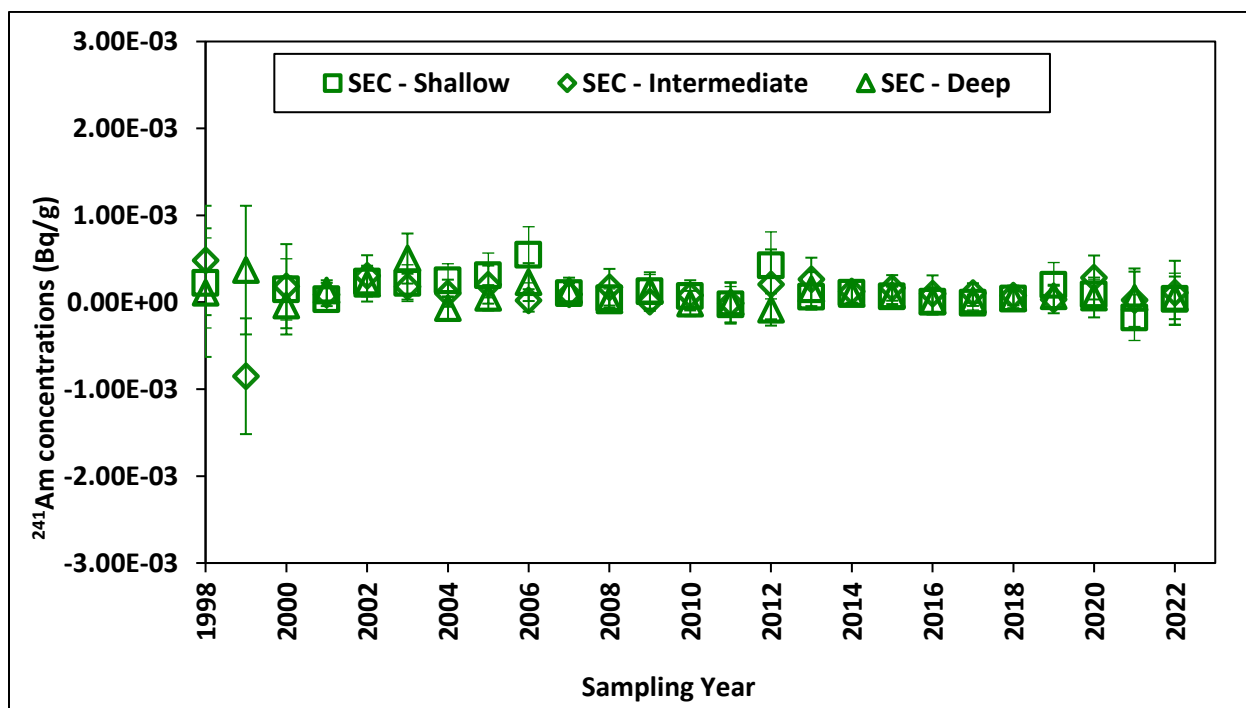
Figure 4.11c – ^{241}\text{Am} Concentrations in Soil Samples Collected from Outer Sites
