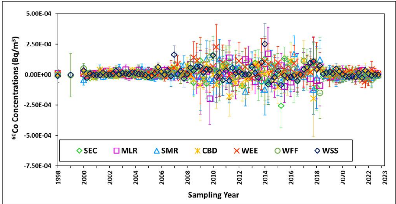
Figure 4.3b – Historical Concentrations of 60 Co at Seven Air Sampling Locations
