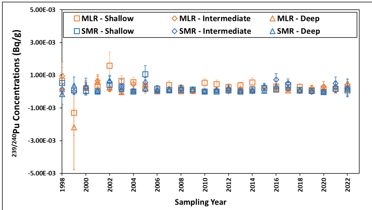
Figure 4.10b – ^{239/240}\text{Pu} Concentrations in Soil Samples Collected from 5-mi Ring
