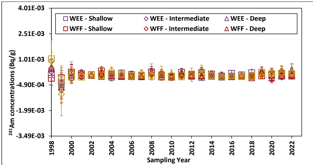
Figure 4.11a – ^{241}\text{Am} Concentrations in Soil Samples Collected from WIPP Site
