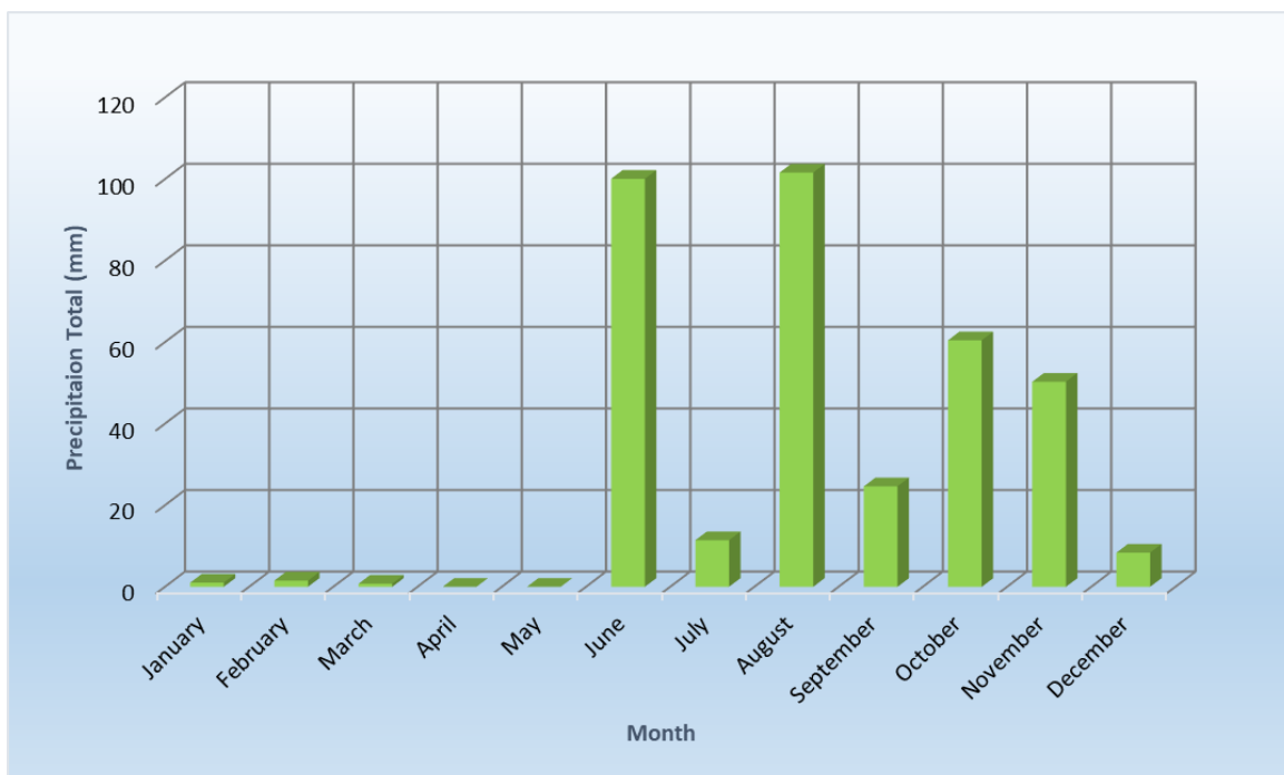
Figure 5.1 – WIPP Site Precipitation Monthly Totals for 2022
