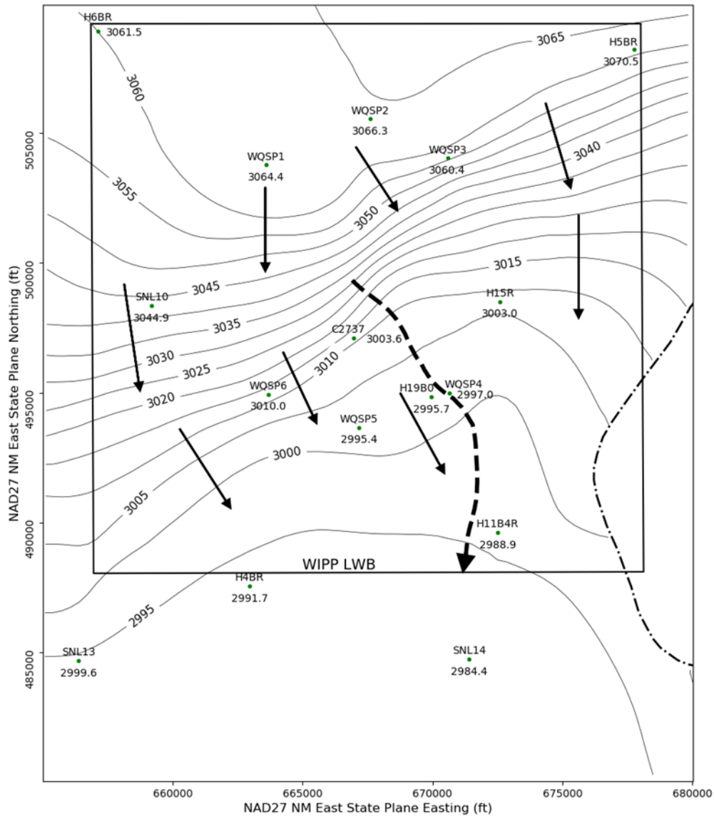
Figure 6.4 – Model-Generated 2022 Culebra Freshwater Head Contours (5-ft Contour Interval) in the WIPP Vicinity with Water Particle Track (Dashed Line with Arrow) from Waste Handling Shaft to WIPP Land Withdrawal Boundary (Contour in feet above mean sea level, black arrows indicate flow direction within LWB).
