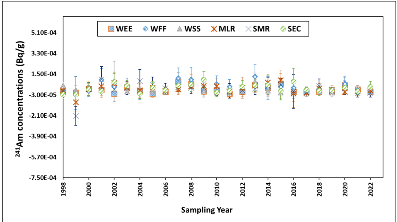
Figure 4.14 – Historical Concentrations of ^{241}\text{Am} in Vegetation Samples Collected from Six Sampling Locations
