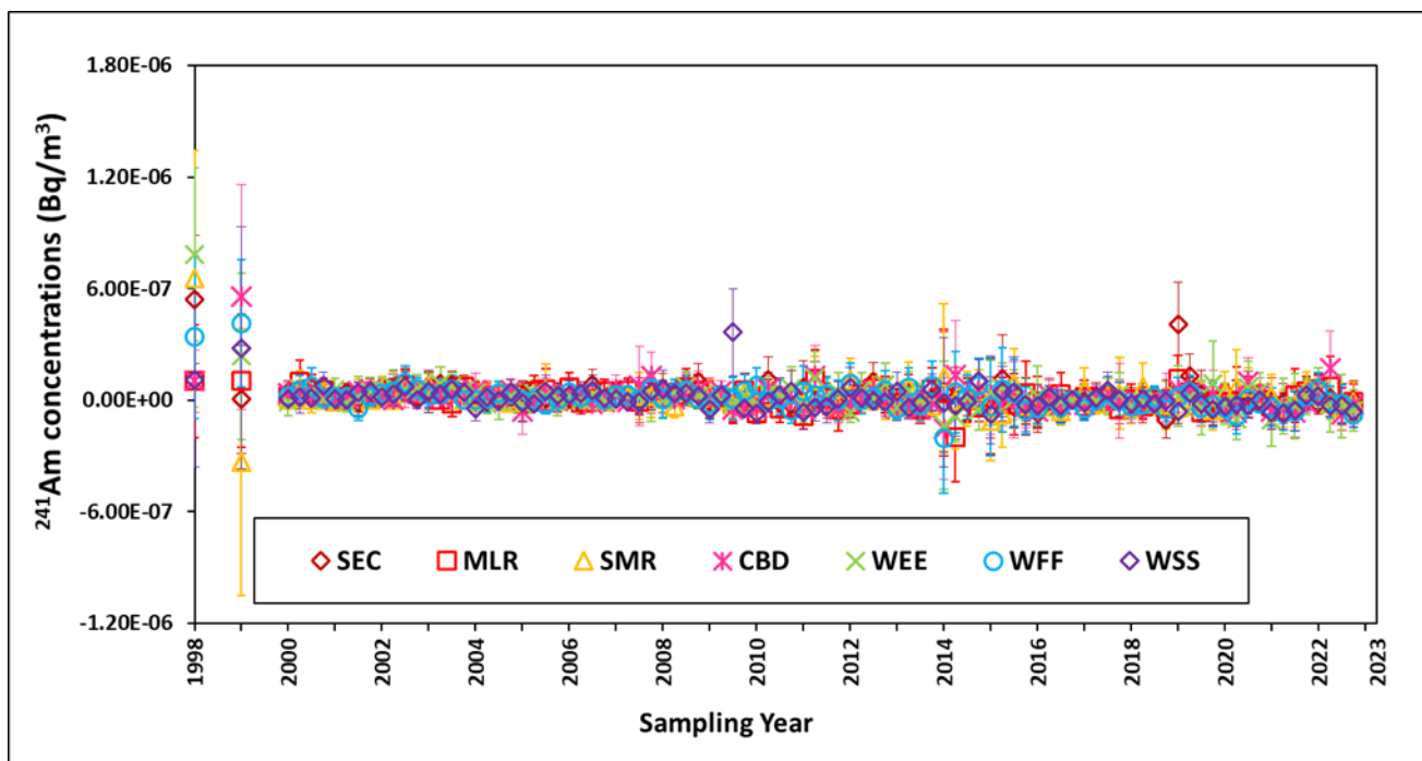
Figure 4.2b – Historical Concentrations of ^{241}\text{Am} at Seven Air Sampling Locations
