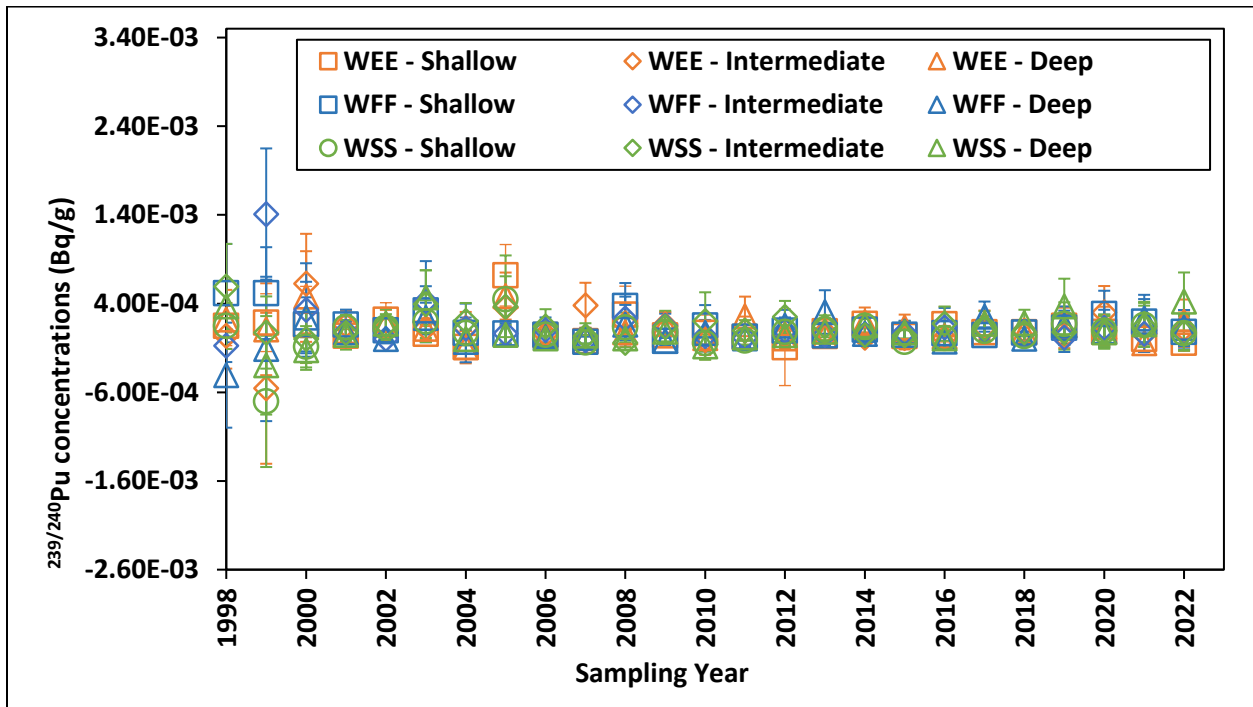
Figure 4.10a – ^{239/240}\text{Pu} Concentrations in Soil Samples Collected from WIPP Site
