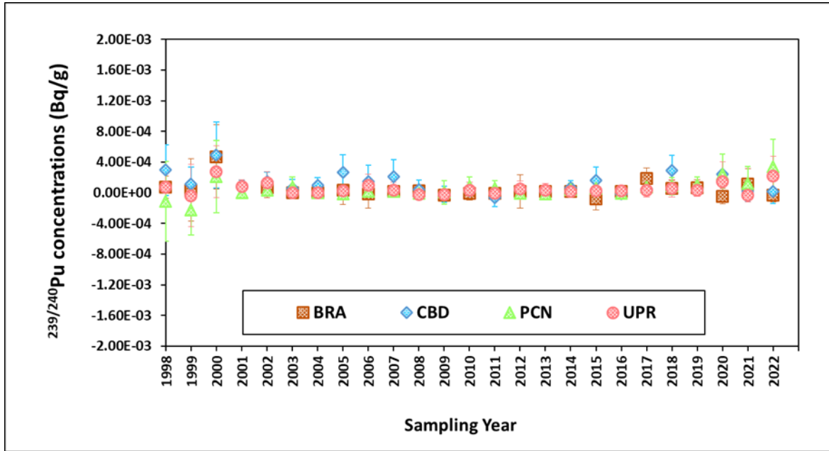
Figure 4.7a – Historical Concentrations of ^{239/240}\text{Pu} in Sediment Samples at Pecos River and Associated Bodies of Water
