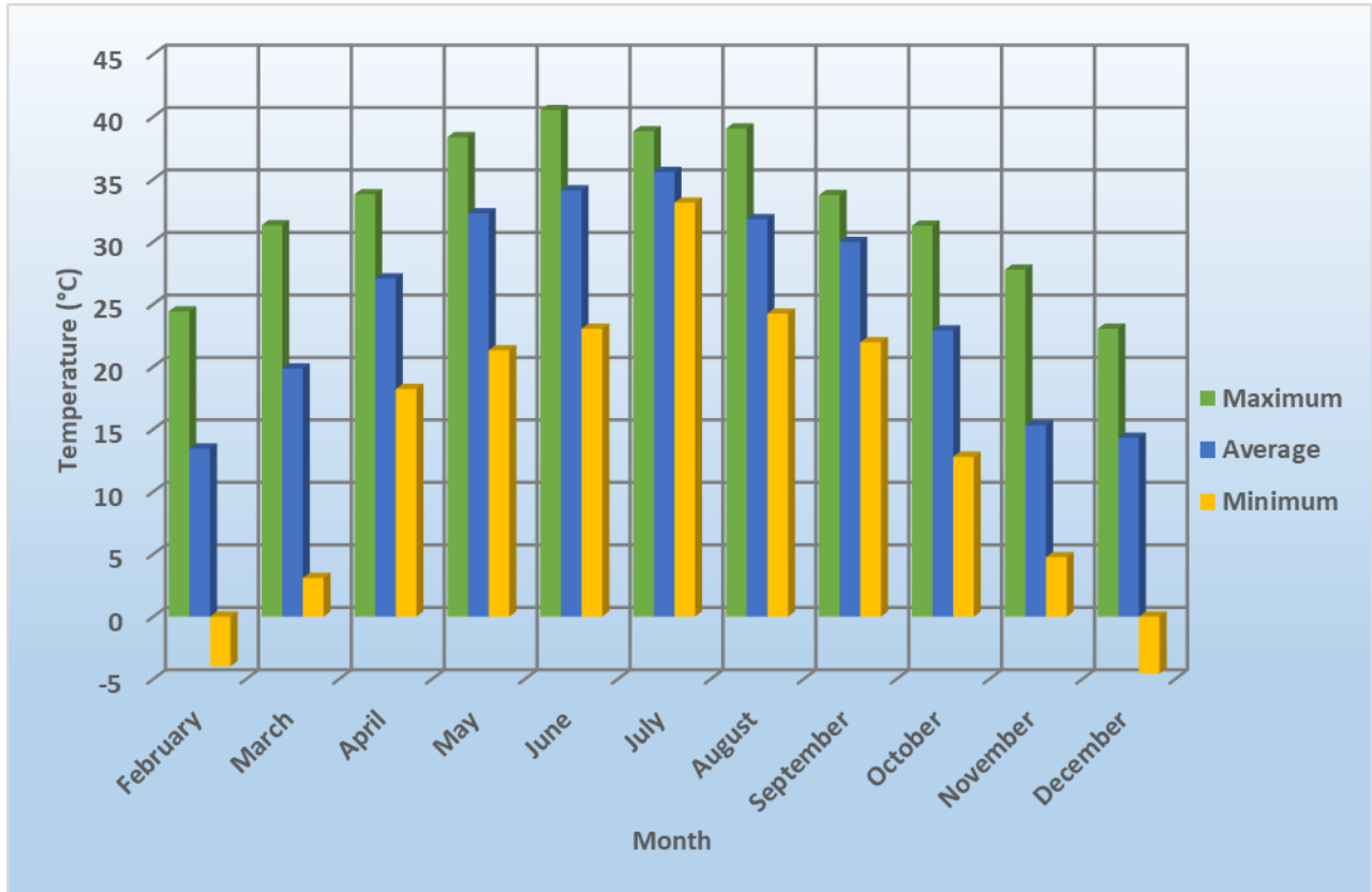
Figure 5.2 – WIPP Site High Temperatures (°C) for 2022
