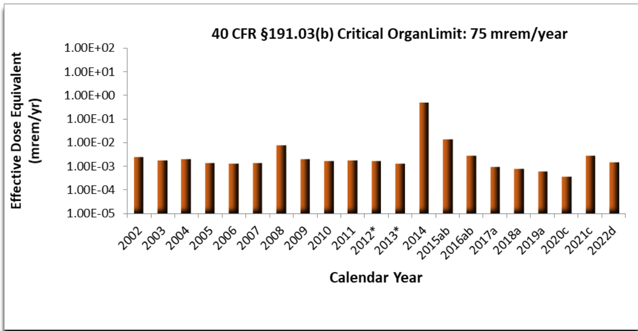
Figure 4.17 – Dose to the Critical Organ for Hypothetical Maximally Exposed Individual at the WIPP Fence Line
