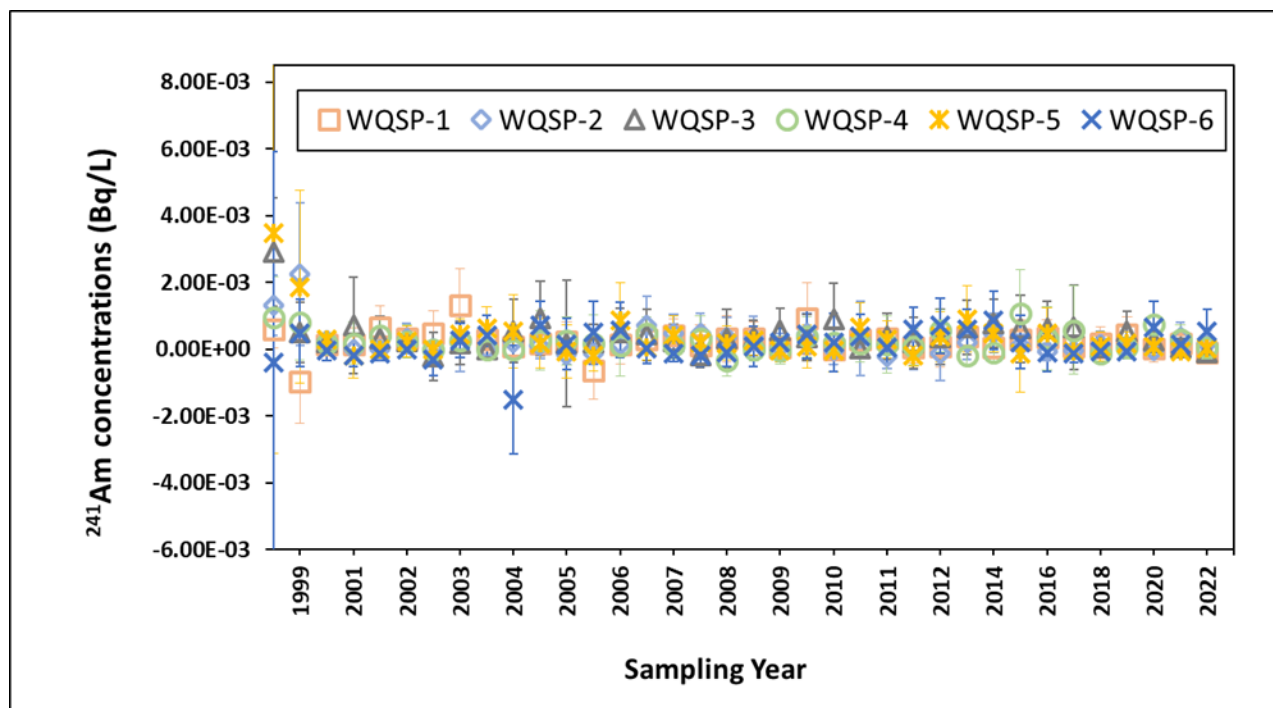
Figure 4.4b – Historical Concentrations of 241 Am at Six DMP Wells
