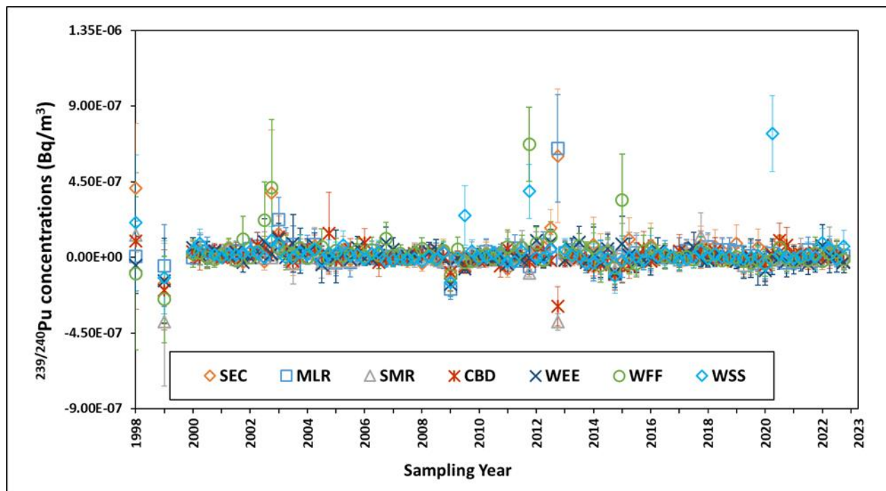
Figure 4.2a – Historical Concentrations of ^{239/240}\text{Pu} at Seven Air Sampling Locations
