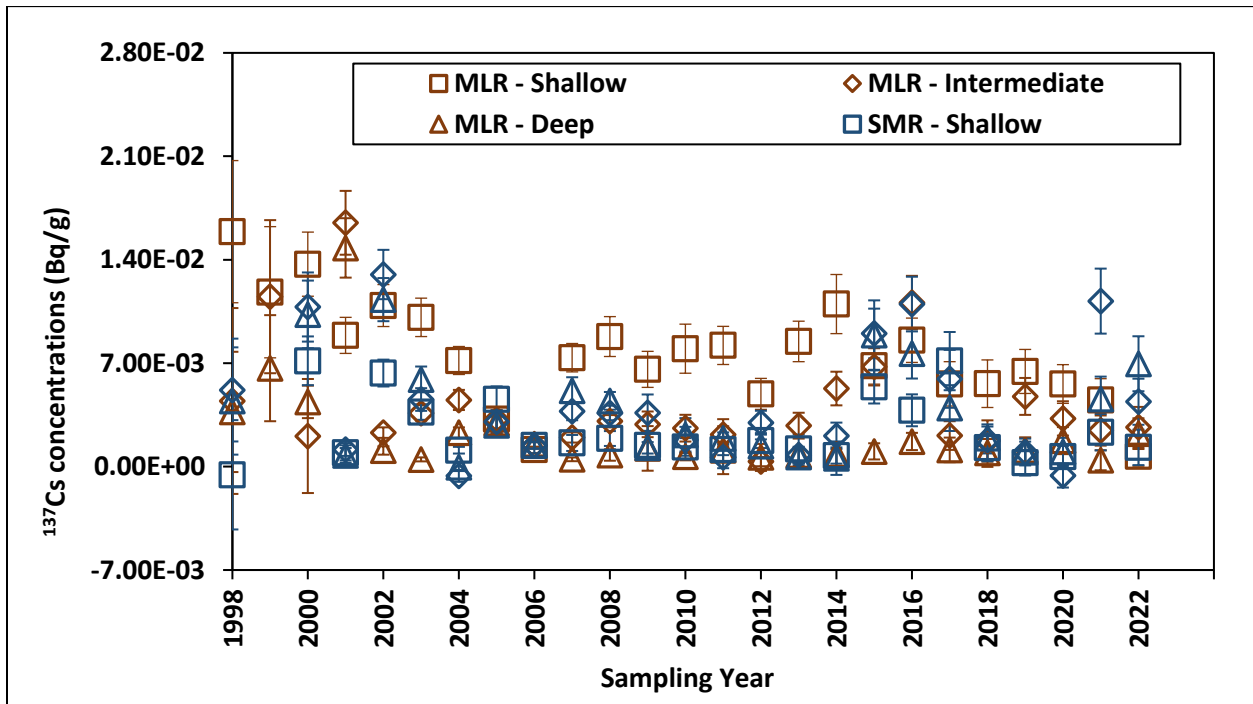
Figure 4.12b – ^{137}\text{Cs} Concentrations in Soil Samples Collected from 5-mi Ring
