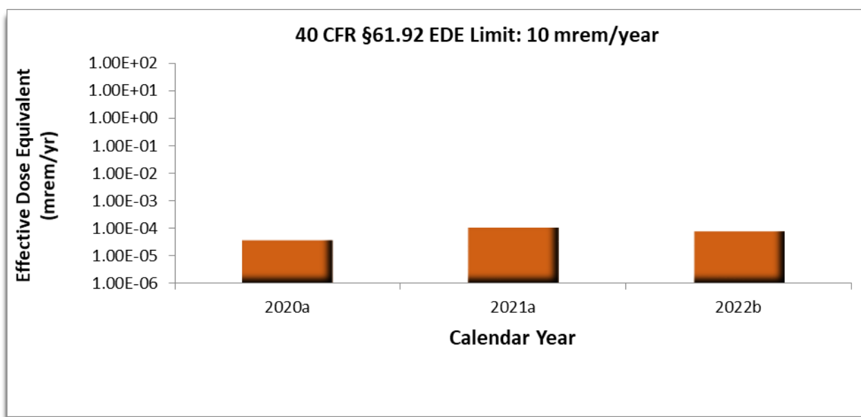
Figure 4.18 – WIPP Effective Dose Equivalent to the Maximally Exposed Individual
