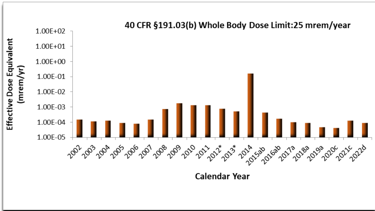
Figure 4.16 – Dose to the Whole Body for the Hypothetical Maximally Exposed Individual at the WIPP Fence Line
