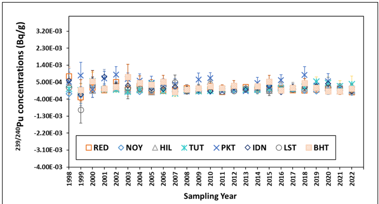
Figure 4.7b – Historical Concentrations of ^{239/240}\text{Pu} in Sediment Samples at Tanks and Tank-like Structures
