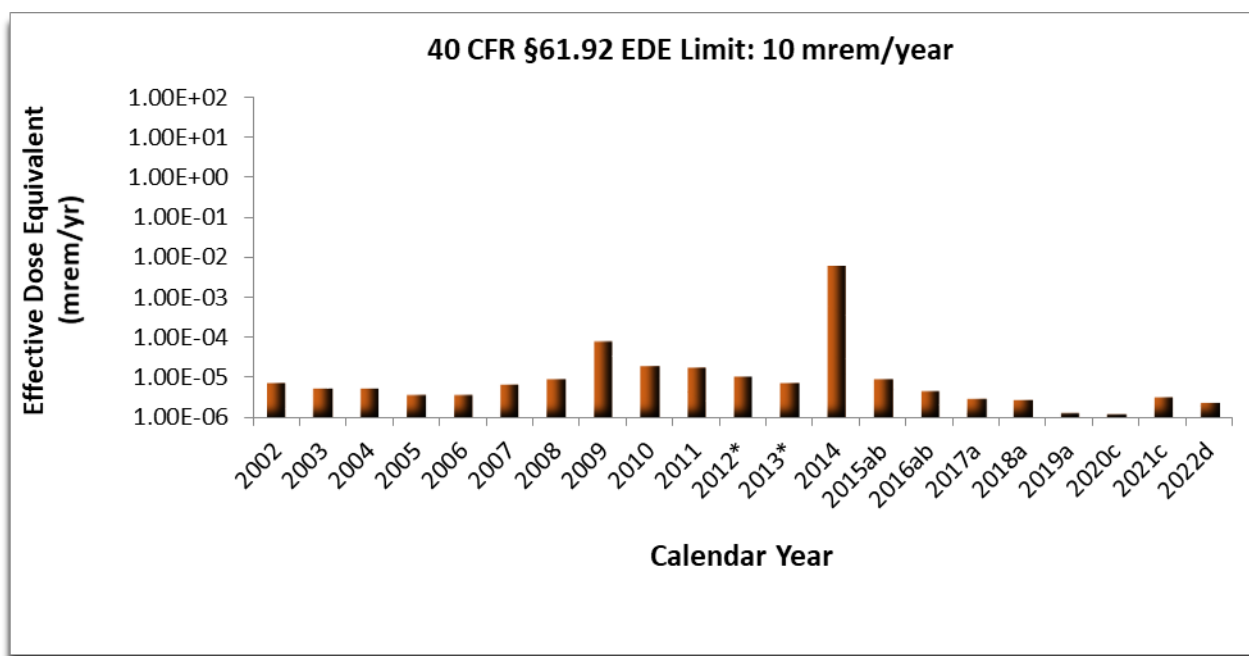
Figure 4.19 – WIPP Effective Dose Equivalent to the Off-Site Maximally Exposed Individual (i.e., individual resident member of the public)
