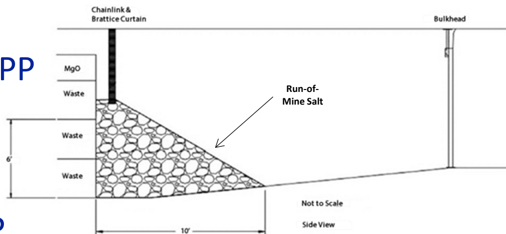
Initial Closure in Panel 6
