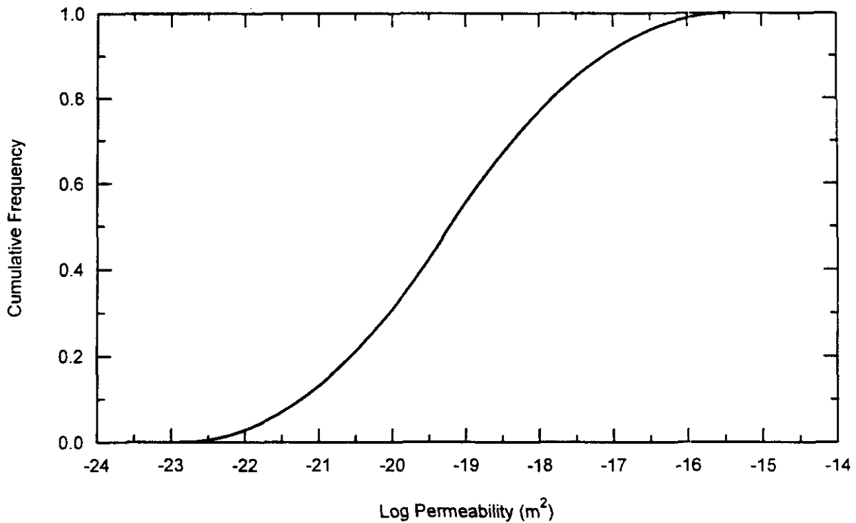
Figure A-8. Compacted salt column permeability cumulative frequency distribution function at seal midpoint 100 years following closure.
