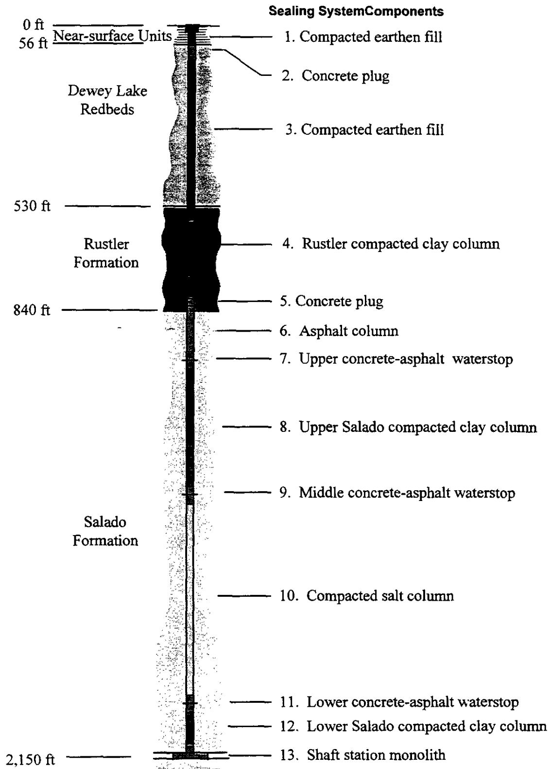
Figure A-1. Schematic of the WIPP shaft seal design.
