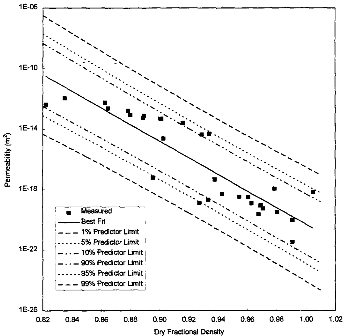
Figure A-7. Permeability of consolidated crushed salt as a function of fractional density.
