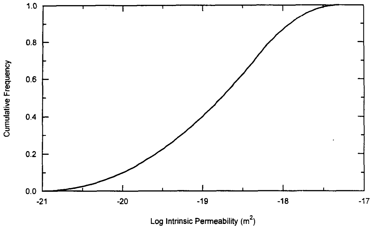
Figure A-4. Cumulative frequency distribution for compacted bentonite.
