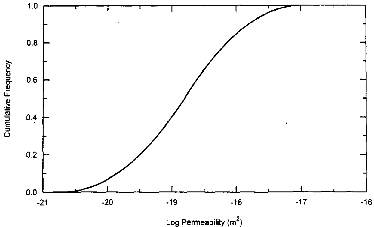
Figure A-2. Cumulative distribution function for SMC.
