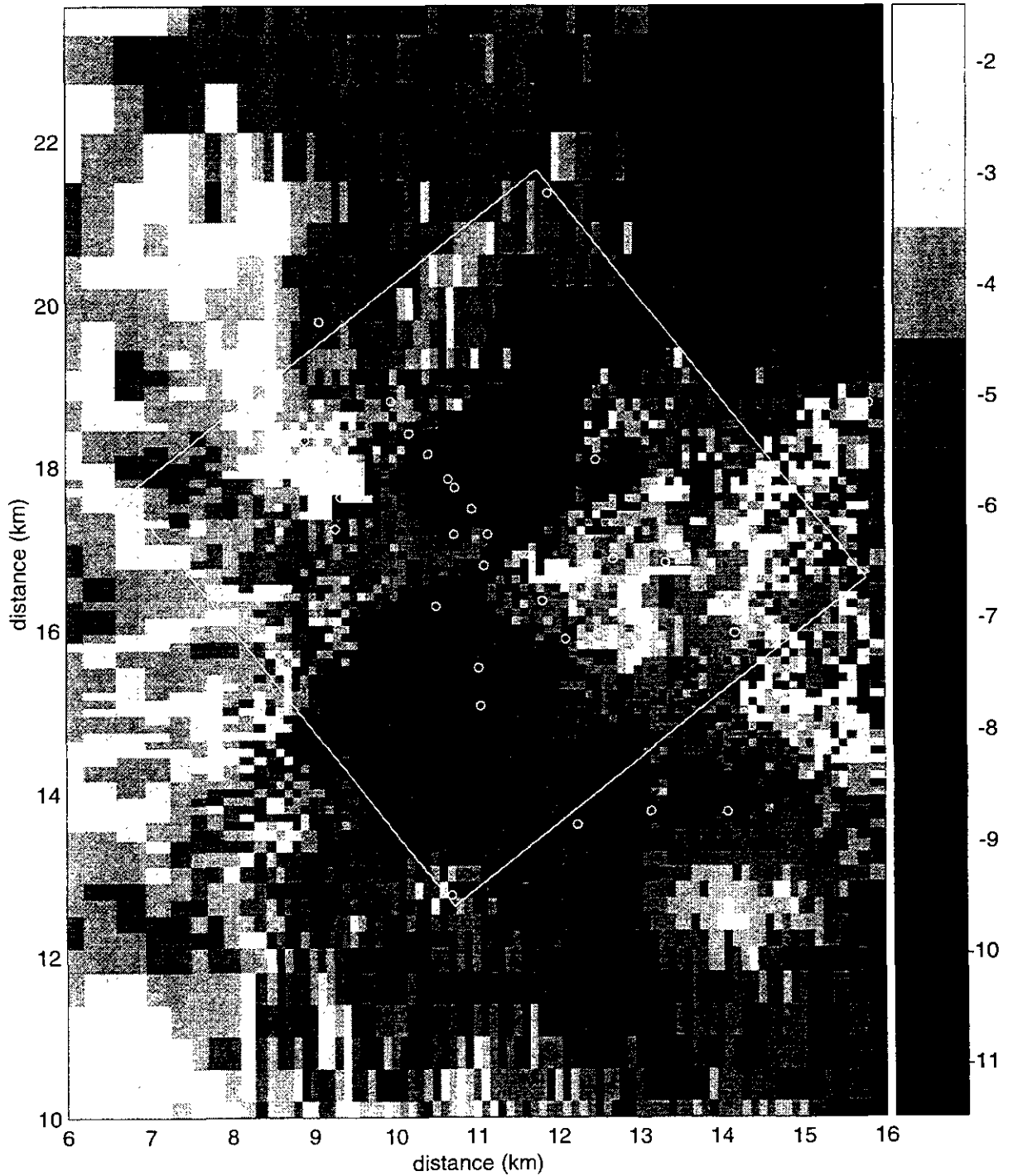
Figure TFIELD-A-34. Transient Calibrated Transmissivity Field no. 17, WIPP-scale.
