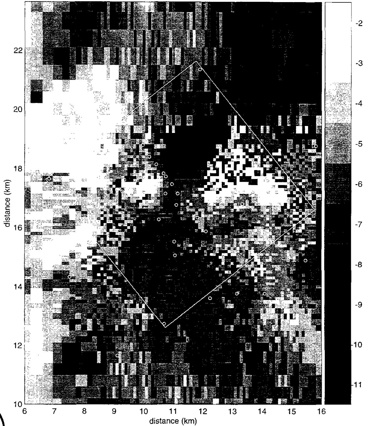
Figure TFIELD-A-102. Transient Calibrated Transmissivity Field no. 51, WIPP-scale.
