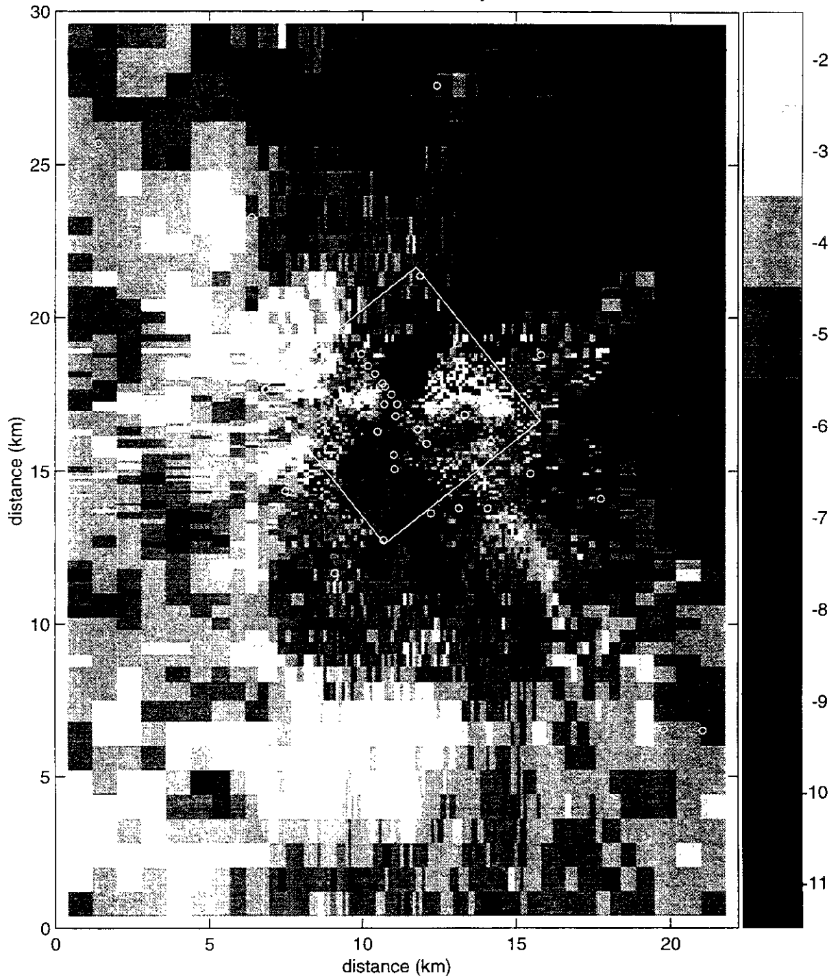
Figure TFIELD-A-101. Transient Calibrated Transmissivity Field no. 51, full-scale.
