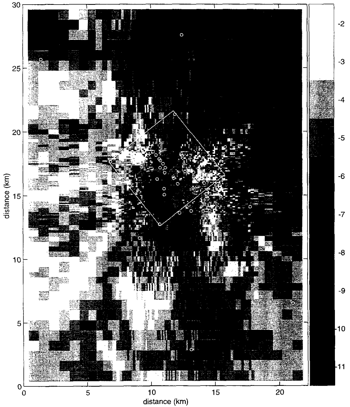
Figure TFIELD-A-13. Transient Calibrated Transmissivity Field no. 7, full-scale.
