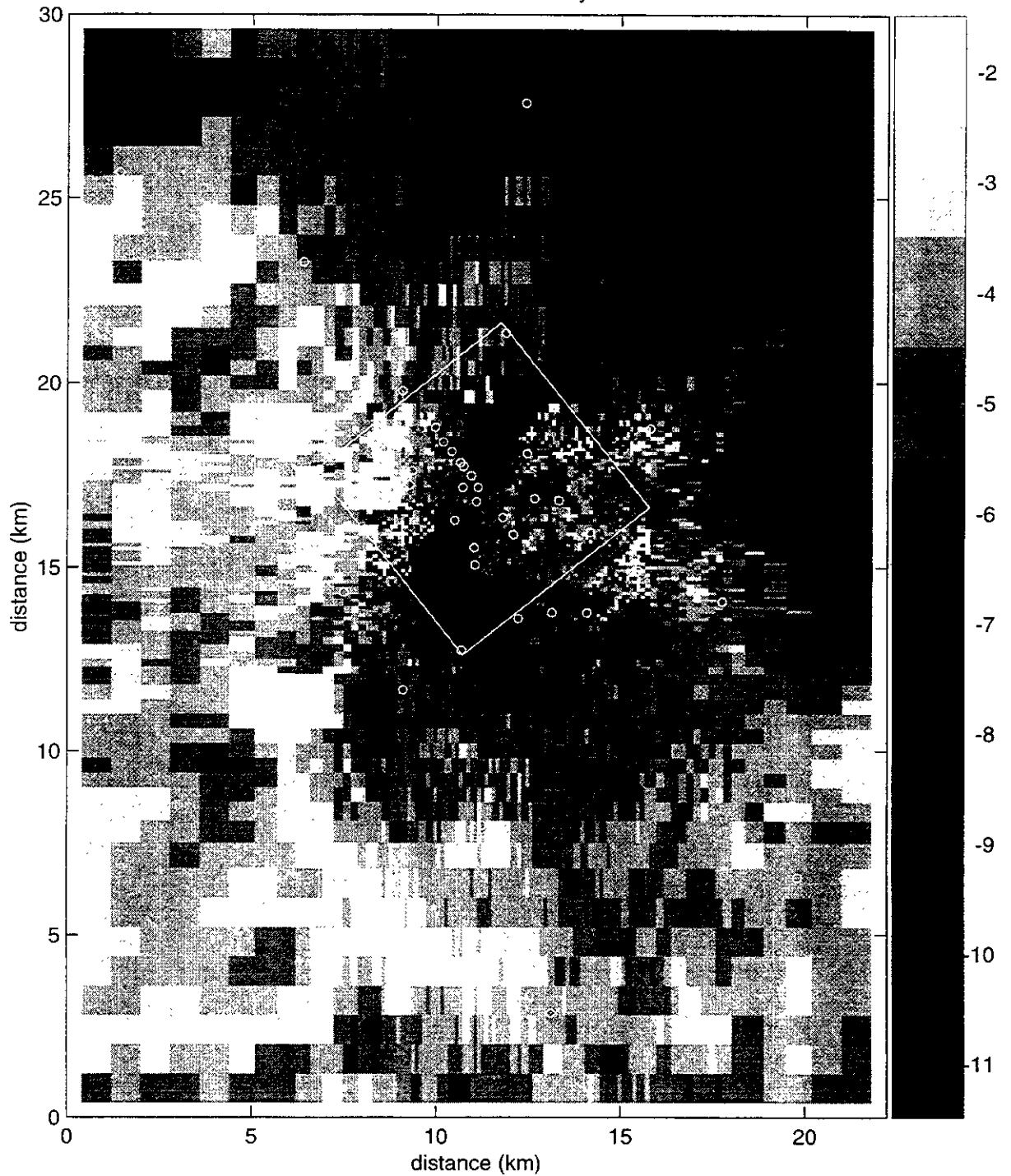
Figure TFIELD-A-131. Transient Calibrated Transmissivity Field no. 66, full-scale.
