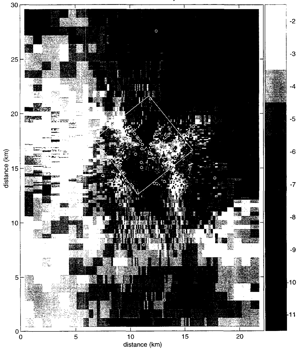
Figure TFIELD-A-17. Transient Calibrated Transmissivity Field no. 9, full-scale.
