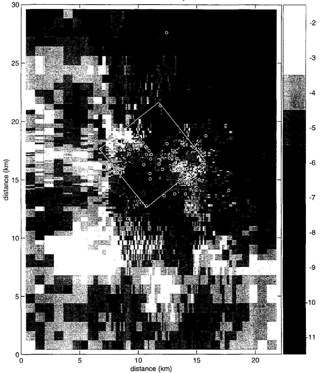
Figure TFIELD-A-75. Transient Calibrated Transmissivity Field no. 38, full-scale.
