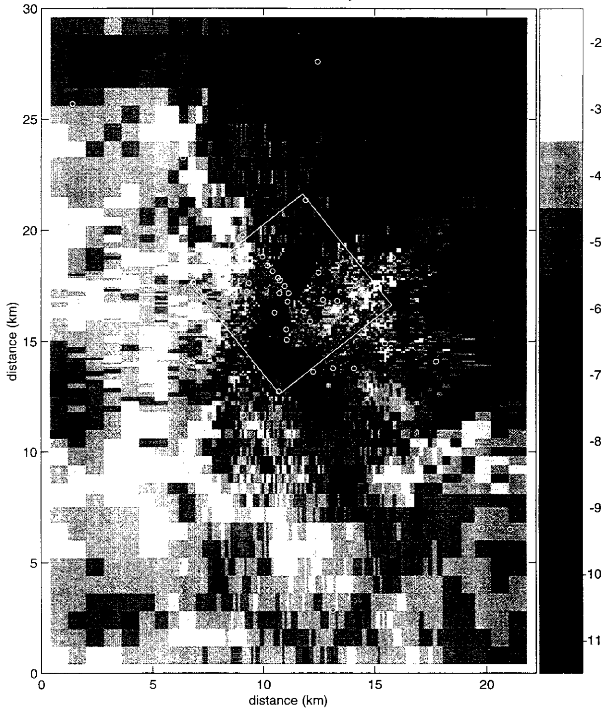
Figure TFIELD-A-111. Transient Calibrated Transmissivity Field no. 56, full-scale.
