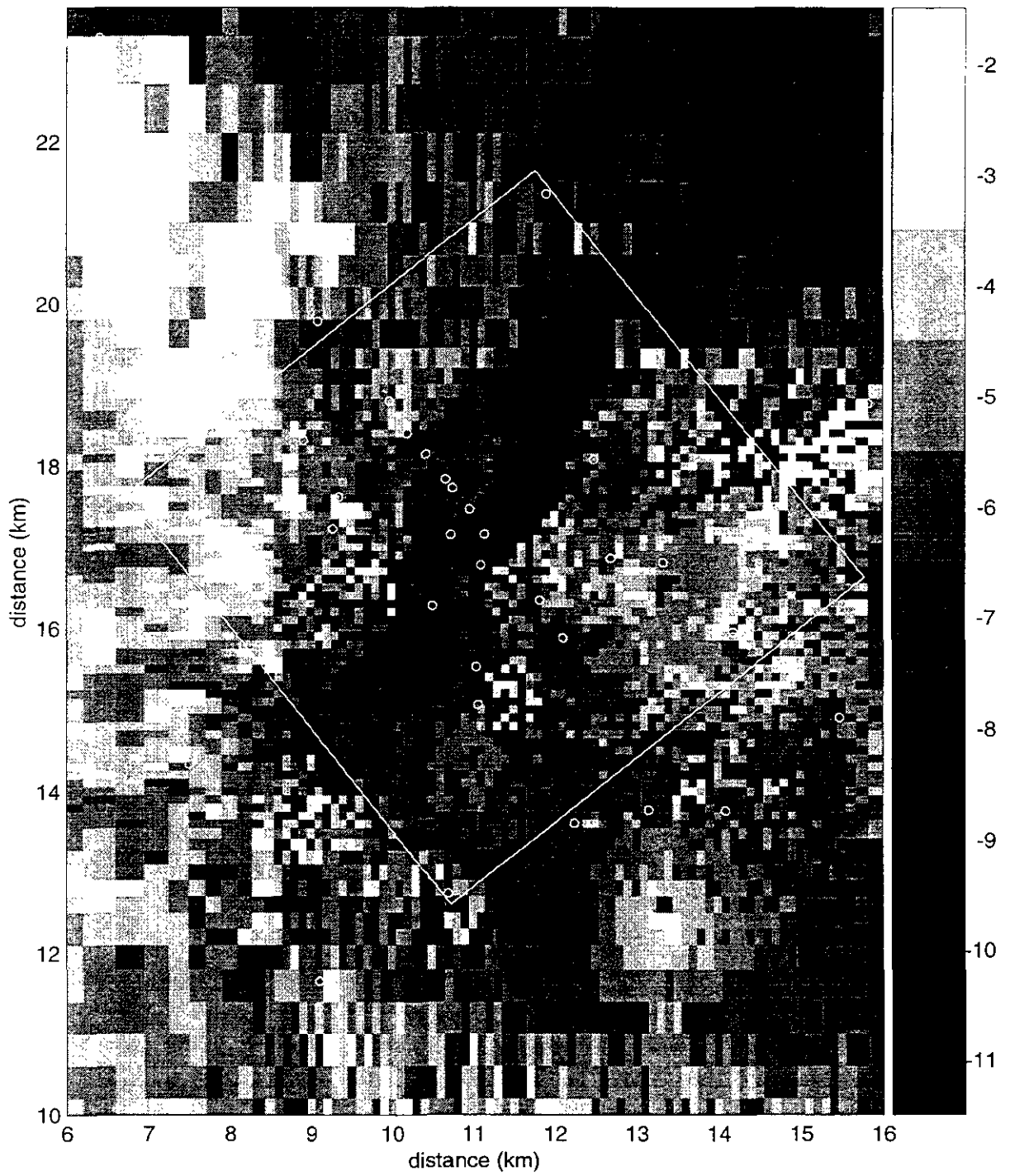
Figure TFIELD-A-120. Transient Calibrated Transmissivity Field no. 60, WIPP-scale.
