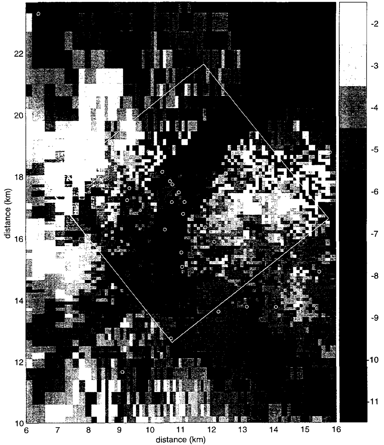
Figure TFIELD-A-74. Transient Calibrated Transmissivity Field no. 37, WIPP-scale.
