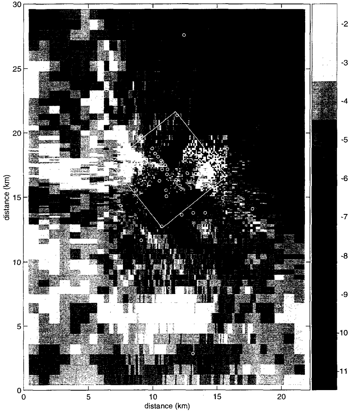
Figure TFIELD-A-197. Transient Calibrated Transmissivity Field no. 99, full-scale.
