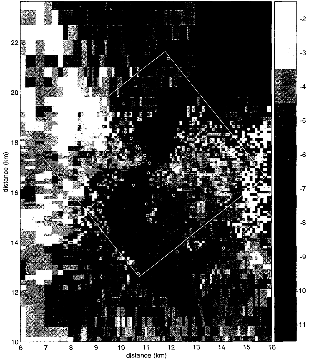
Figure TFIELD-A-56. Transient Calibrated Transmissivity Field no. 28, WIPP-scale.
