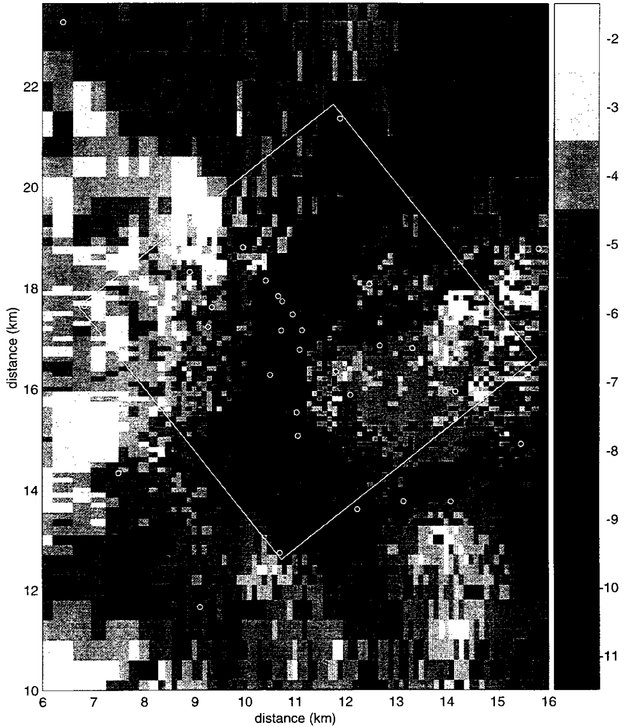
Figure TFIELD-A-48. Transient Calibrated Transmissivity Field no. 24, WIPP-scale.
