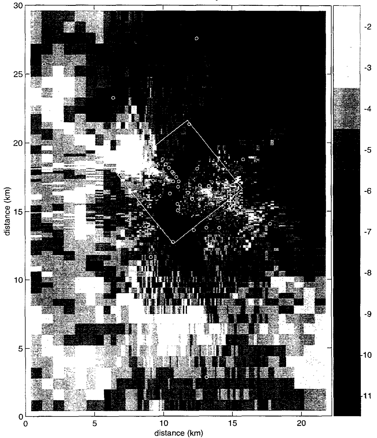
Figure TFIELD-A-125. Transient Calibrated Transmissivity Field no. 63, full-scale.
