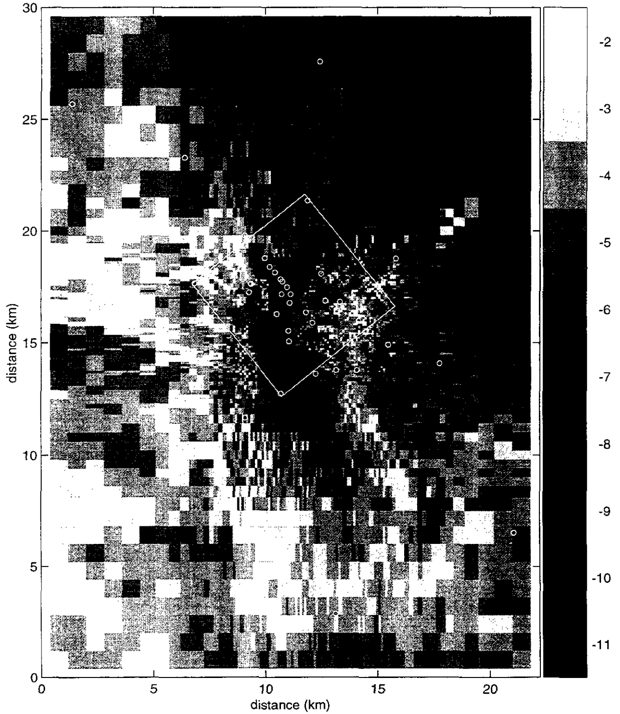
Figure TFIELD-A-199. Transient Calibrated Transmissivity Field no. 100, full-scale.
