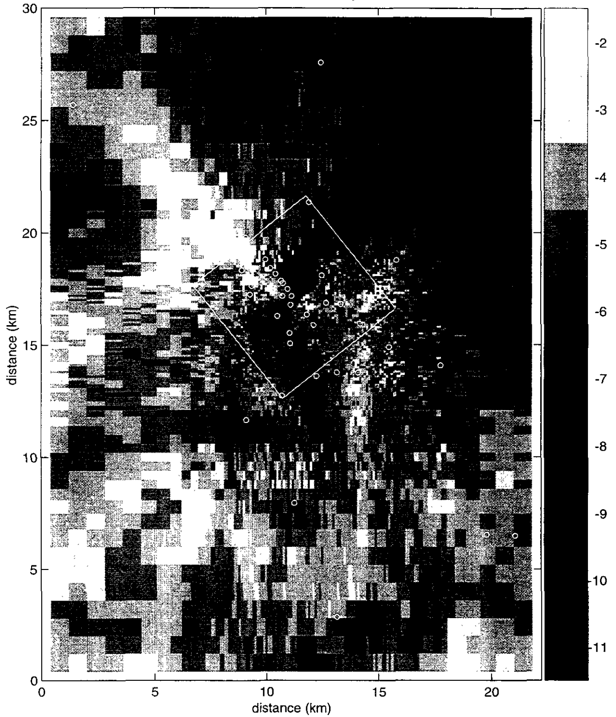
Figure TFIELD-A-137. Transient Calibrated Transmissivity Field no. 69, full-scale.
