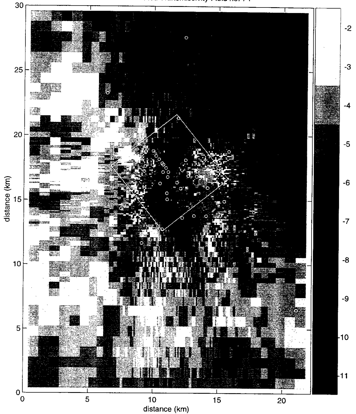
Figure TFIELD-A-147. Transient Calibrated Transmissivity Field no. 74, full-scale.
