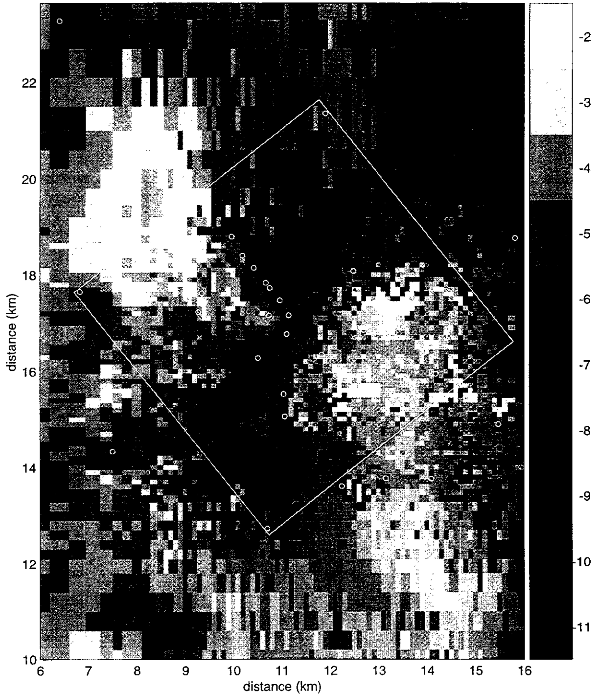
Figure TFIELD-A-88. Transient Calibrated Transmissivity Field no. 44, WIPP-scale.
