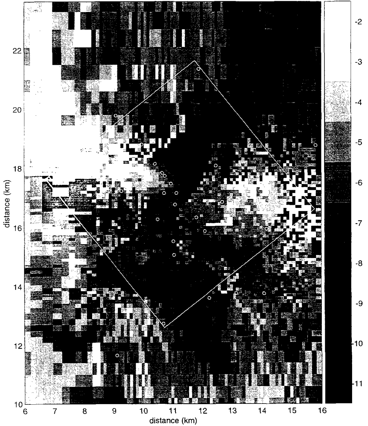
Figure TFIELD-A-140. Transient Calibrated Transmissivity Field no. 70, WIPP-scale.
