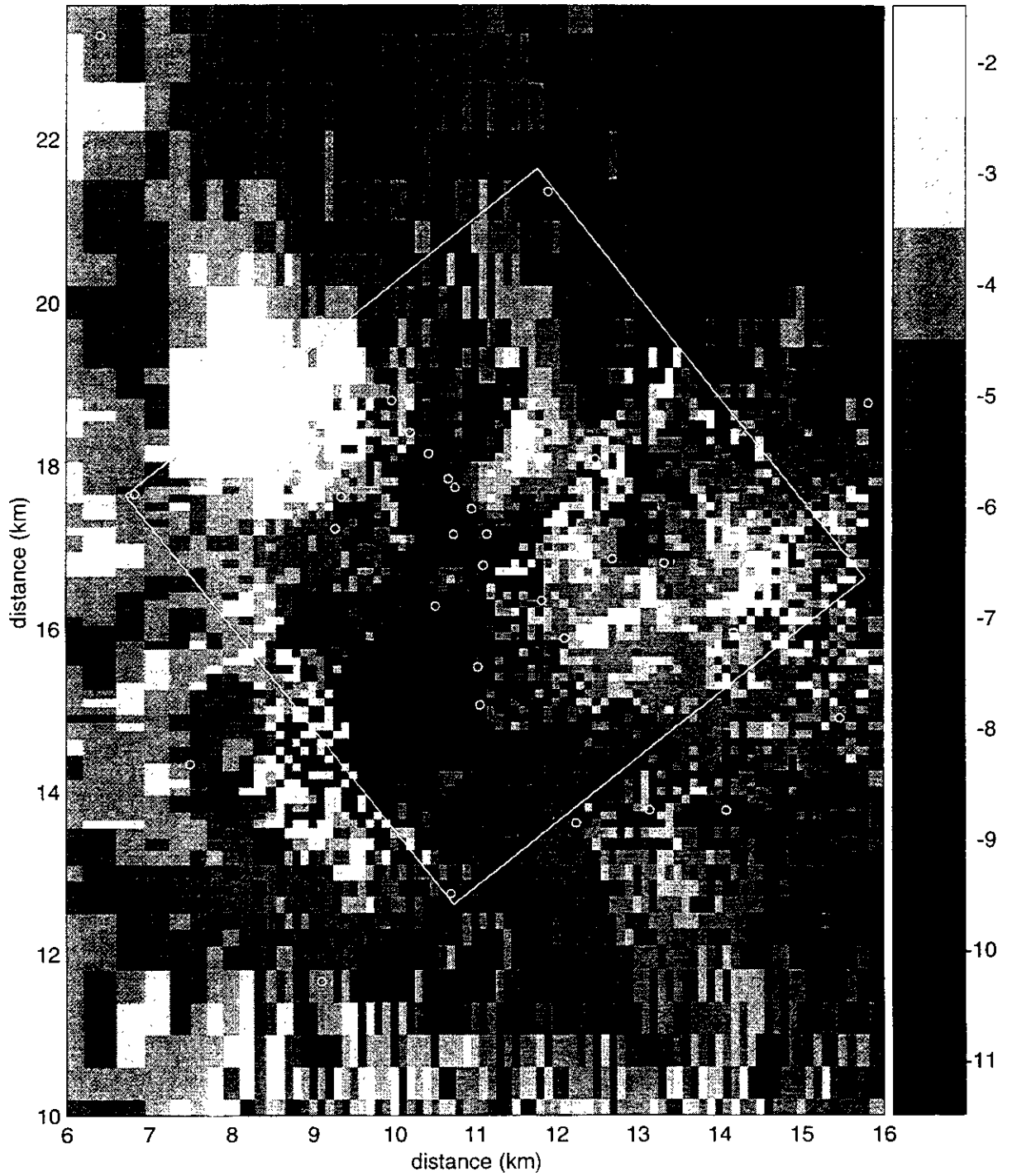
Figure TFIELD-A-68. Transient Calibrated Transmissivity Field no. 34, WIPP-scale.
