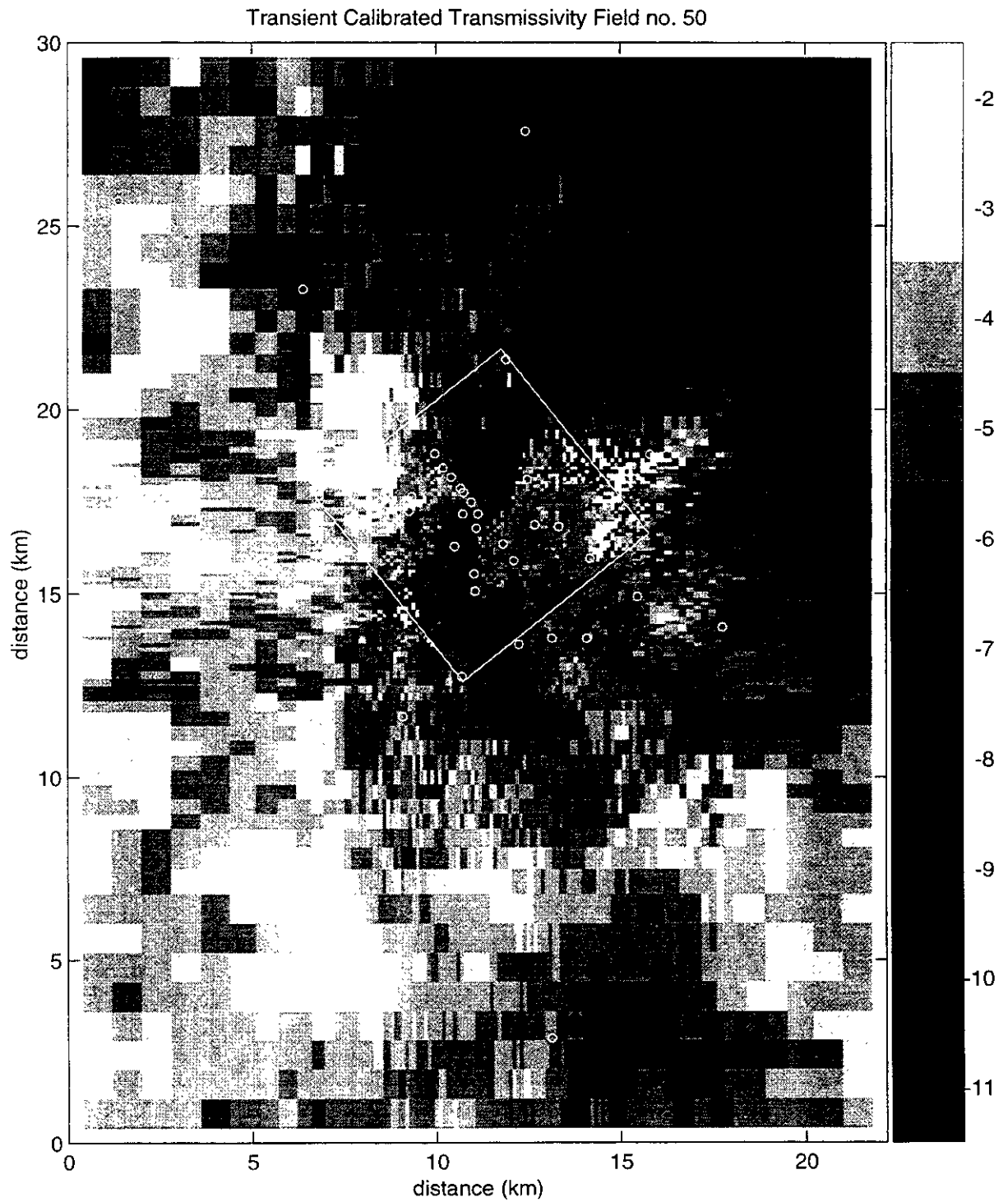
Figure TFIELD-A-99. Transient Calibrated Transmissivity Field no. 50, full-scale.
