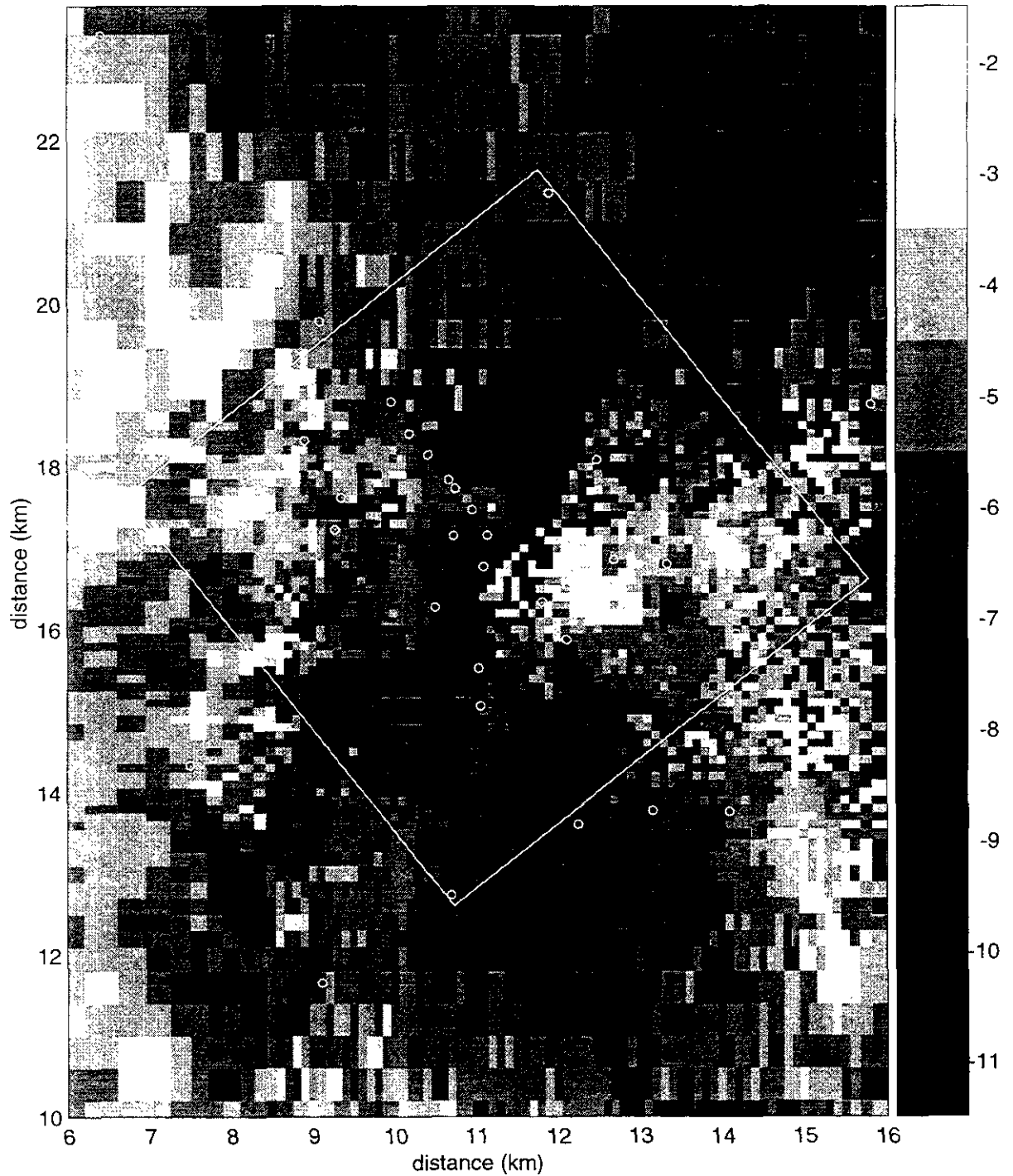
Figure TFIELD-A-194. Transient Calibrated Transmissivity Field no. 97, WIPP-scale.
