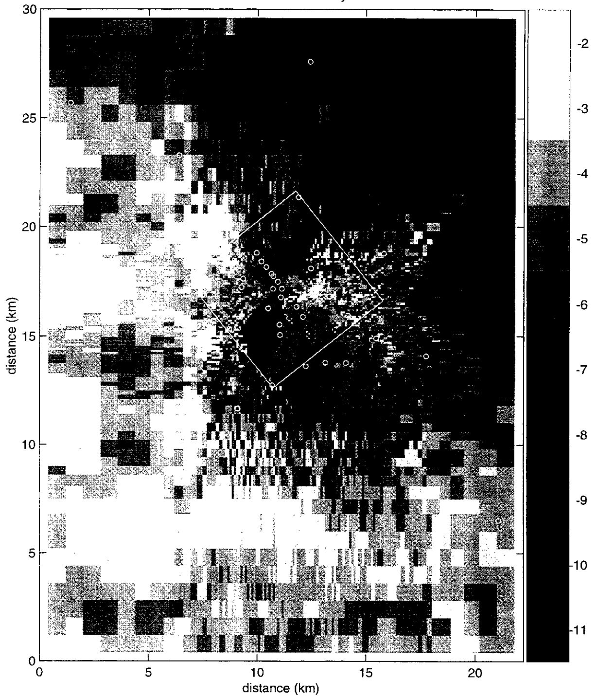
Figure TFIELD-A-43. Transient Calibrated Transmissivity Field no. 22, full-scale.
