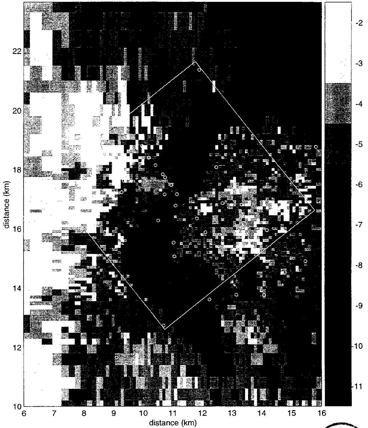
Figure TFIELD-A-2. Transient Calibrated Transmissivity Field no. 1, WIPP-scale.
