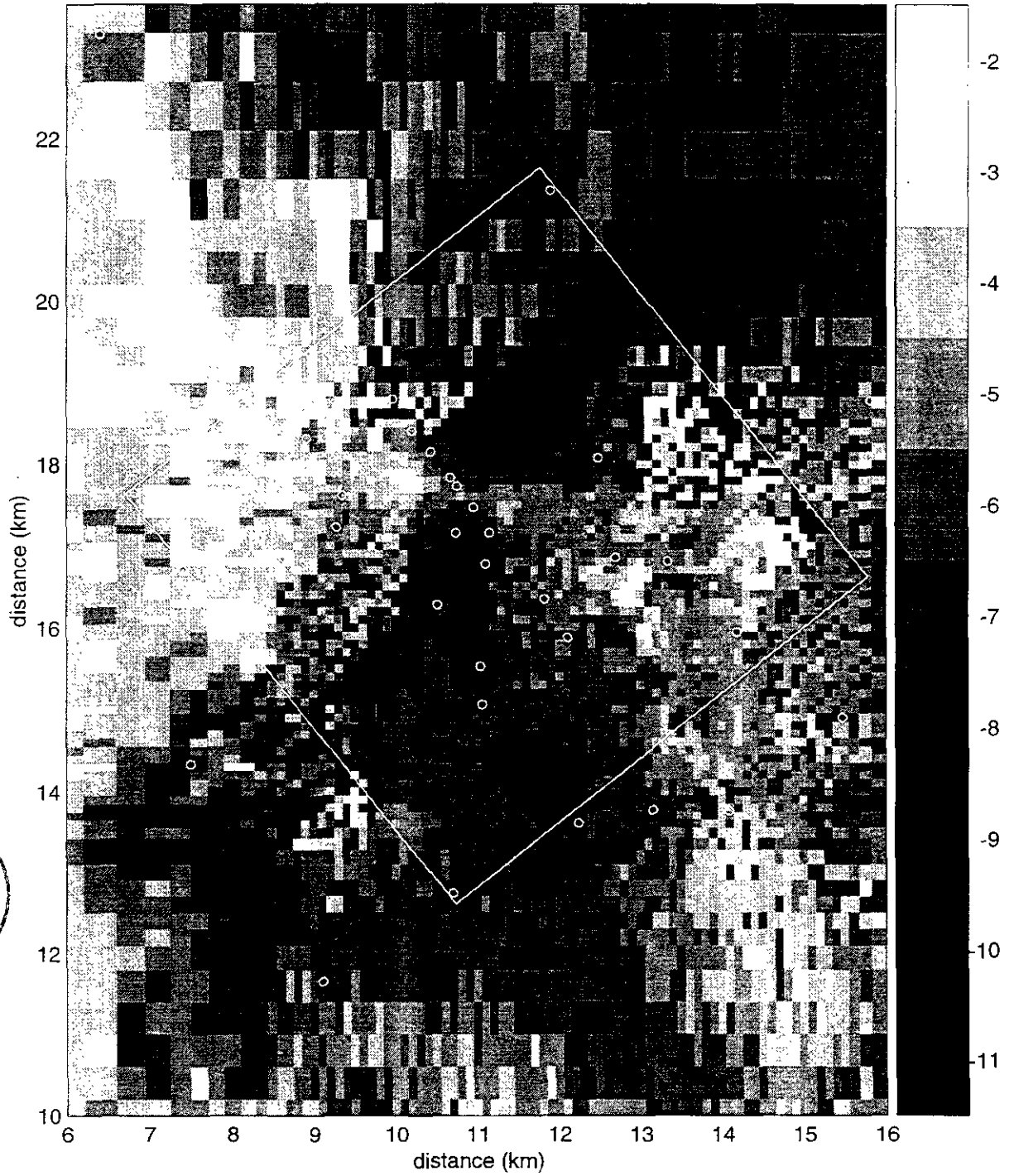
Figure TFIELD-A-110. Transient Calibrated Transmissivity Field no. 55, WIPP-scale.
