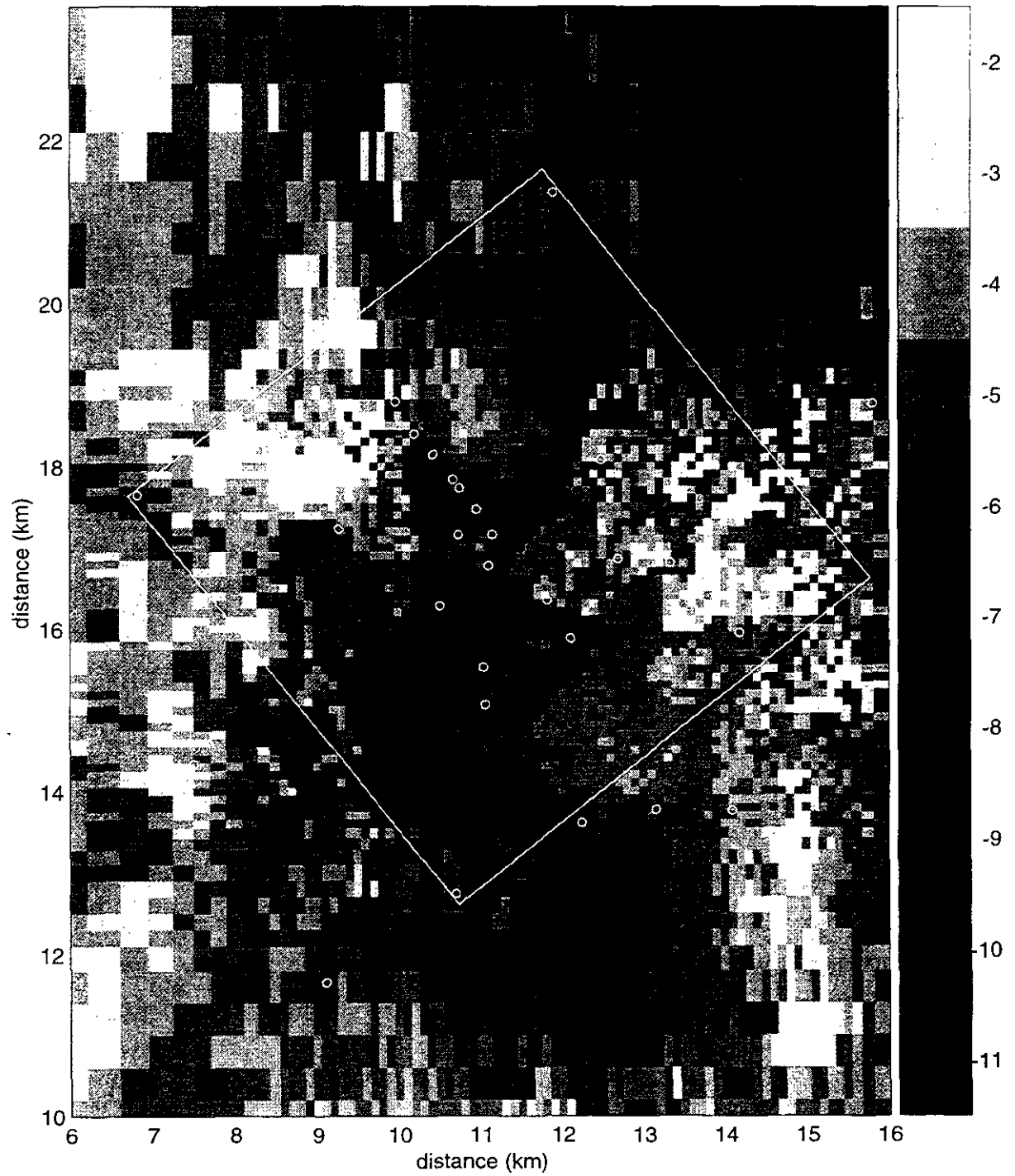
Figure TFIELD-A-14. Transient Calibrated Transmissivity Field no. 7, WIPP-scale.
