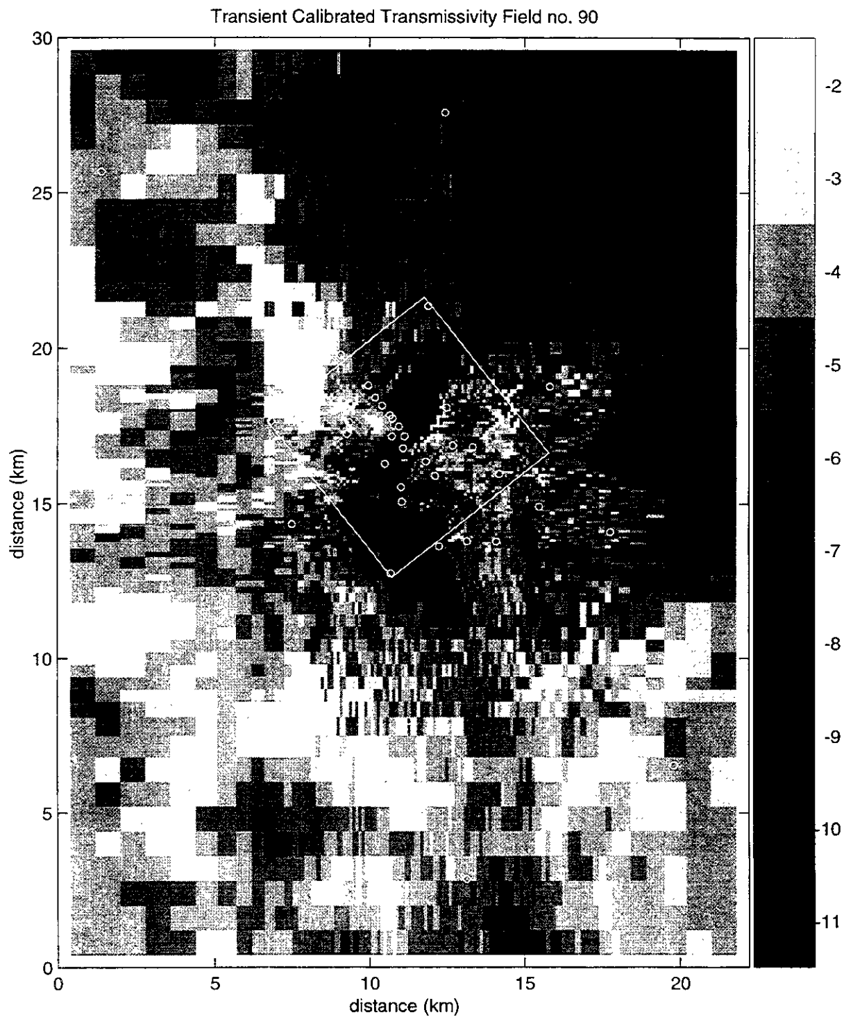
Figure TFIELD-A-179. Transient Calibrated Transmissivity Field no. 90, full-scale.
