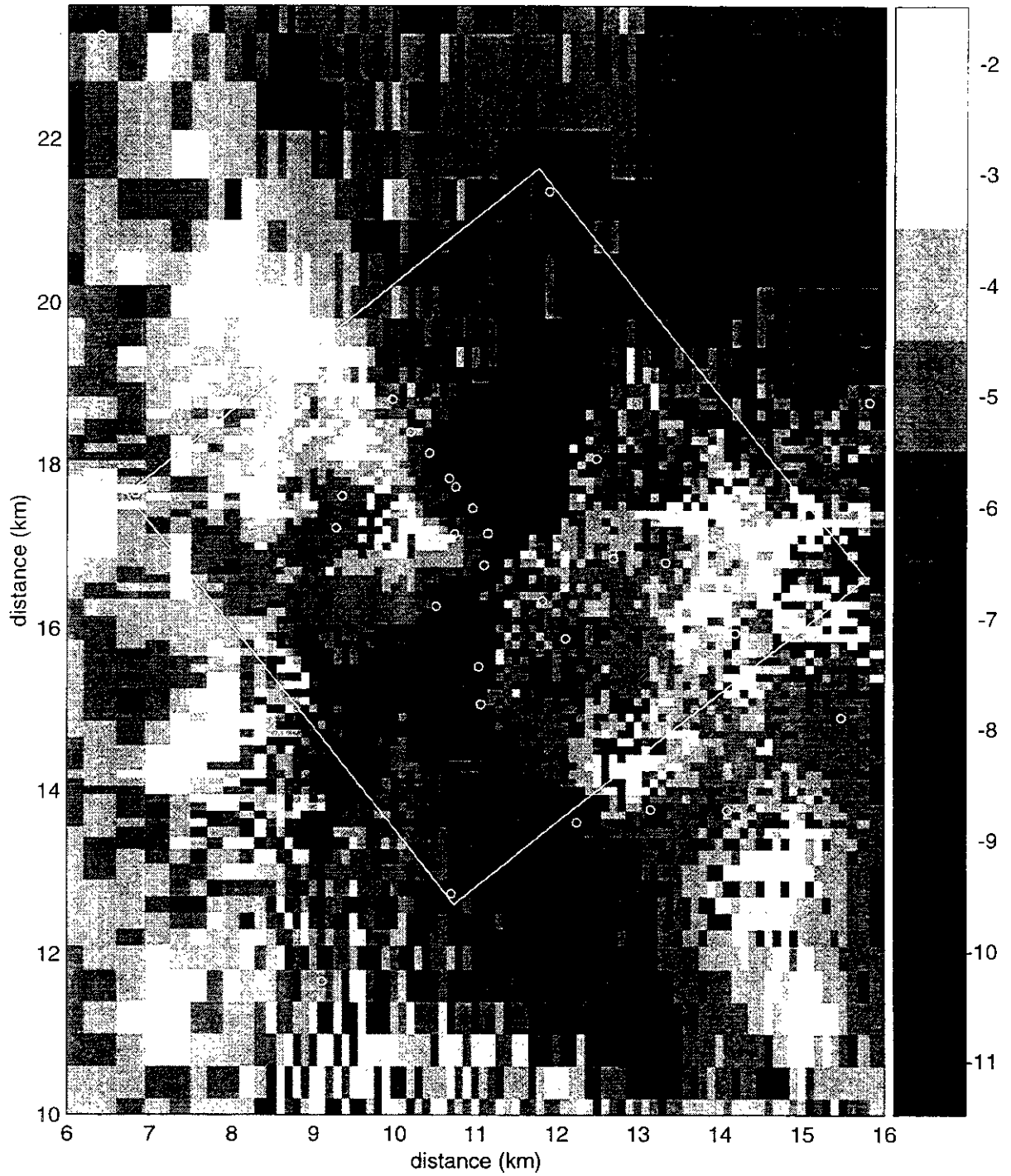
Figure TFIELD-A-192. Transient Calibrated Transmissivity Field no. 96, WIPP-scale.
