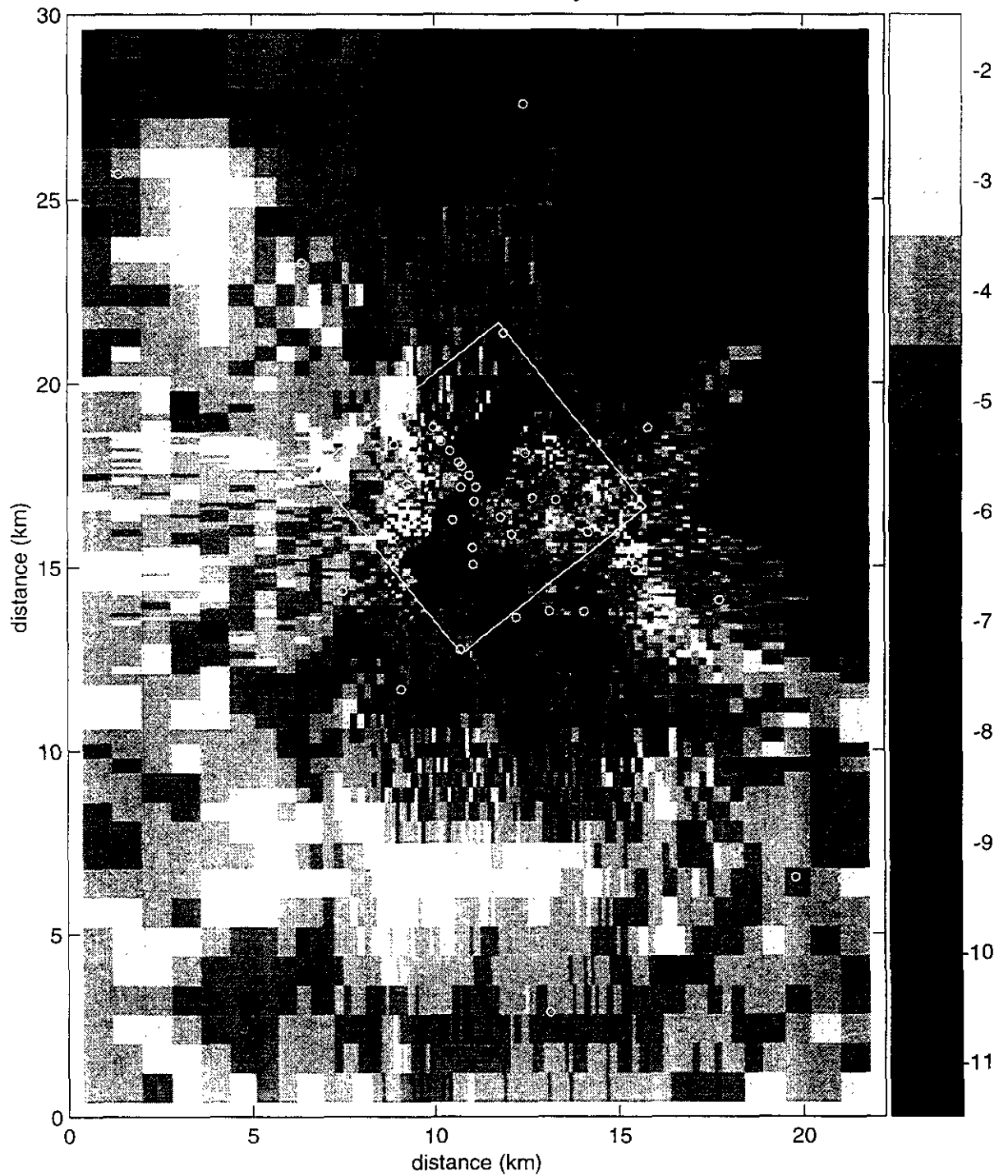
Figure TFIELD-A-143. Transient Calibrated Transmissivity Field no. 72, full-scale.
