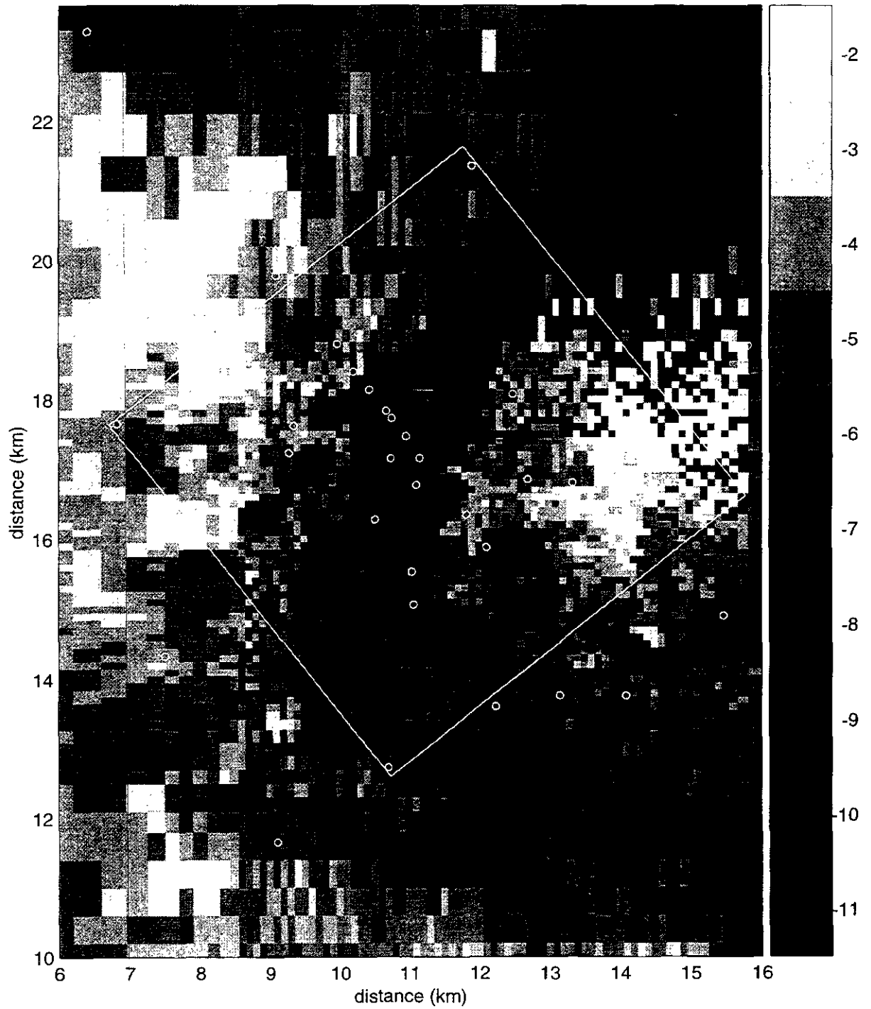
Figure TFIELD-A-26. Transient Calibrated Transmissivity Field no. 13, WIPP-scale.
