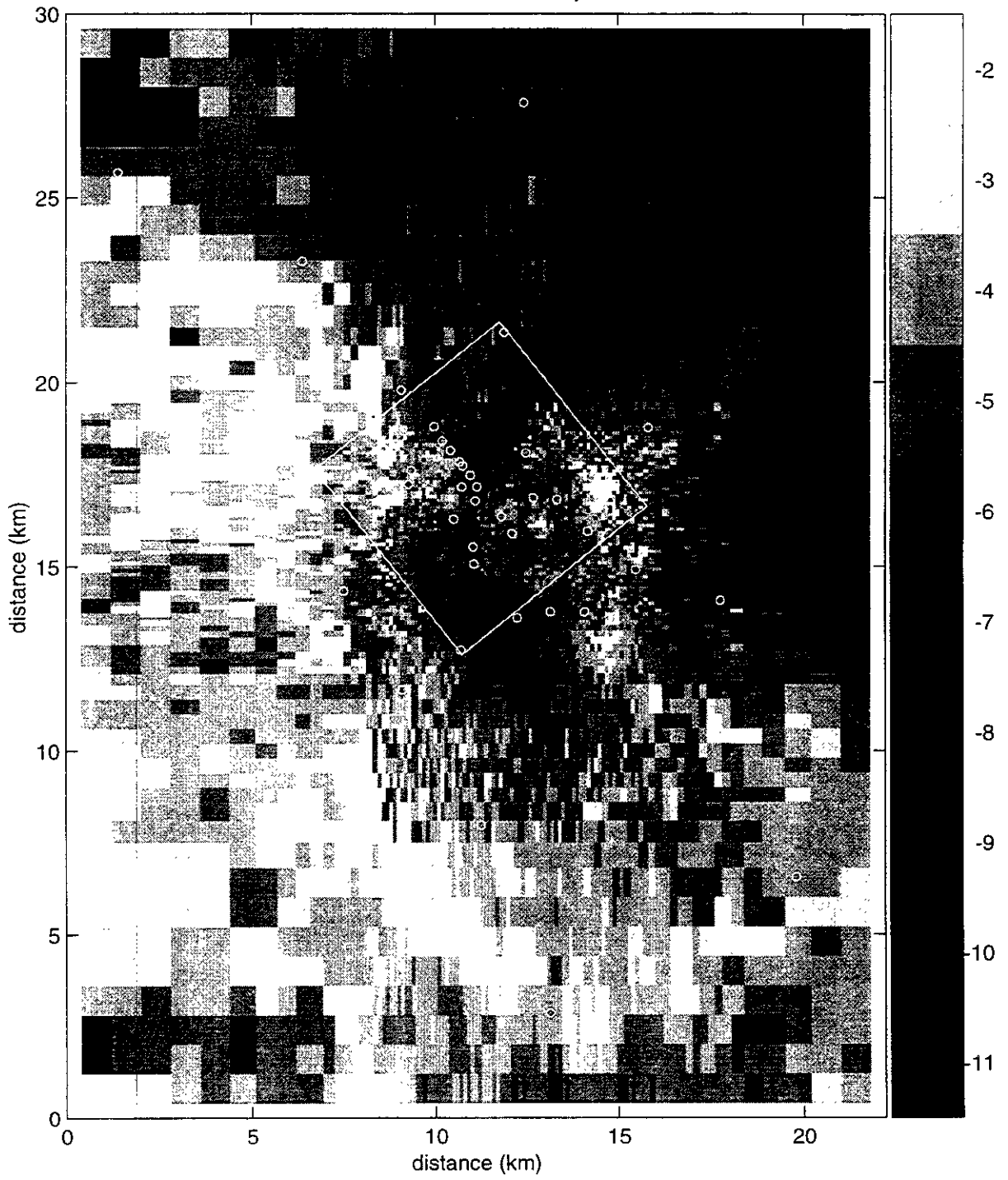
Figure TFIELD-A-97. Transient Calibrated Transmissivity Field no. 49, full-scale.
