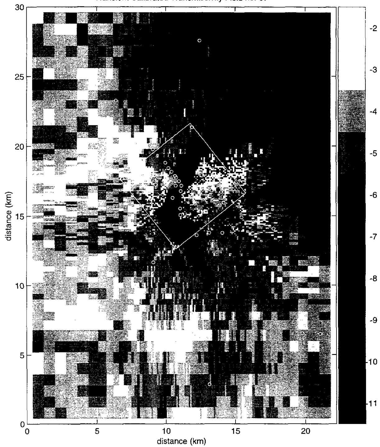
Figure TFIELD-A-133. Transient Calibrated Transmissivity Field no. 67, full-scale.
