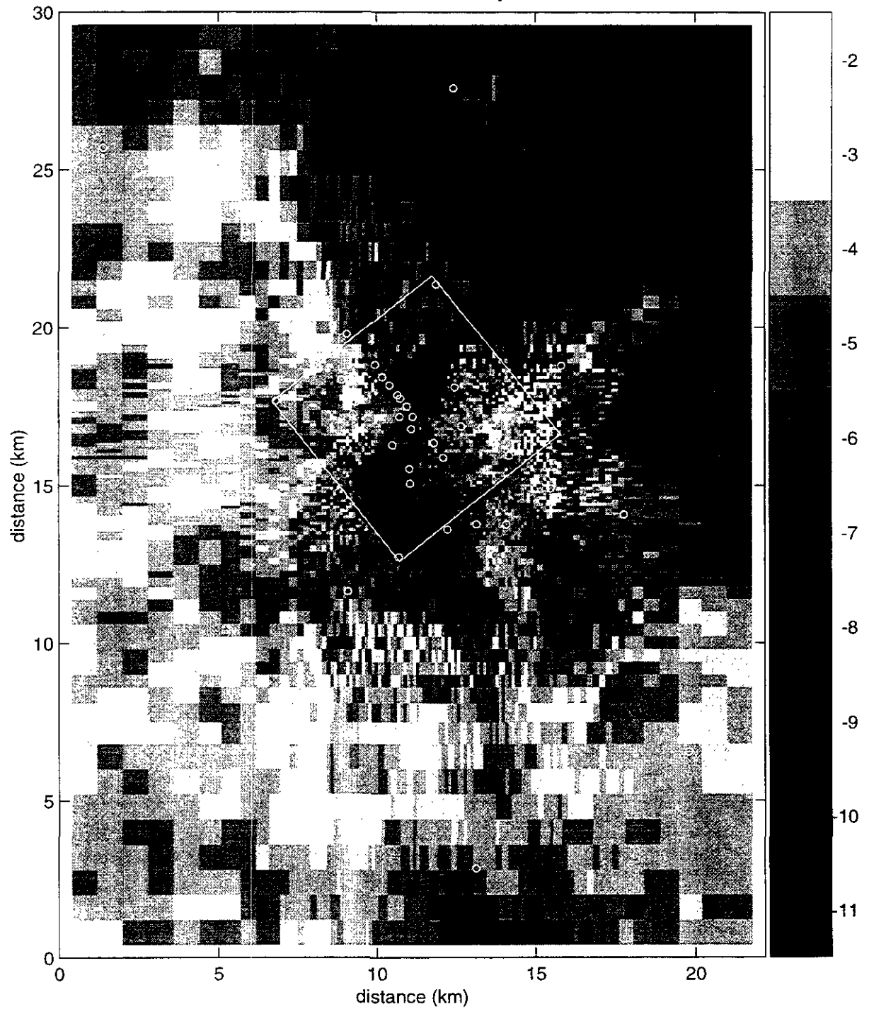
Figure TFIELD-A-69. Transient Calibrated Transmissivity Field no. 35, full-scale.
