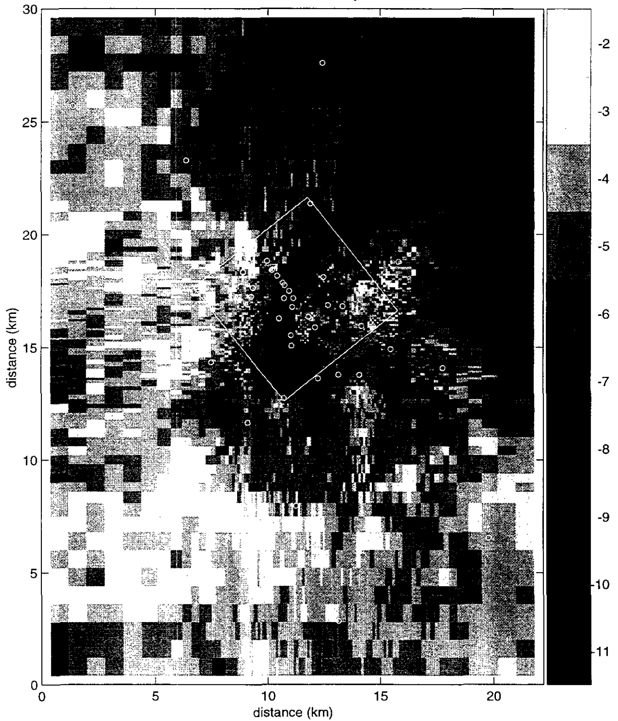
Figure TFIELD-A-47. Transient Calibrated Transmissivity Field no. 24, full-scale.
