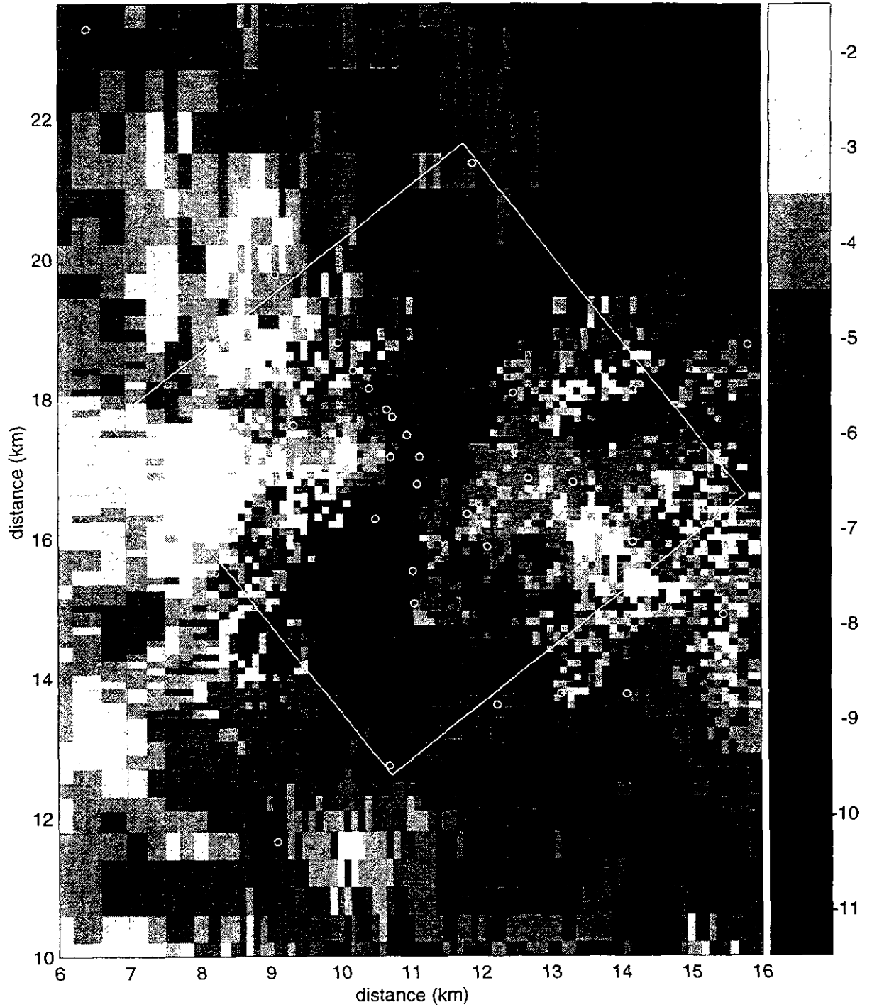
Figure TFIELD-A-50. Transient Calibrated Transmissivity Field no. 25, WIPP-scale.
