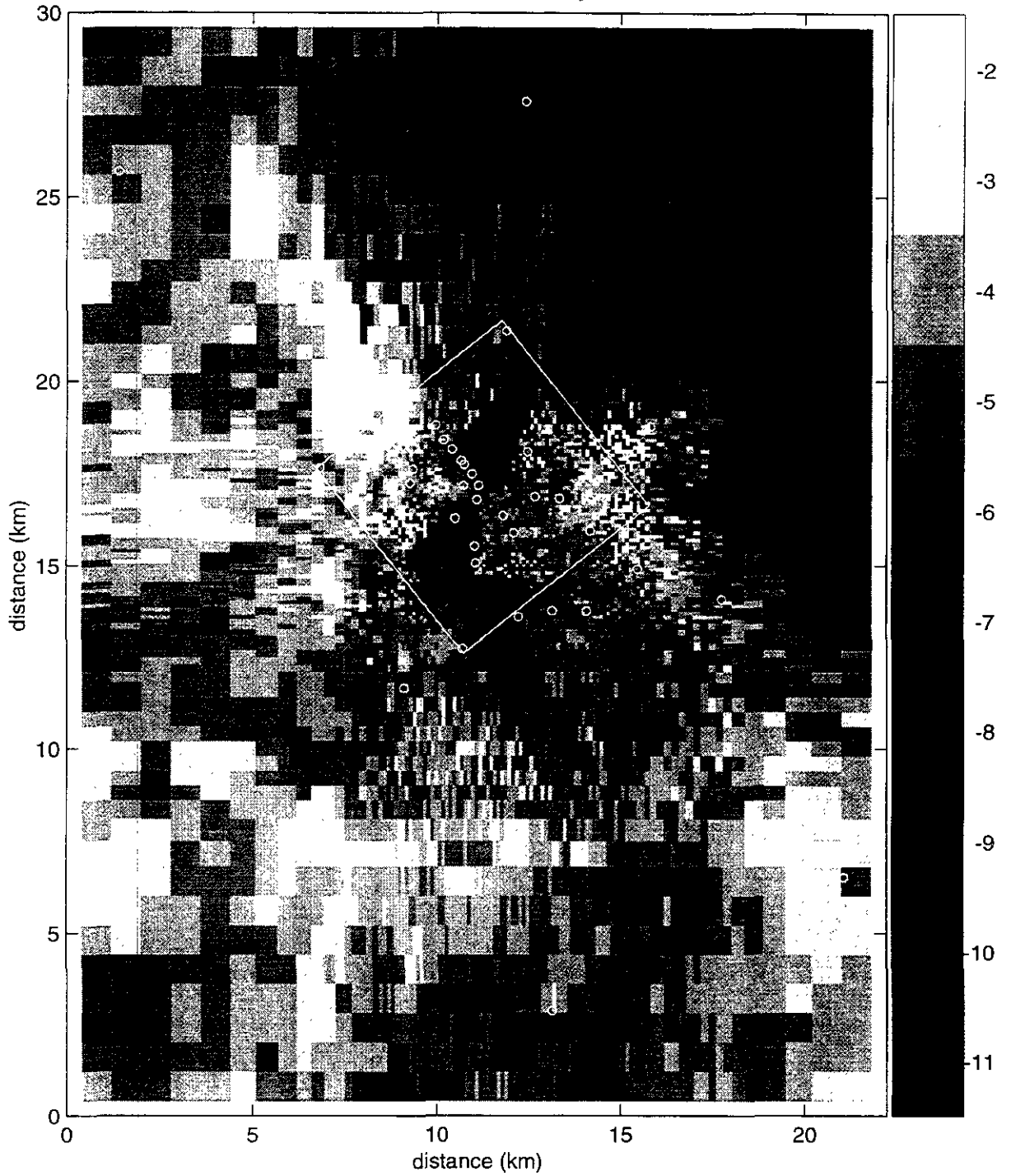
Figure TFIELD-A-81. Transient Calibrated Transmissivity Field no. 41, full-scale.
