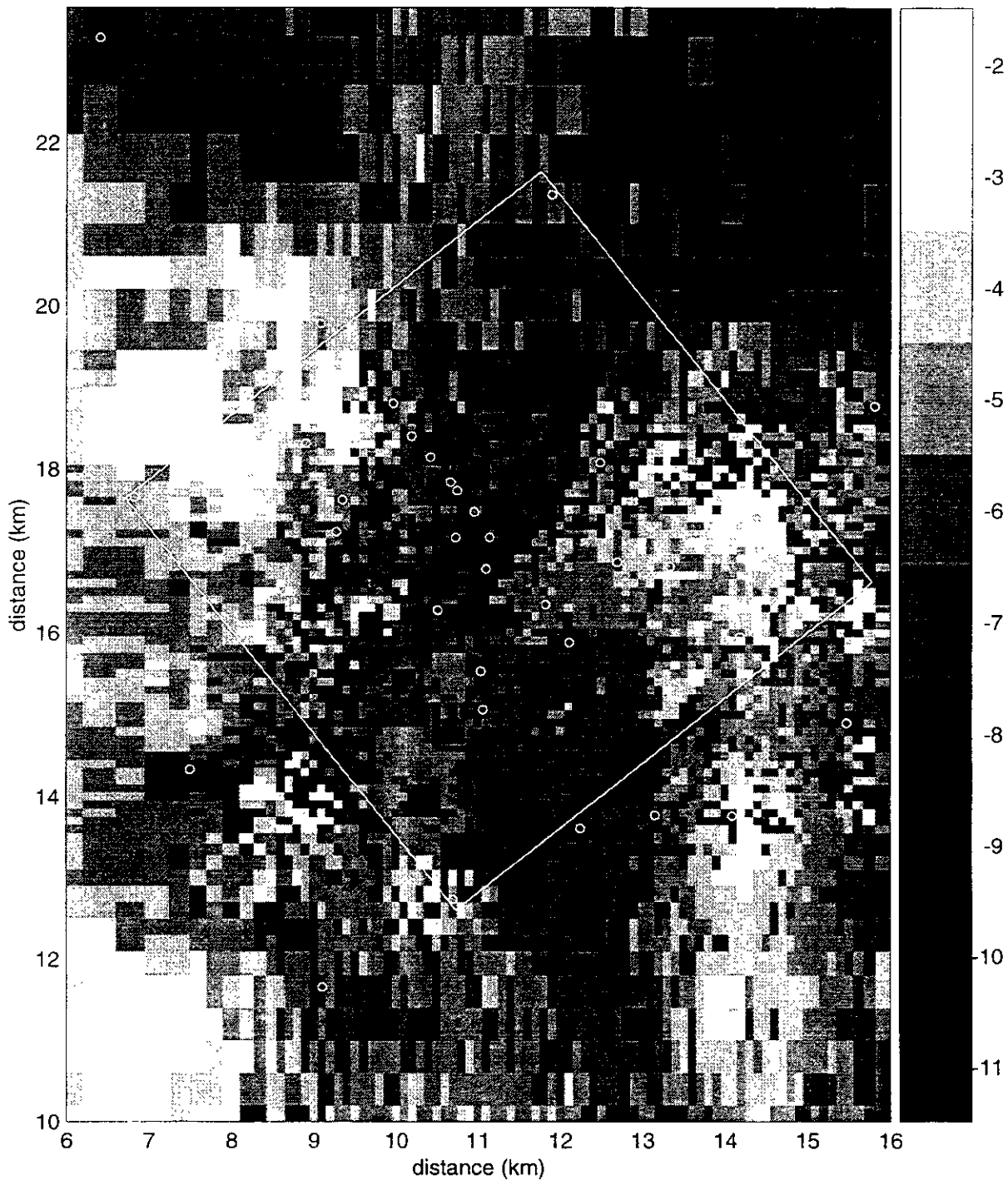
Figure TFIELD-A-122. Transient Calibrated Transmissivity Field no. 61, WIPP-scale.
