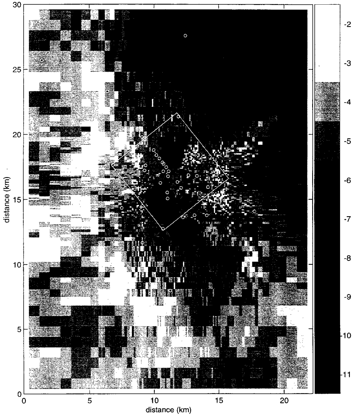
Figure TFIELD-A-41. Transient Calibrated Transmissivity Field no. 21, full-scale.
