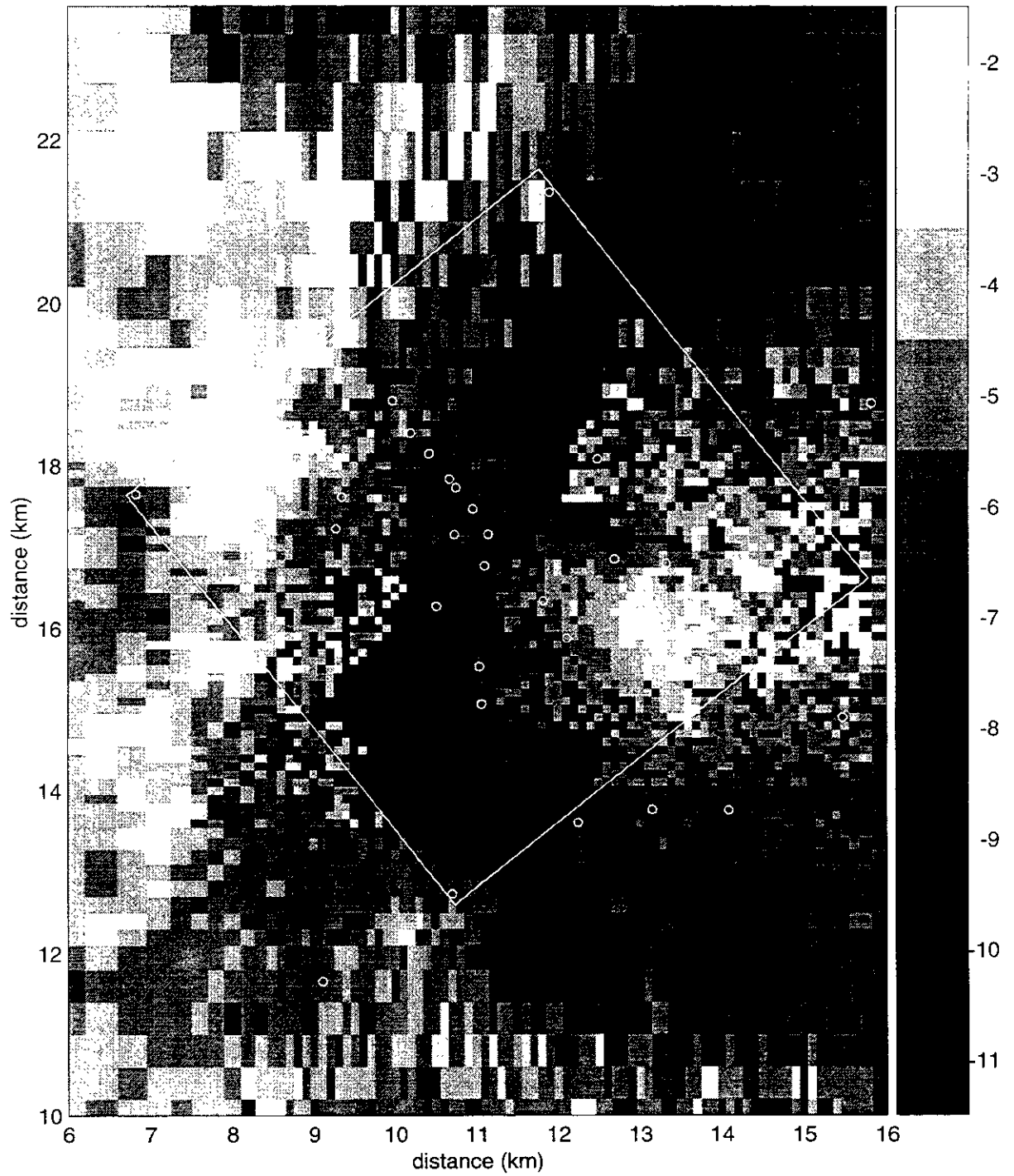
Figure TFIELD-A-176. Transient Calibrated Transmissivity Field no. 88, WIPP-scale.
