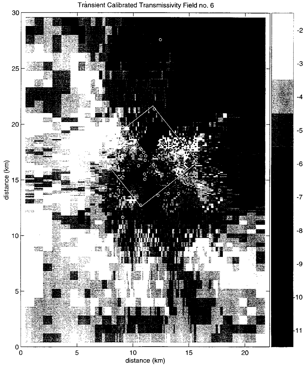
Figure TFIELD-A-11. Transient Calibrated Transmissivity Field no. 6, full-scale.
