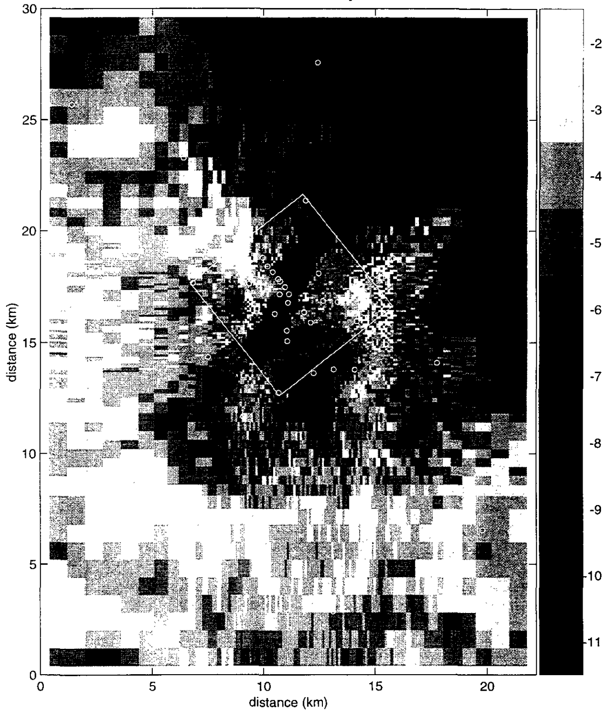
Figure TFIELD-A-157. Transient Calibrated Transmissivity Field no. 79, full-scale.
