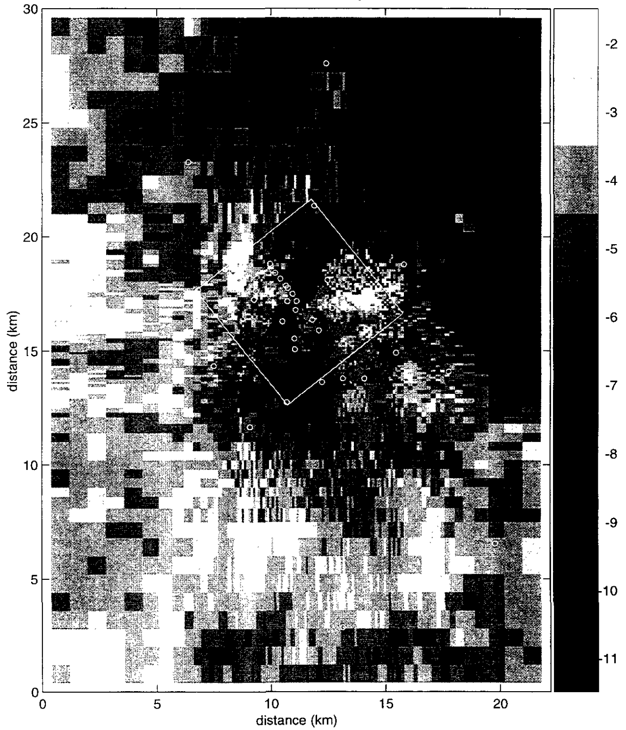
Figure TFIELD-A-165. Transient Calibrated Transmissivity Field no. 83, full-scale.
