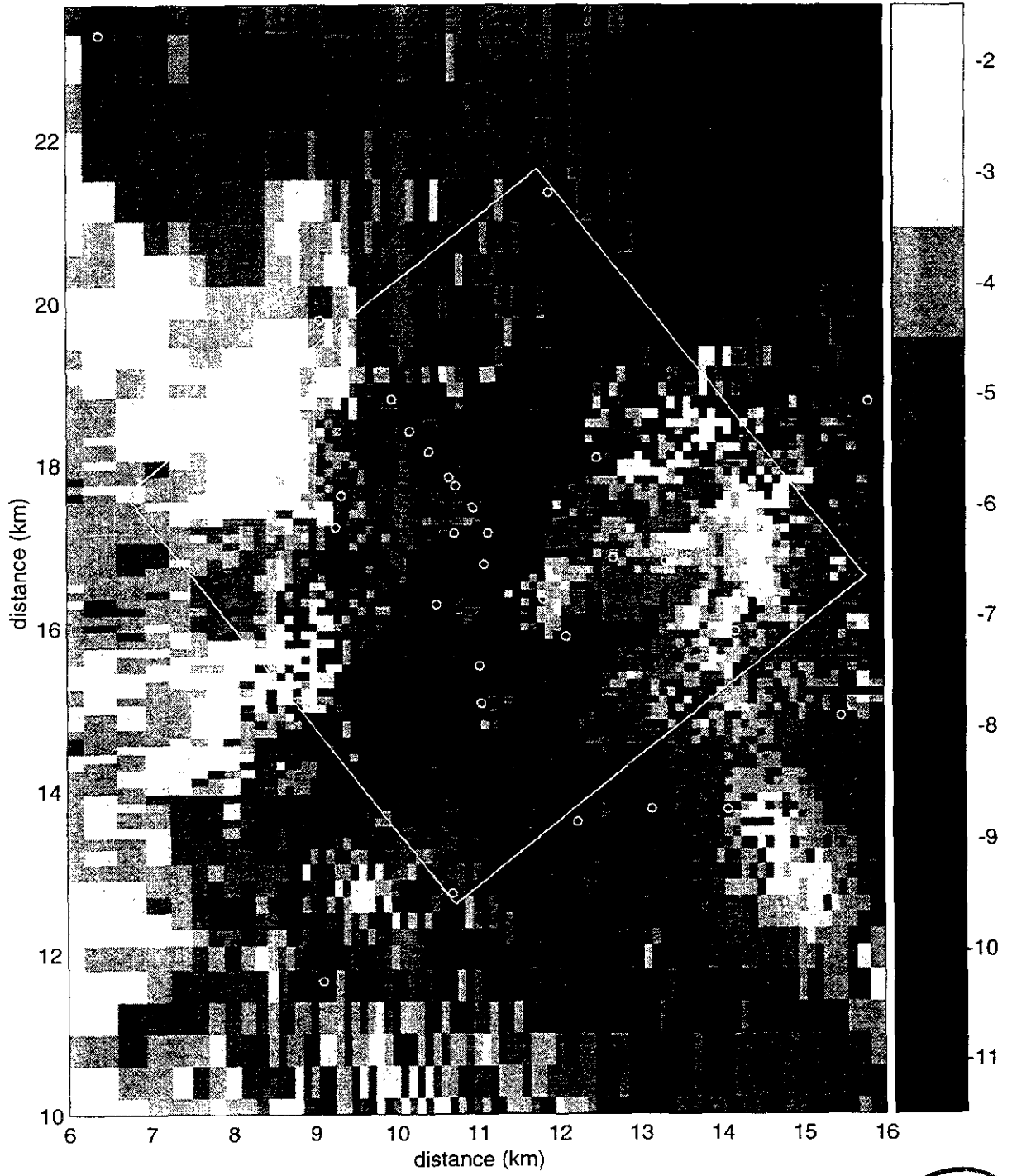
Figure TFIELD-A-8. Transient Calibrated Transmissivity Field no. 4, WIPP-scale.
