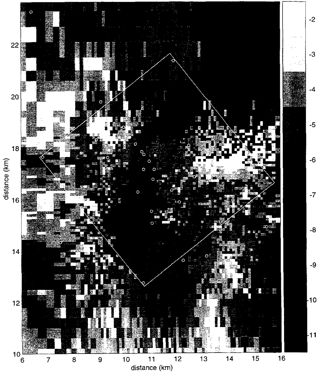
Figure TFIELD-A-40. Transient Calibrated Transmissivity Field no. 20, WIPP-scale.
