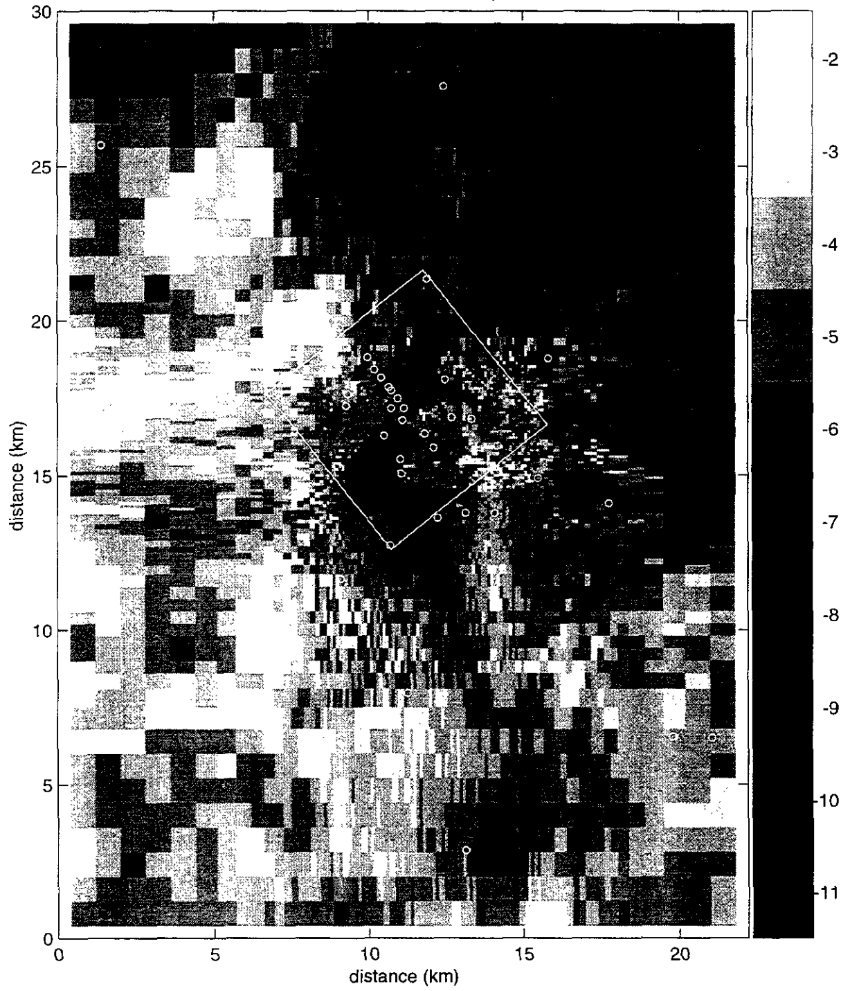
Figure TFIELD-A-5. Transient Calibrated Transmissivity Field no. 3, full-scale.
