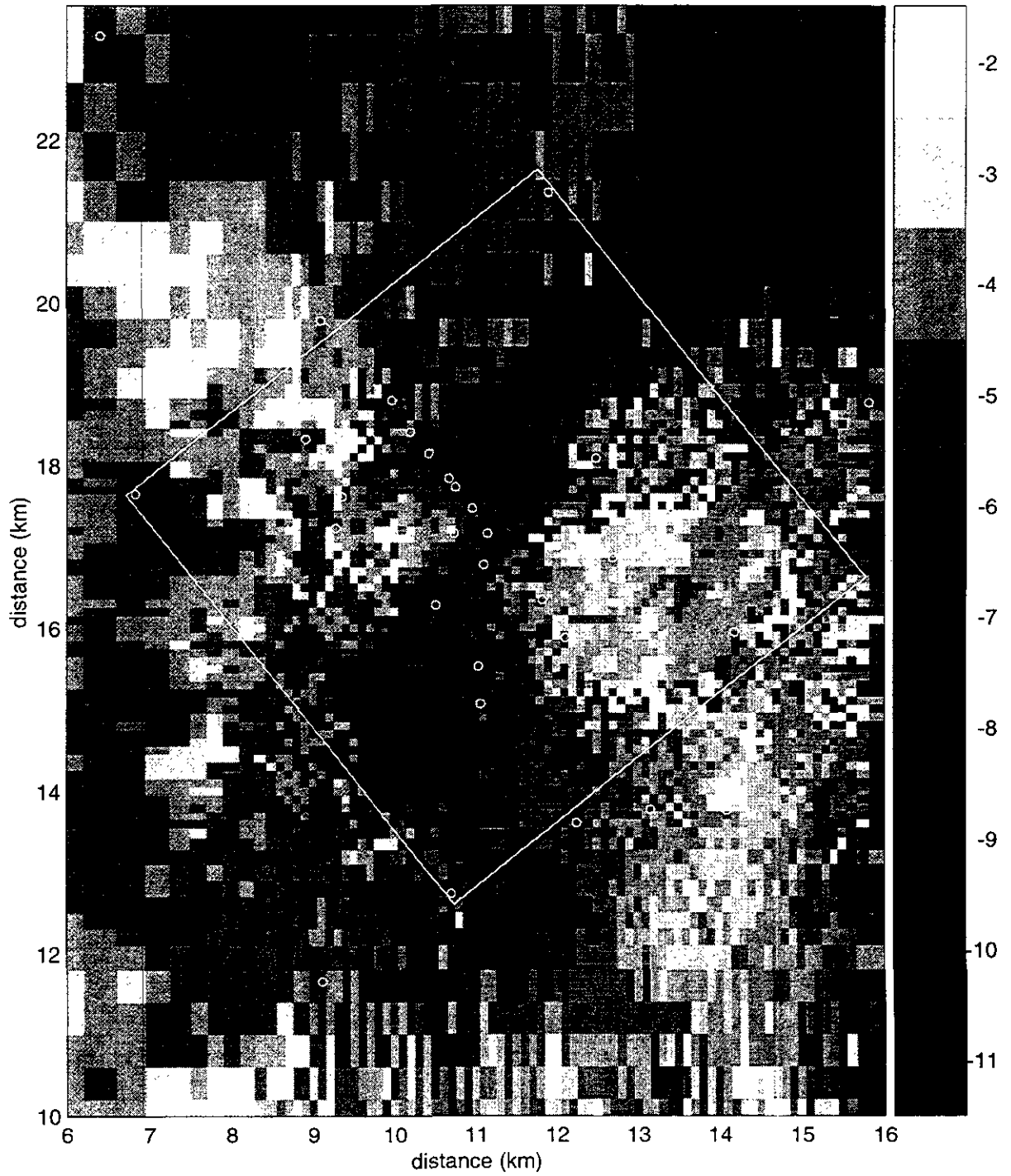
Figure TFIELD-A-90. Transient Calibrated Transmissivity Field no. 45, WIPP-scale.
