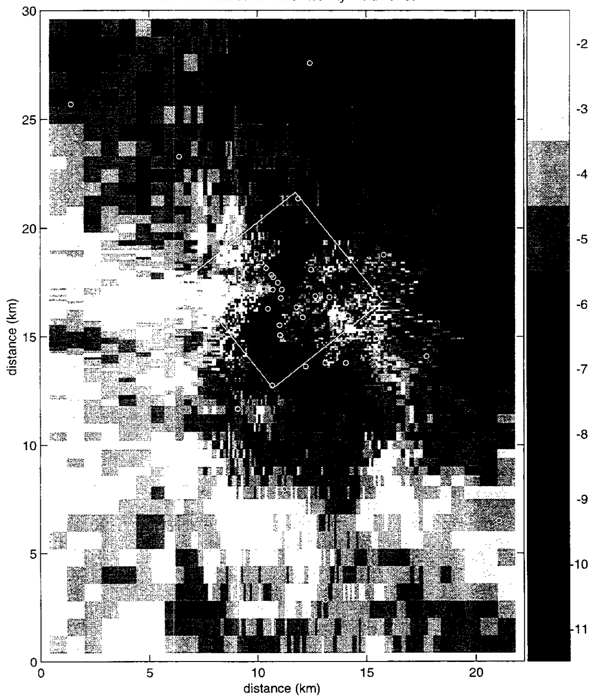
Figure TFIELD-A-49. Transient Calibrated Transmissivity Field no. 25, full-scale.
