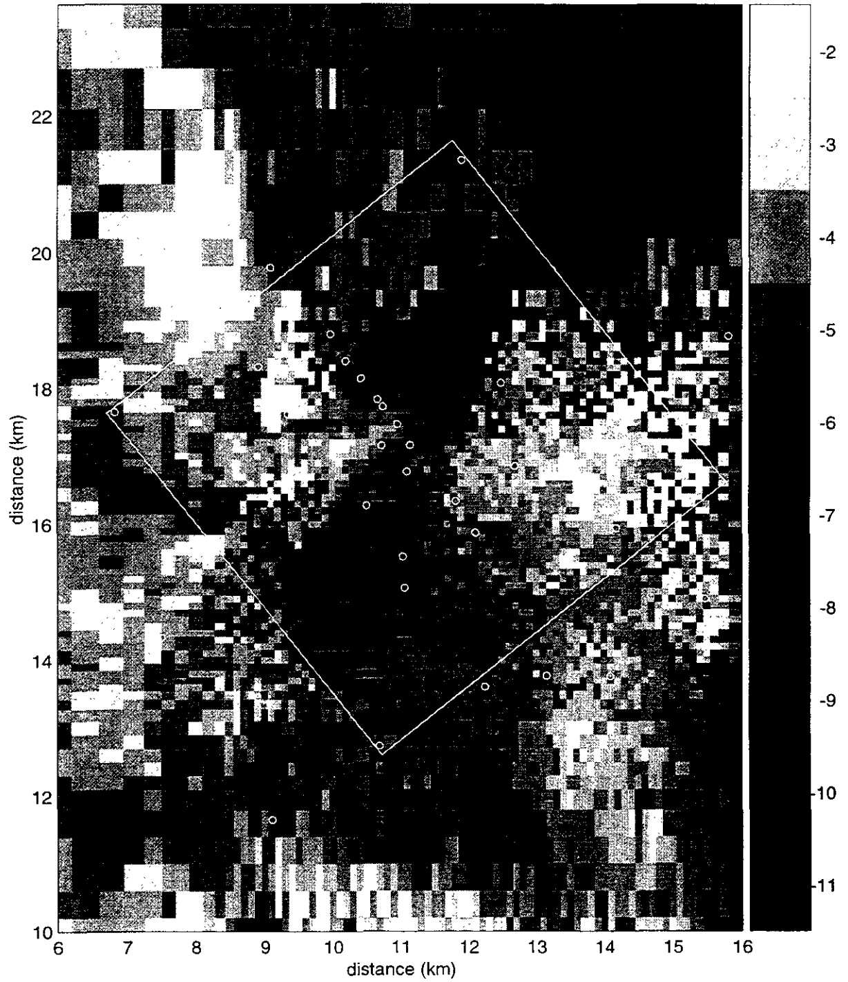
Figure TFIELD-A-70. Transient Calibrated Transmissivity Field no. 35, WIPP-scale.
