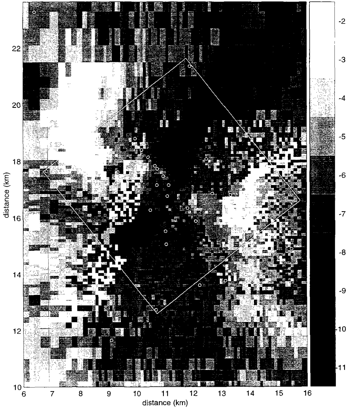
Figure TFIELD-A-104. Transient Calibrated Transmissivity Field no. 52, WIPP-scale.
