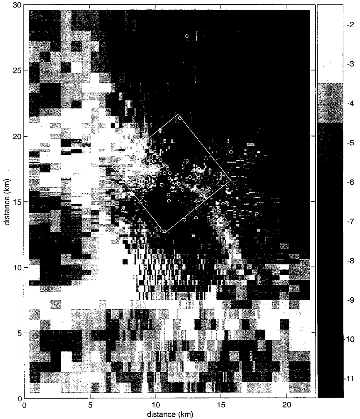
Figure TFIELD-A-79. Transient Calibrated Transmissivity Field no. 40, full-scale.
