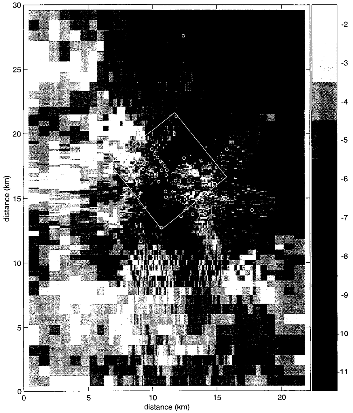
Figure TFIELD-A-151. Transient Calibrated Transmissivity Field no. 76, full-scale.
