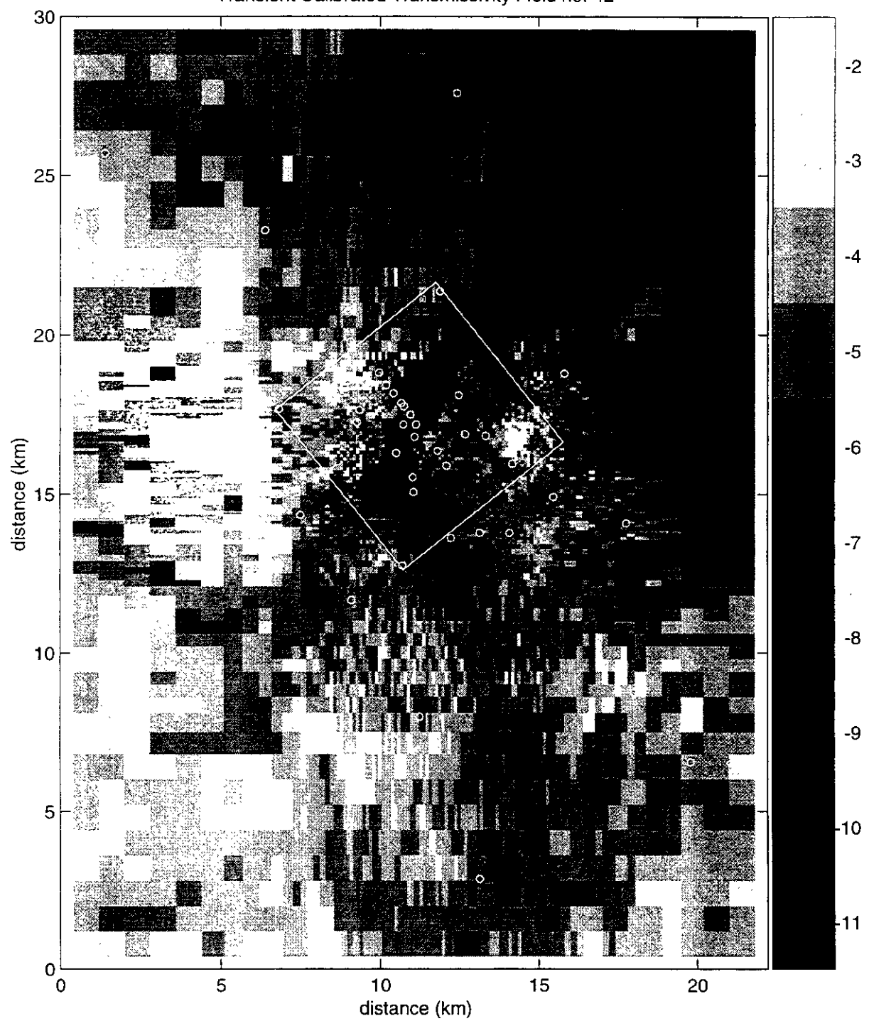
Figure TFIELD-A-83. Transient Calibrated Transmissivity Field no. 42, full-scale.
