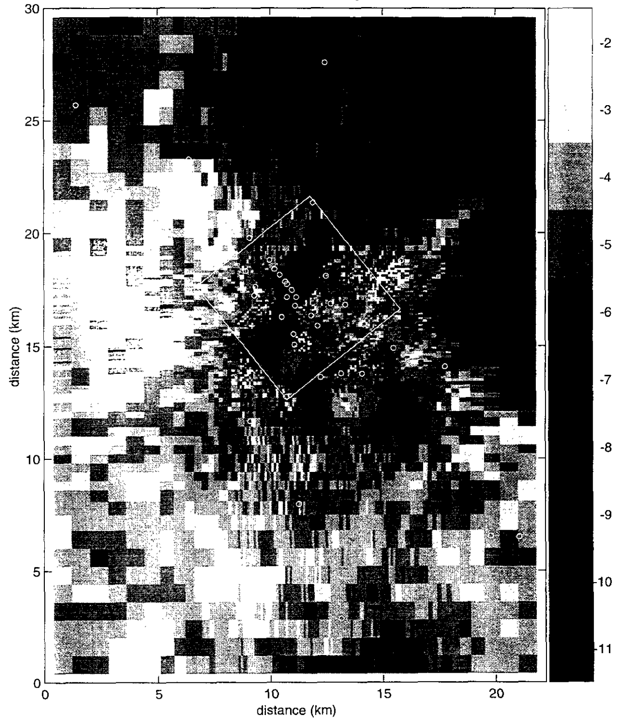
Figure TFIELD-A-119. Transient Calibrated Transmissivity Field no. 60, full-scale.
