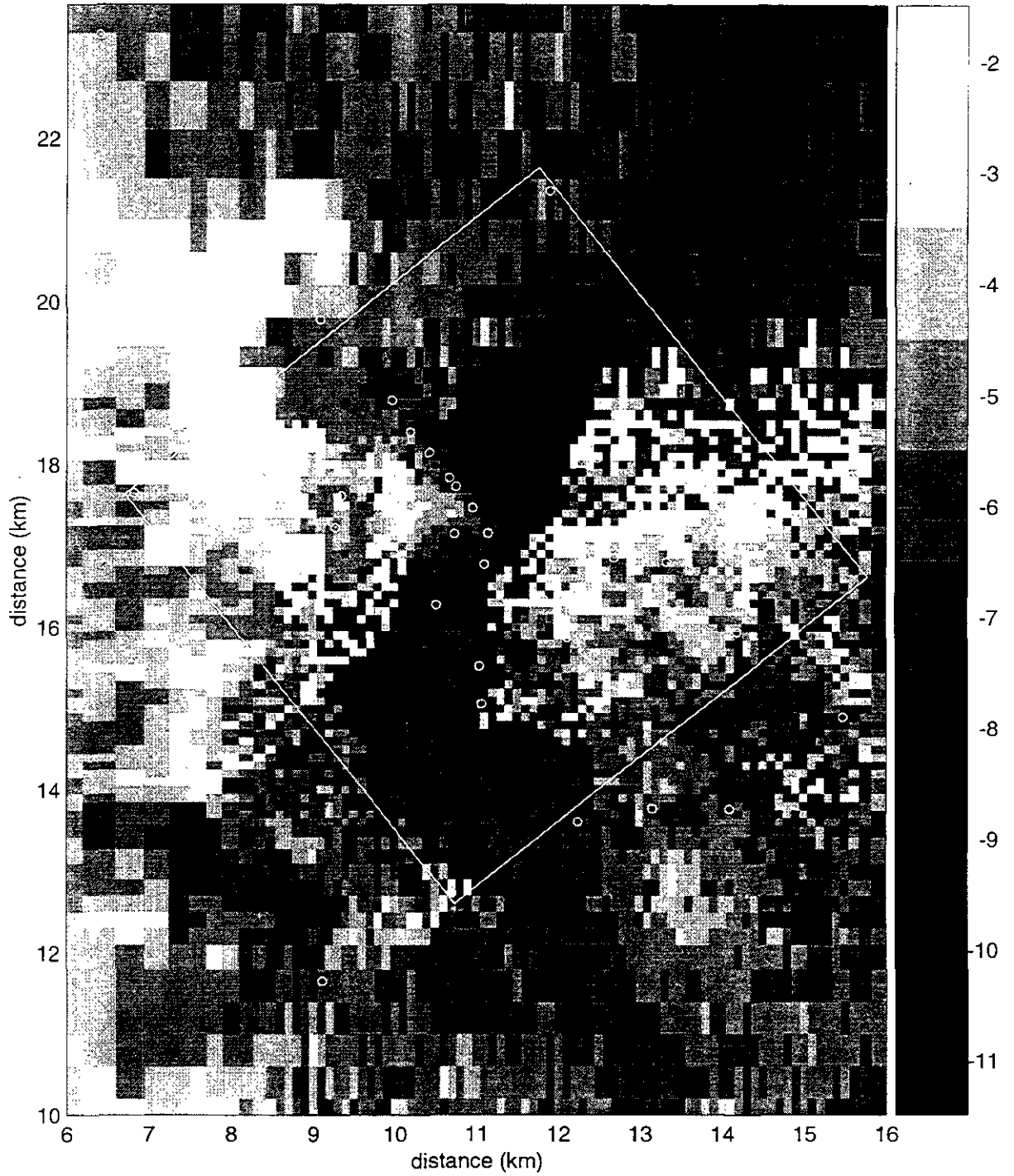
Figure TFIELD-A-134. Transient Calibrated Transmissivity Field no. 67, WIPP-scale.
