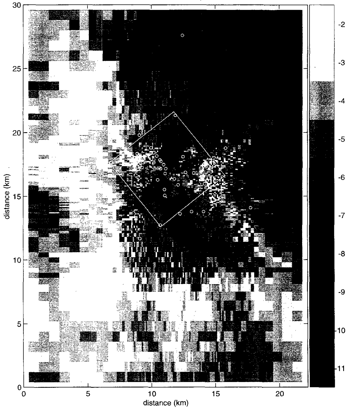
Figure TFIELD-A-63. Transient Calibrated Transmissivity Field no. 32, full-scale.
