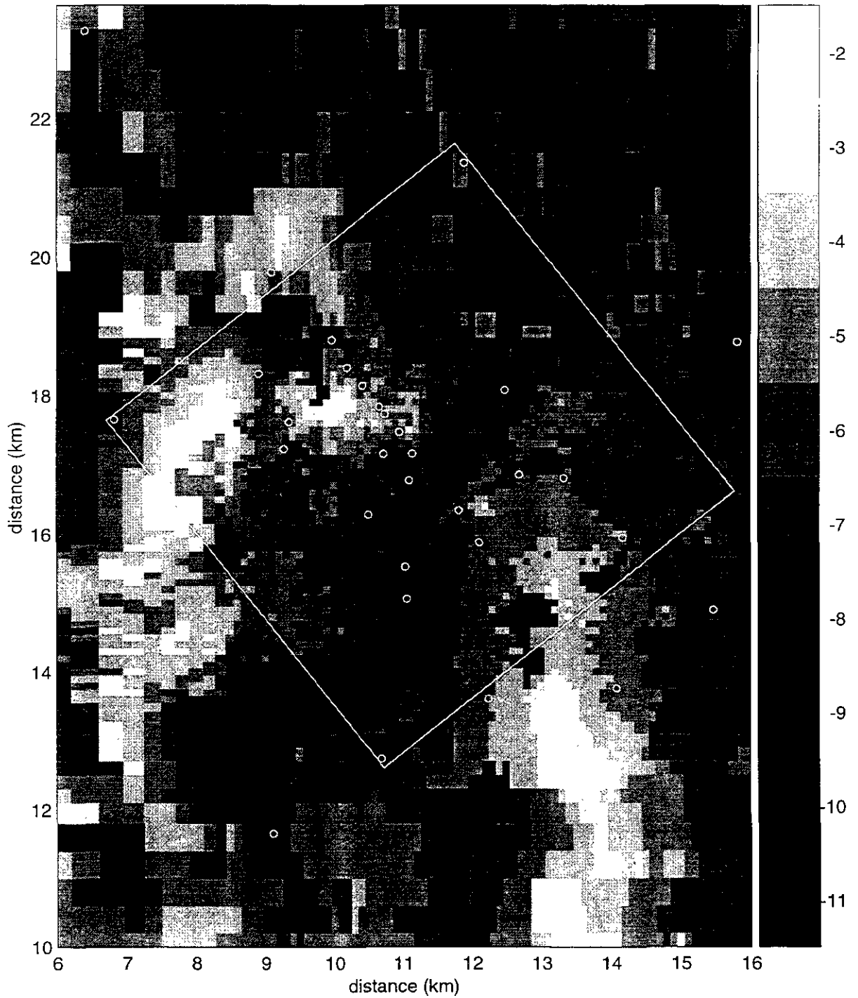
Figure TFIELD-A-150. Transient Calibrated Transmissivity Field no. 75, WIPP-scale.
