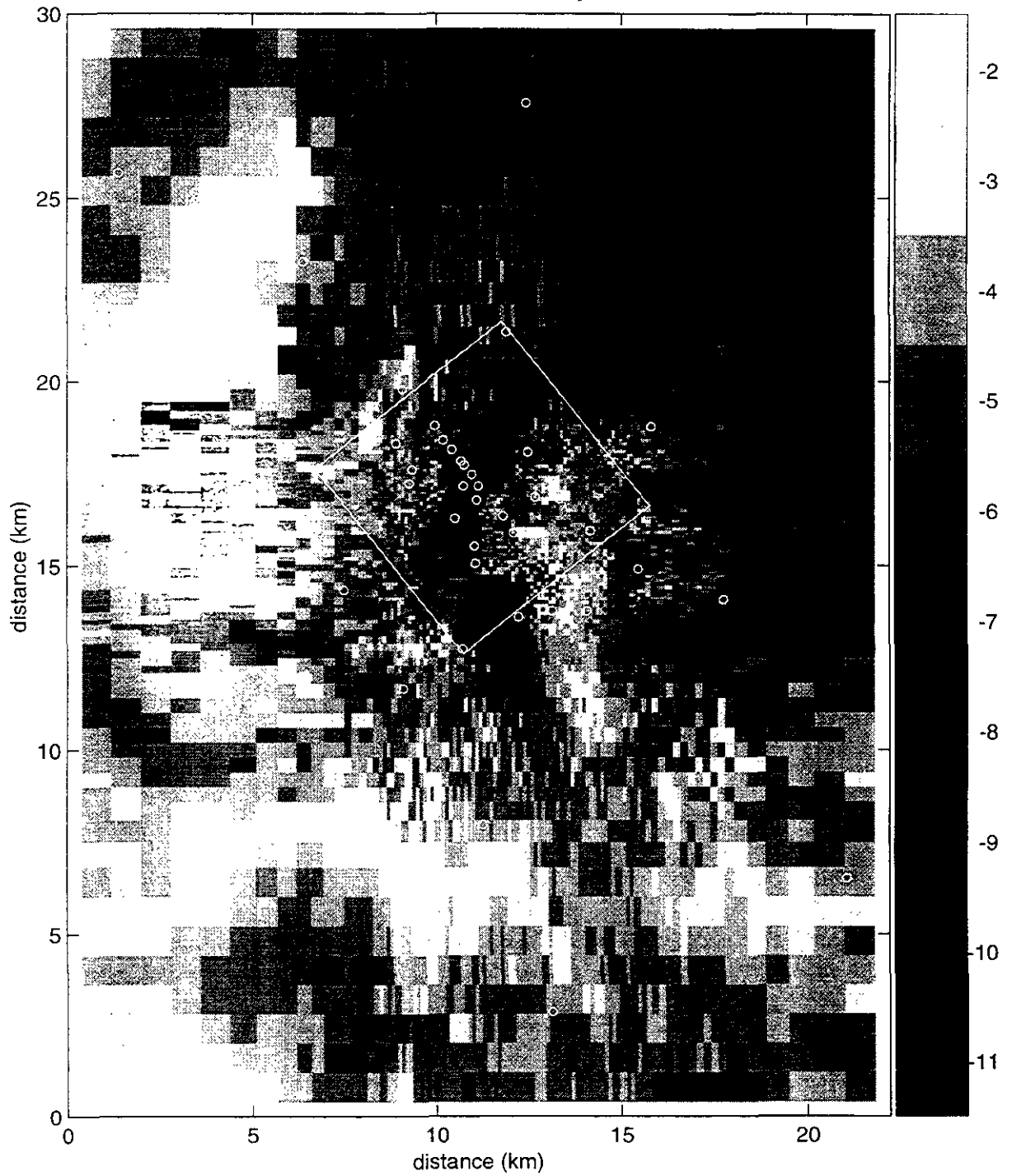
Figure TFIELD-A-105. Transient Calibrated Transmissivity Field no. 53, full-scale.
