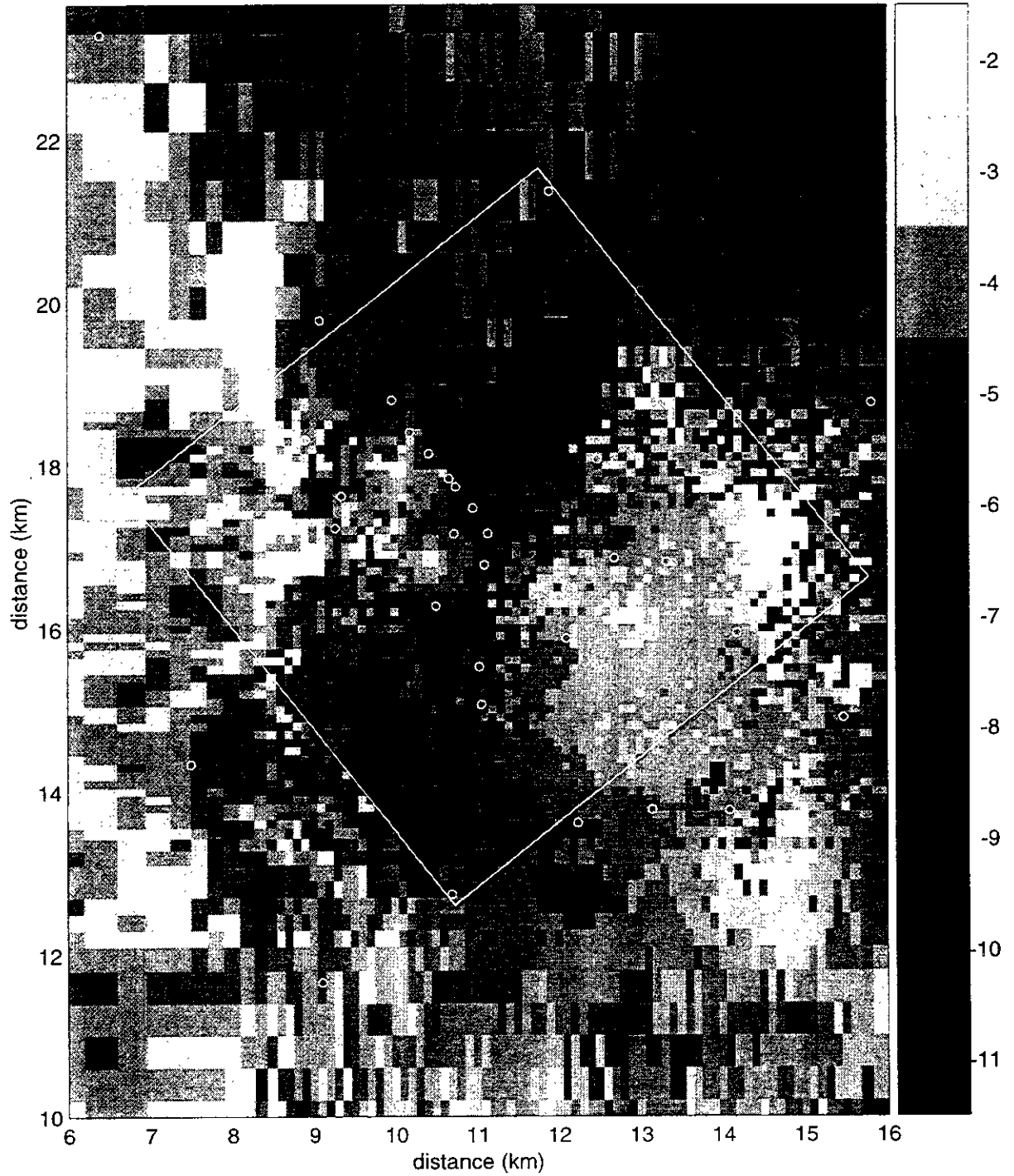
Figure TFIELD-A-98. Transient Calibrated Transmissivity Field no. 49, WIPP-scale.
