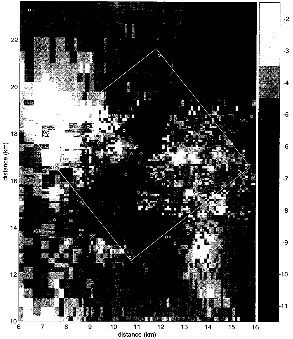
Figure TFIELD-A-20. Transient Calibrated Transmissivity Field no. 10, WIPP-scale.
