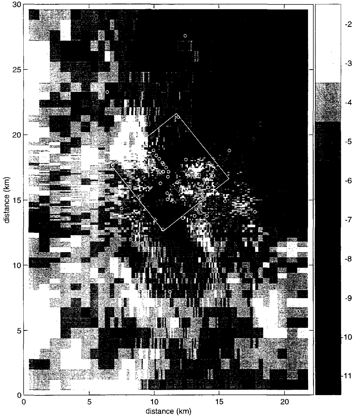
Figure TFIELD-A-87. Transient Calibrated Transmissivity Field no. 44, full-scale.
