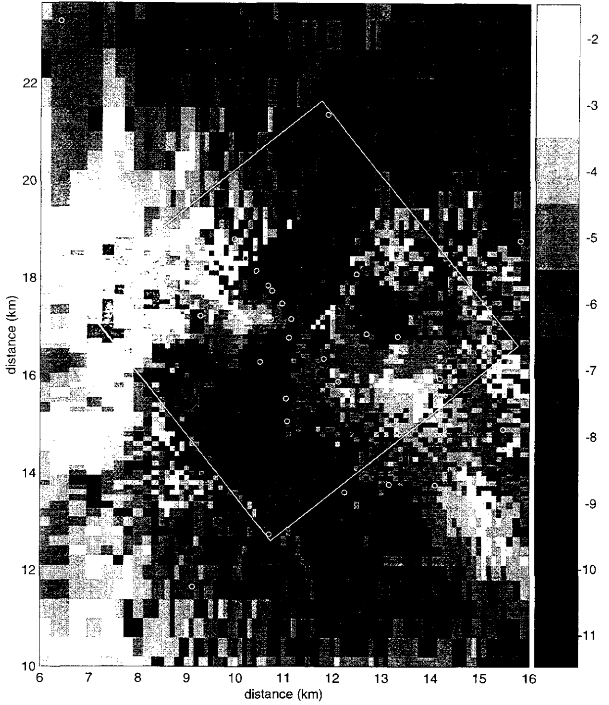
Figure TFIELD-A-172. Transient Calibrated Transmissivity Field no. 86, WIPP-scale.
