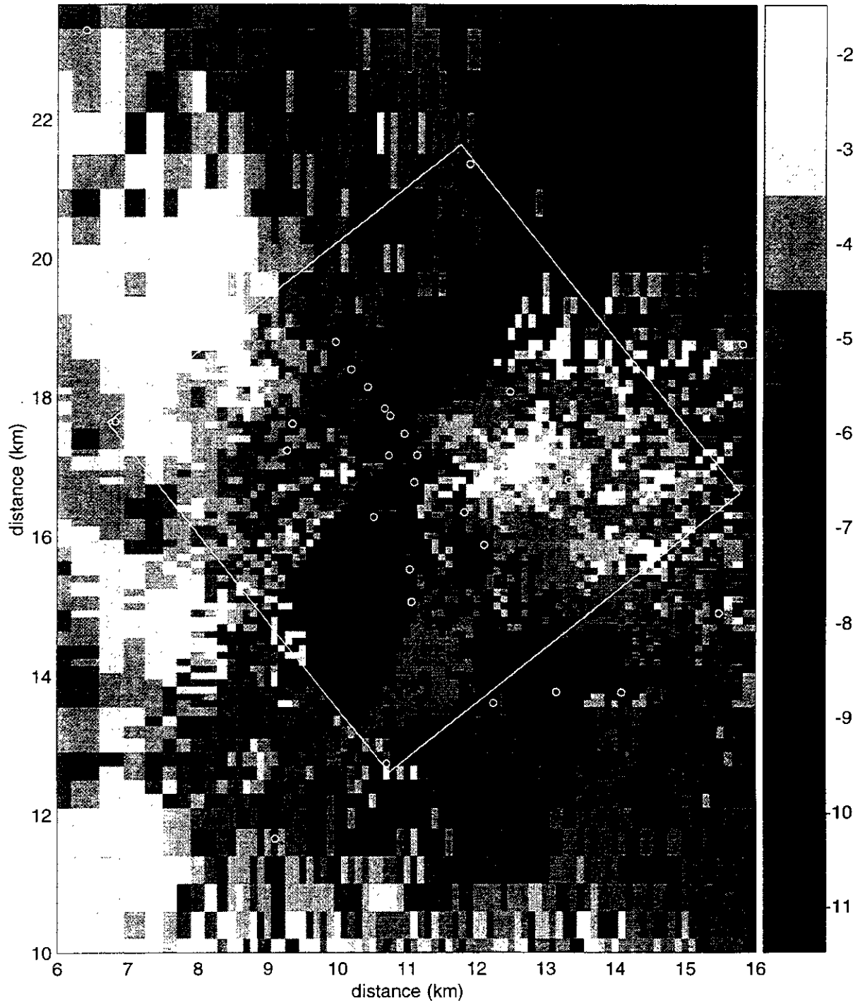
Figure TFIELD-A-44. Transient Calibrated Transmissivity Field no. 22, WIPP-scale.
