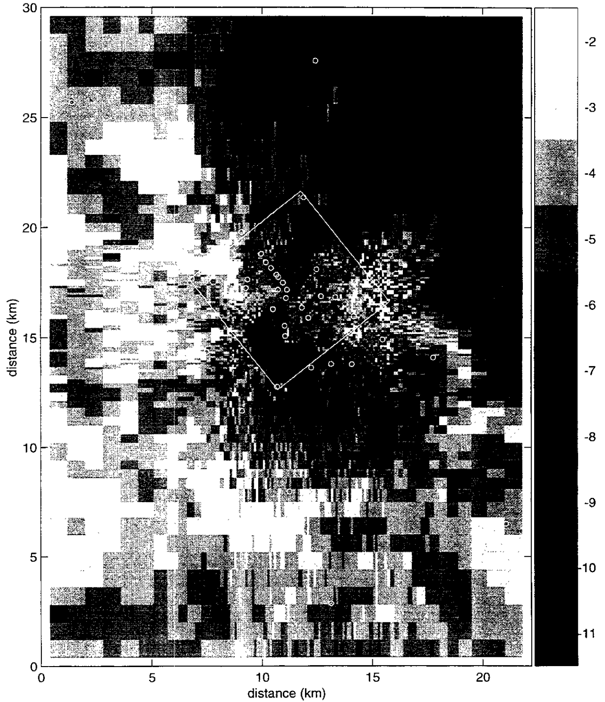
Figure TFIELD-A-59. Transient Calibrated Transmissivity Field no. 30, full-scale.
