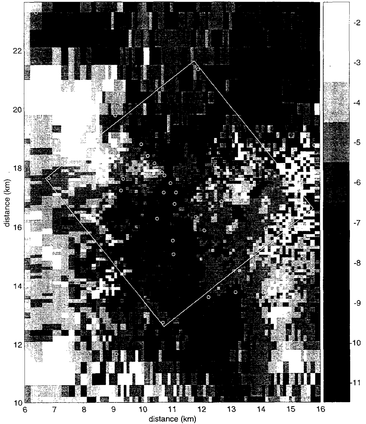
Figure TFIELD-A-164. Transient Calibrated Transmissivity Field no. 82, WIPP-scale.
