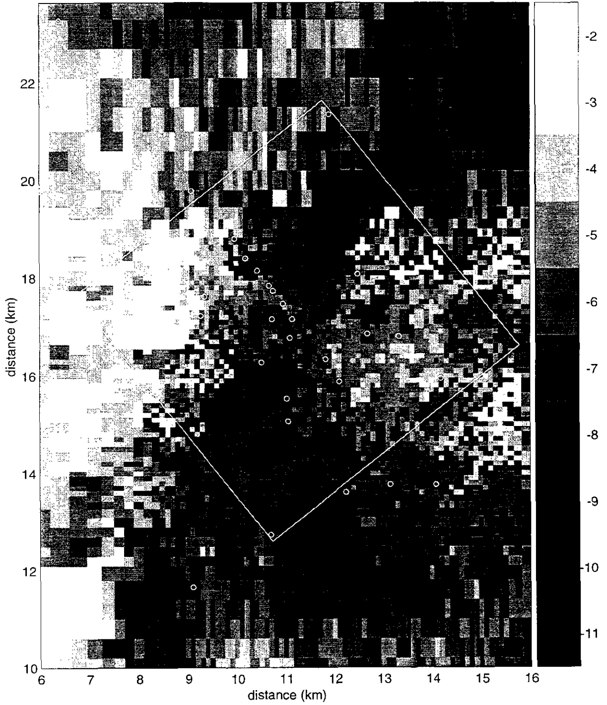
Figure TFIELD-A-132. Transient Calibrated Transmissivity Field no. 66, WIPP-scale.
