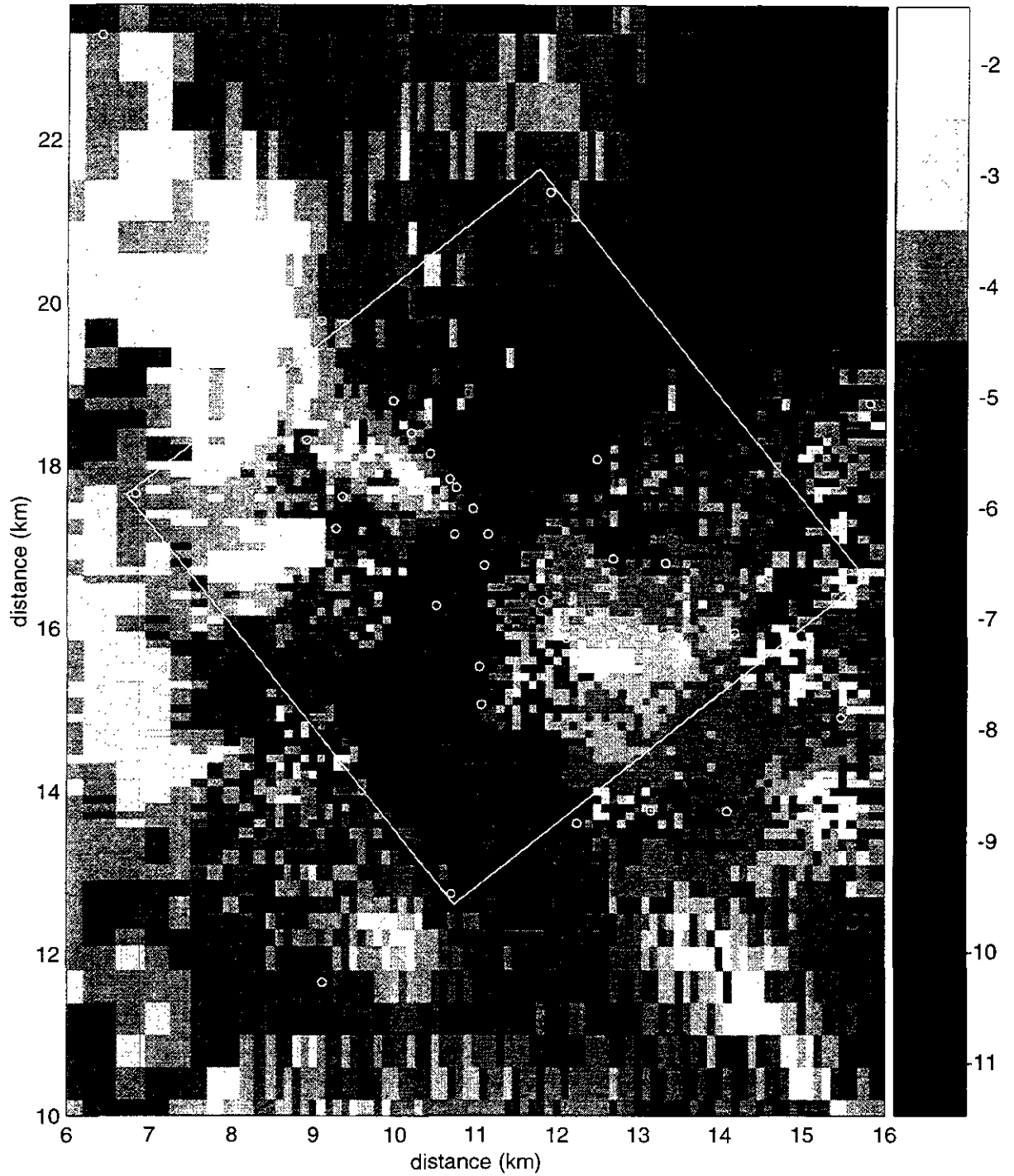
Figure TFIELD-A-52. Transient Calibrated Transmissivity Field no. 26, WIPP-scale.
