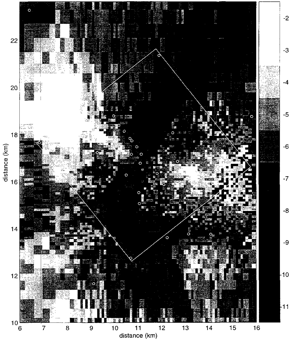
Figure TFIELD-A-126. Transient Calibrated Transmissivity Field no. 63, WIPP-scale.
