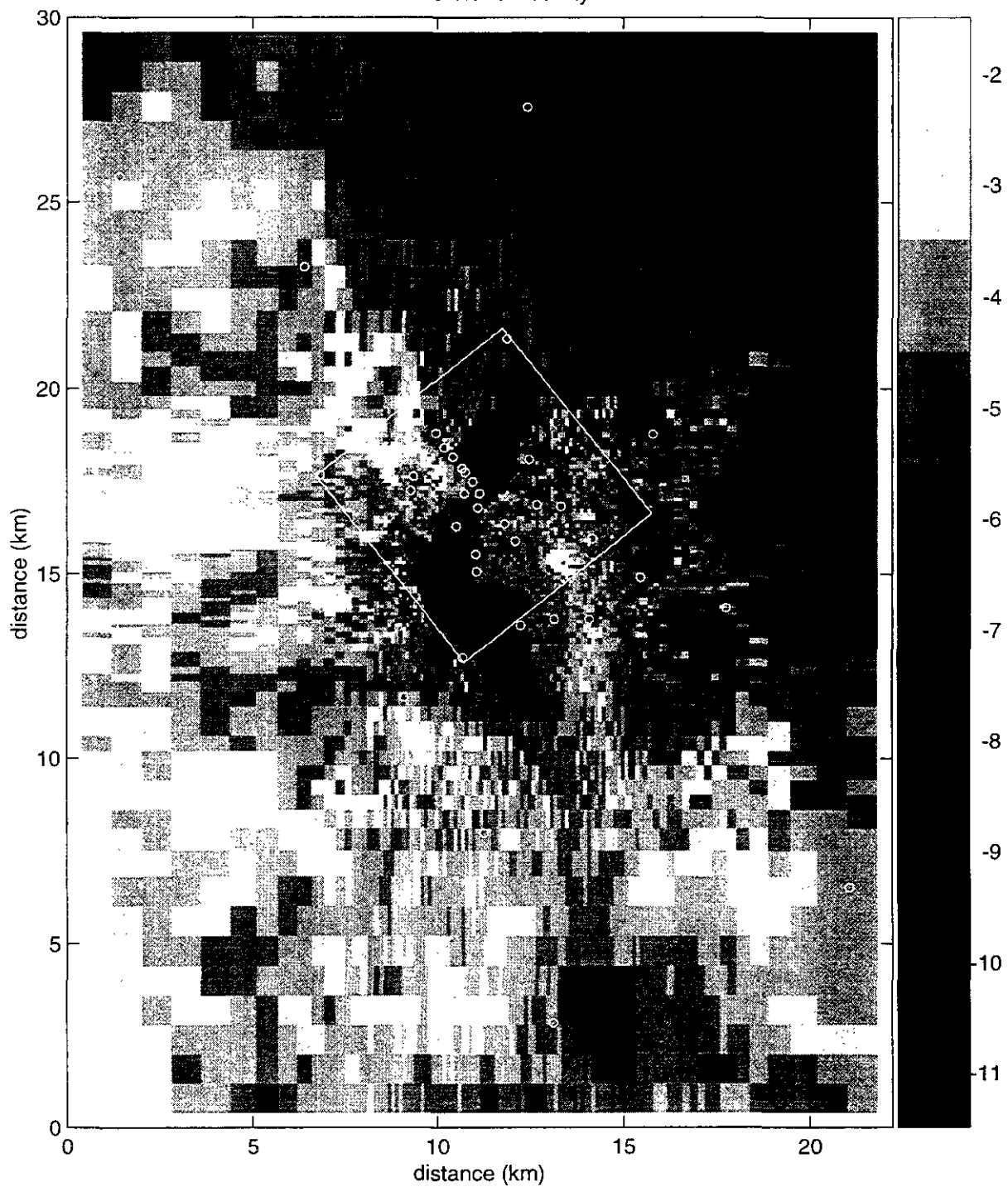
Figure TFIELD-A-185. Transient Calibrated Transmissivity Field no. 93, full-scale.
