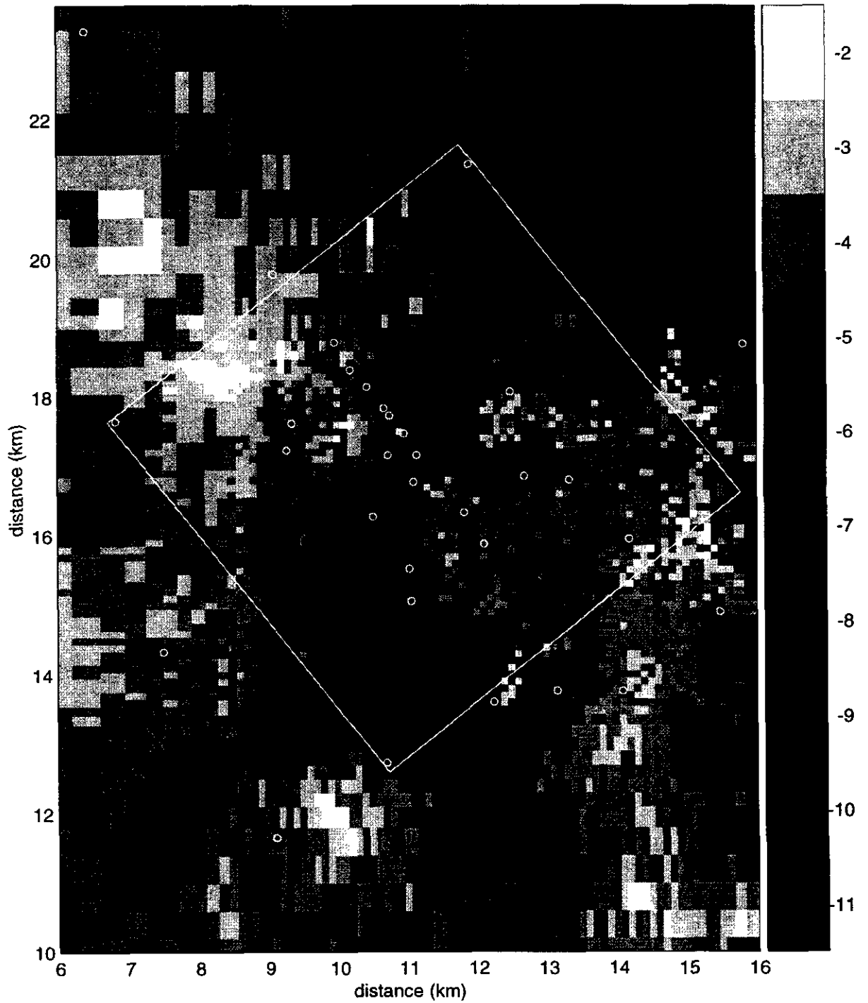
Figure TFIELD-A-16. Transient Calibrated Transmissivity Field no. 8, WIPP-scale.
