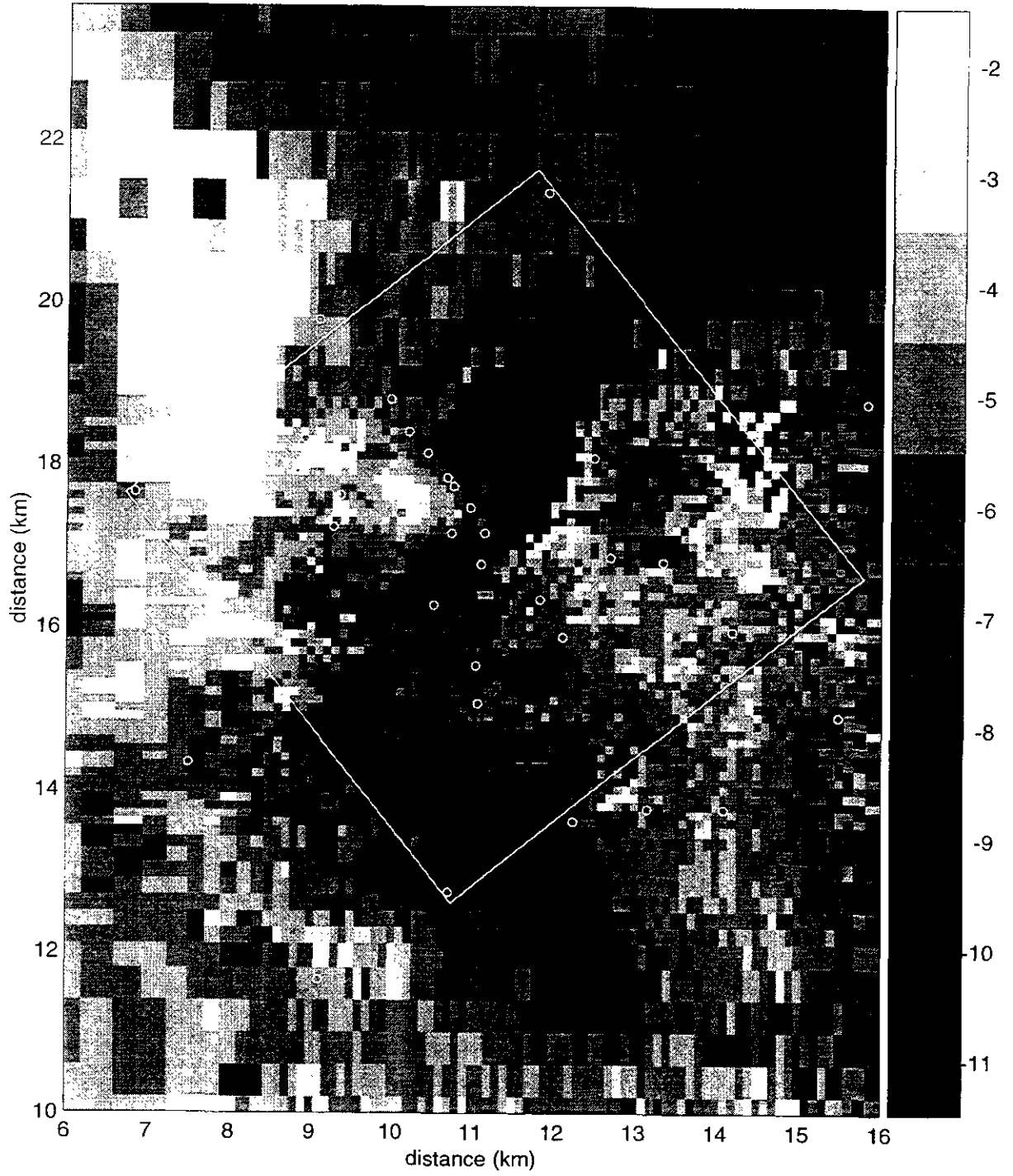
Figure TFIELD-A-180. Transient Calibrated Transmissivity Field no. 90, WIPP-scale.
