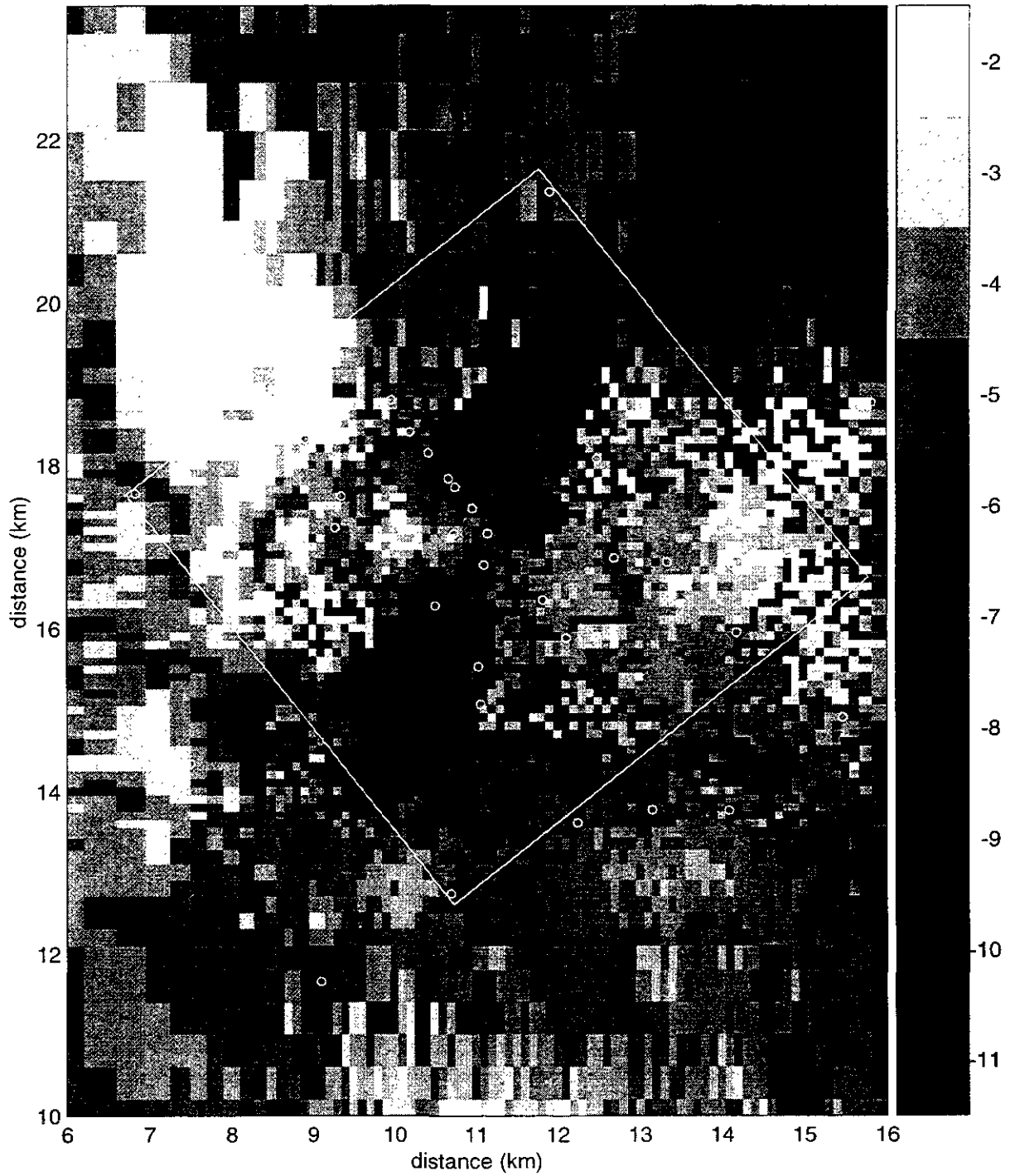
Figure TFIELD-A-82. Transient Calibrated Transmissivity Field no. 41, WIPP-scale.
