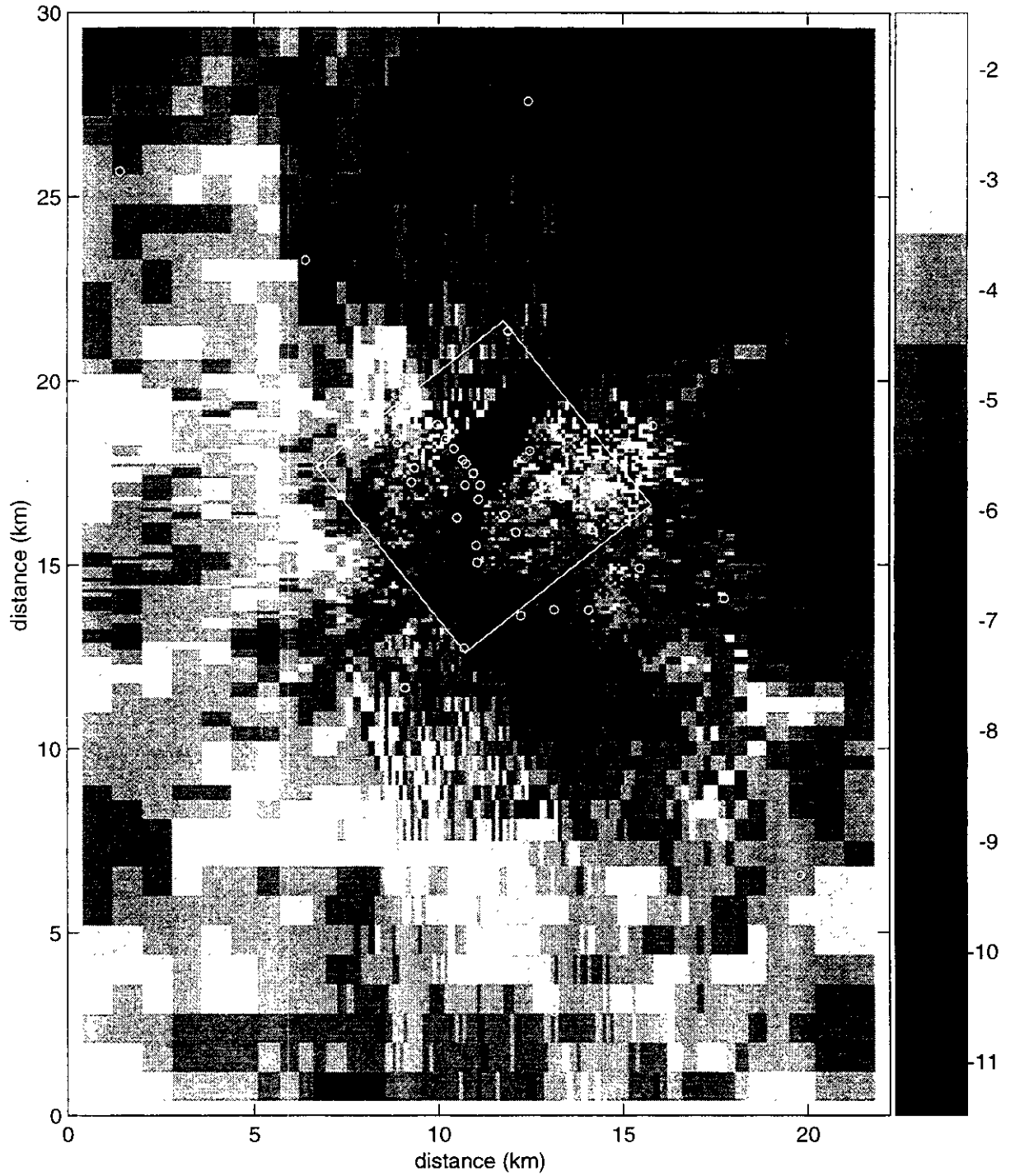
Figure TFIELD-A-73. Transient Calibrated Transmissivity Field no. 37, full-scale.
