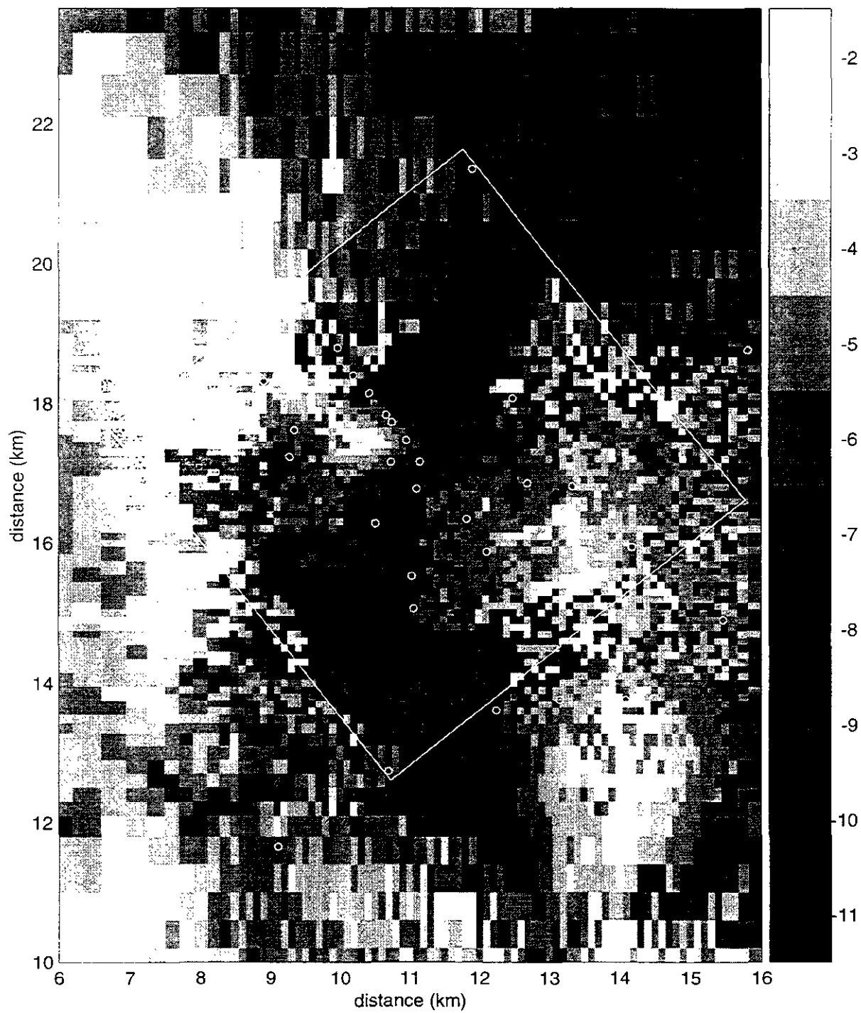
Figure TFIELD-A-162. Transient Calibrated Transmissivity Field no. 81, WIPP-scale.
