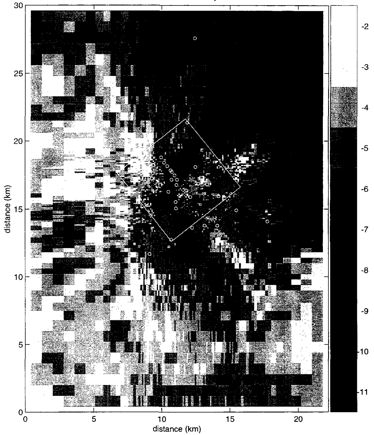
Figure TFIELD-A-71. Transient Calibrated Transmissivity Field no. 36, full-scale.
