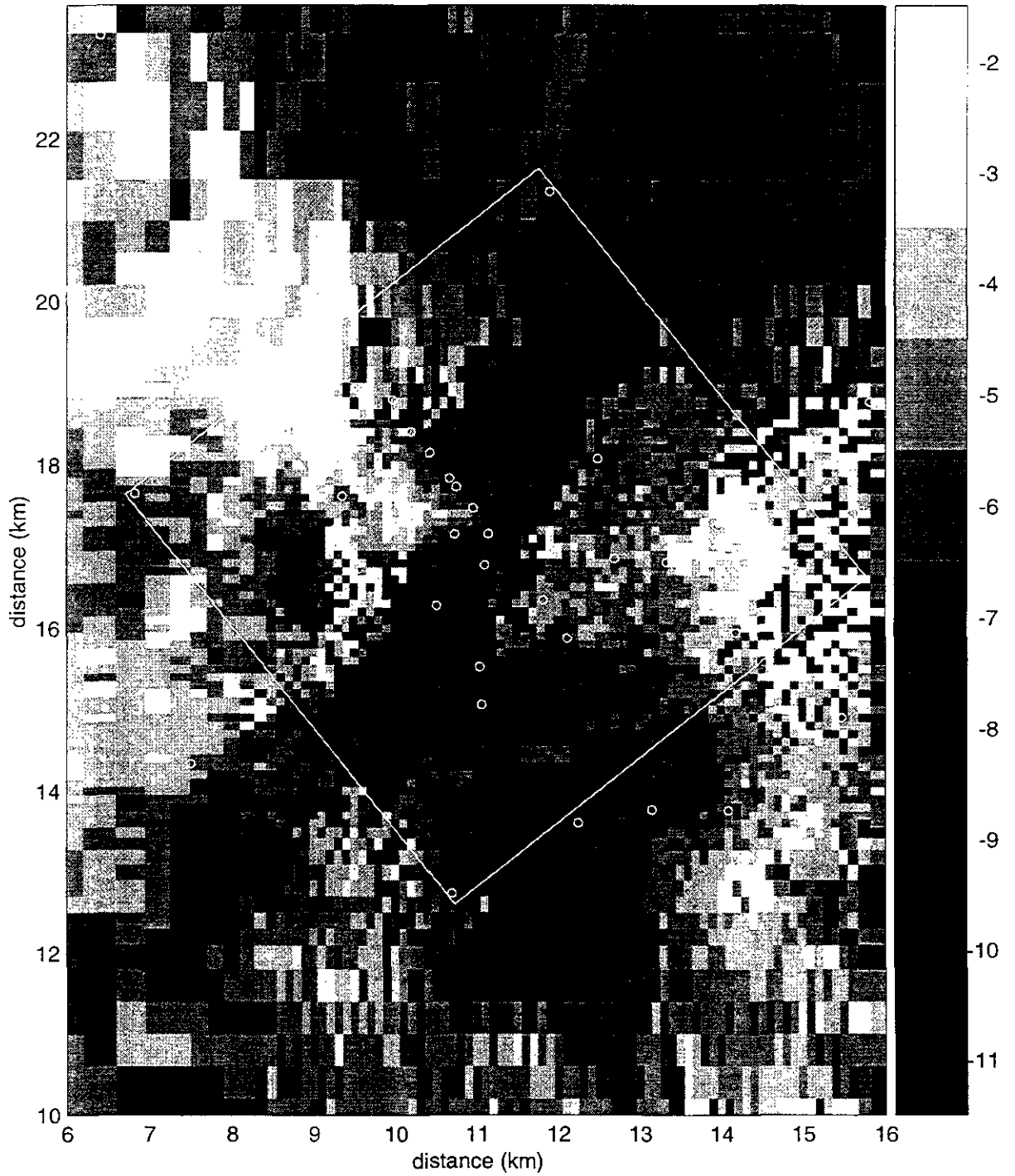
Figure TFIELD-A-158. Transient Calibrated Transmissivity Field no. 79, WIPP-scale.
