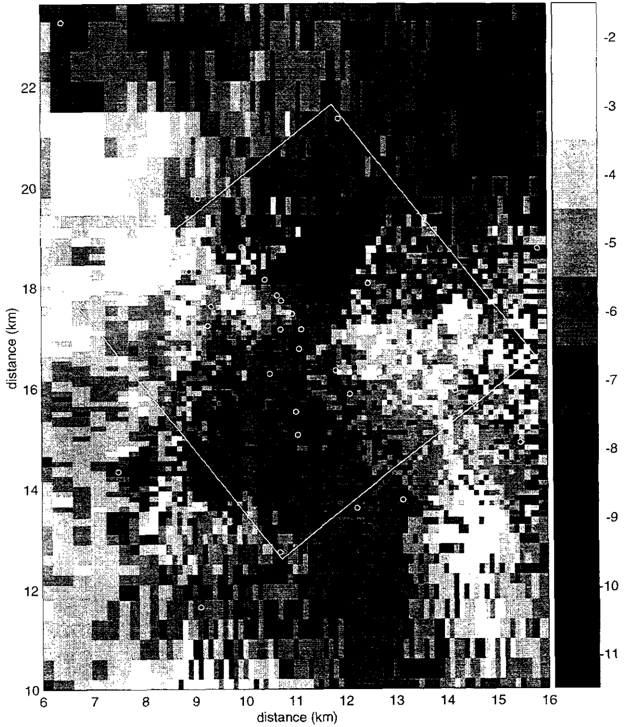
Figure TFIELD-A-116. Transient Calibrated Transmissivity Field no. 58, WIPP-scale.
