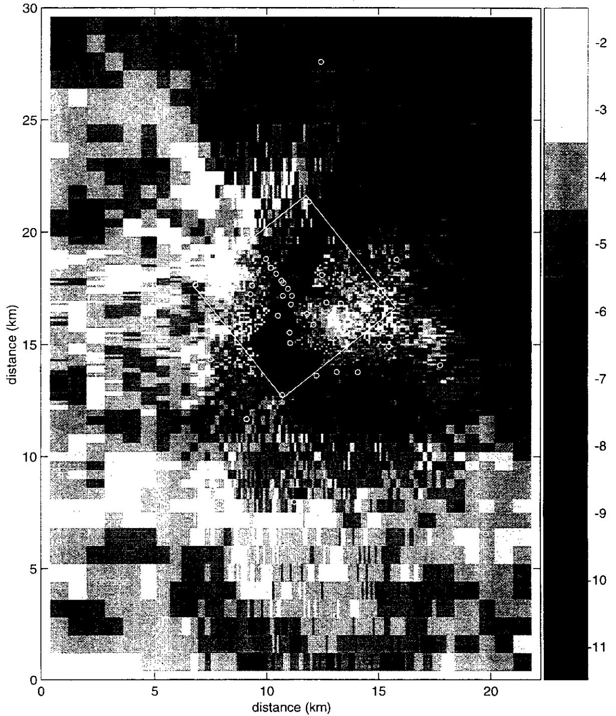
Figure TFIELD-A-175. Transient Calibrated Transmissivity Field no. 88, full-scale.
