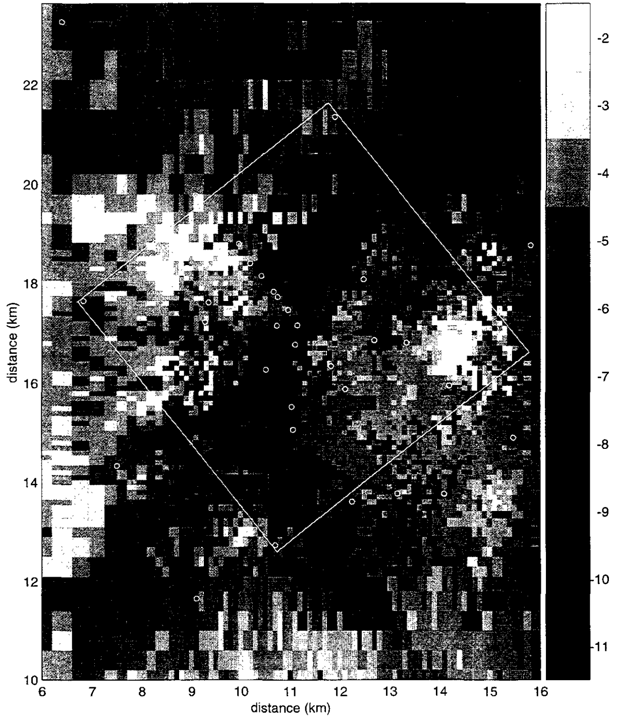
Figure TFIELD-A-84. Transient Calibrated Transmissivity Field no. 42, WIPP-scale.
