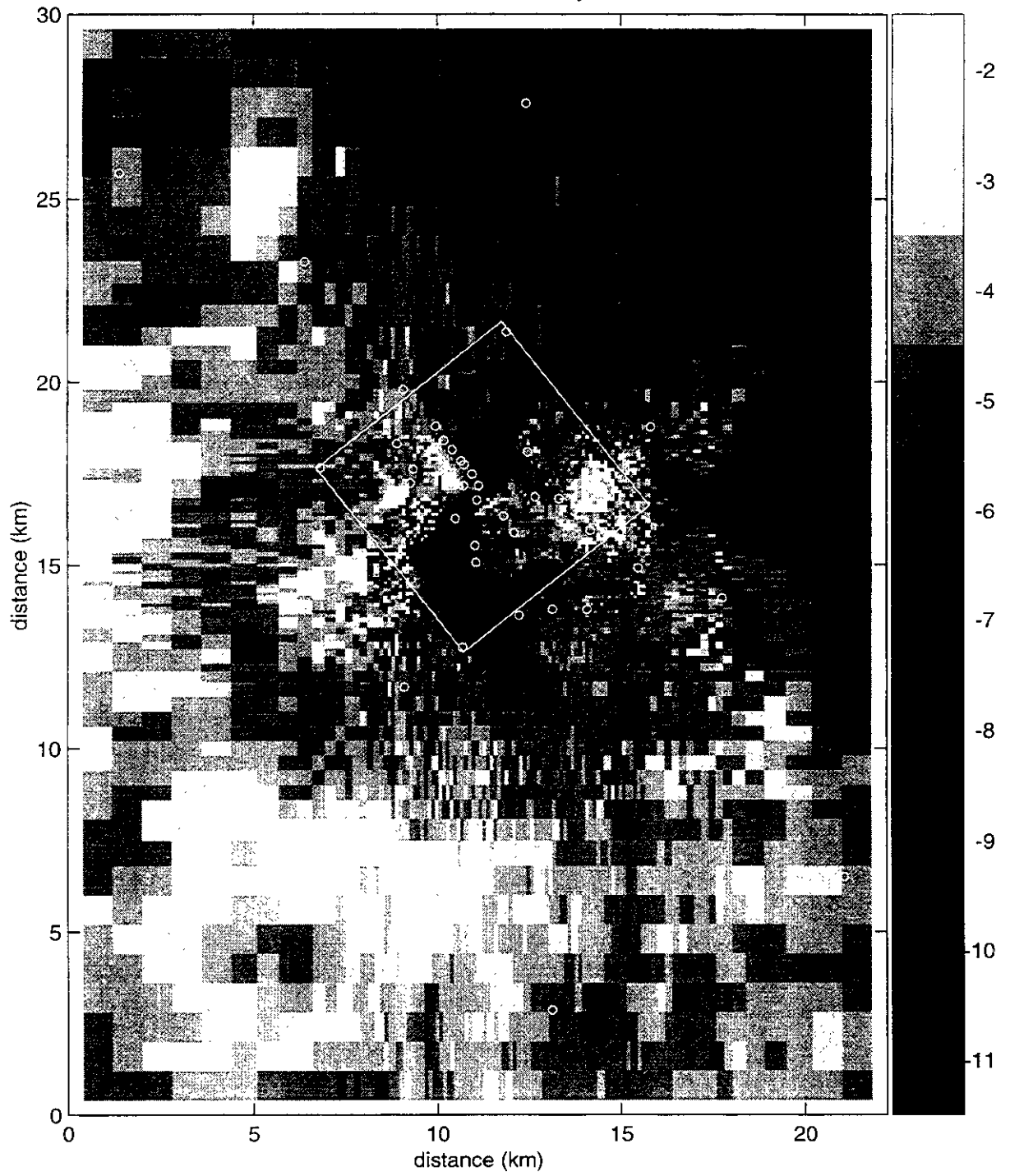
Figure TFIELD-A-169. Transient Calibrated Transmissivity Field no. 85, full-scale.
