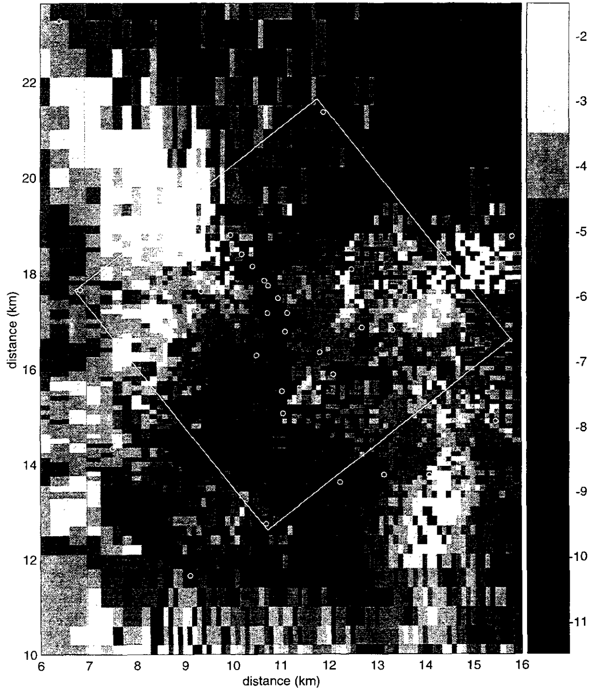
Figure TFIELD-A-30. Transient Calibrated Transmissivity Field no. 15, WIPP-scale.
