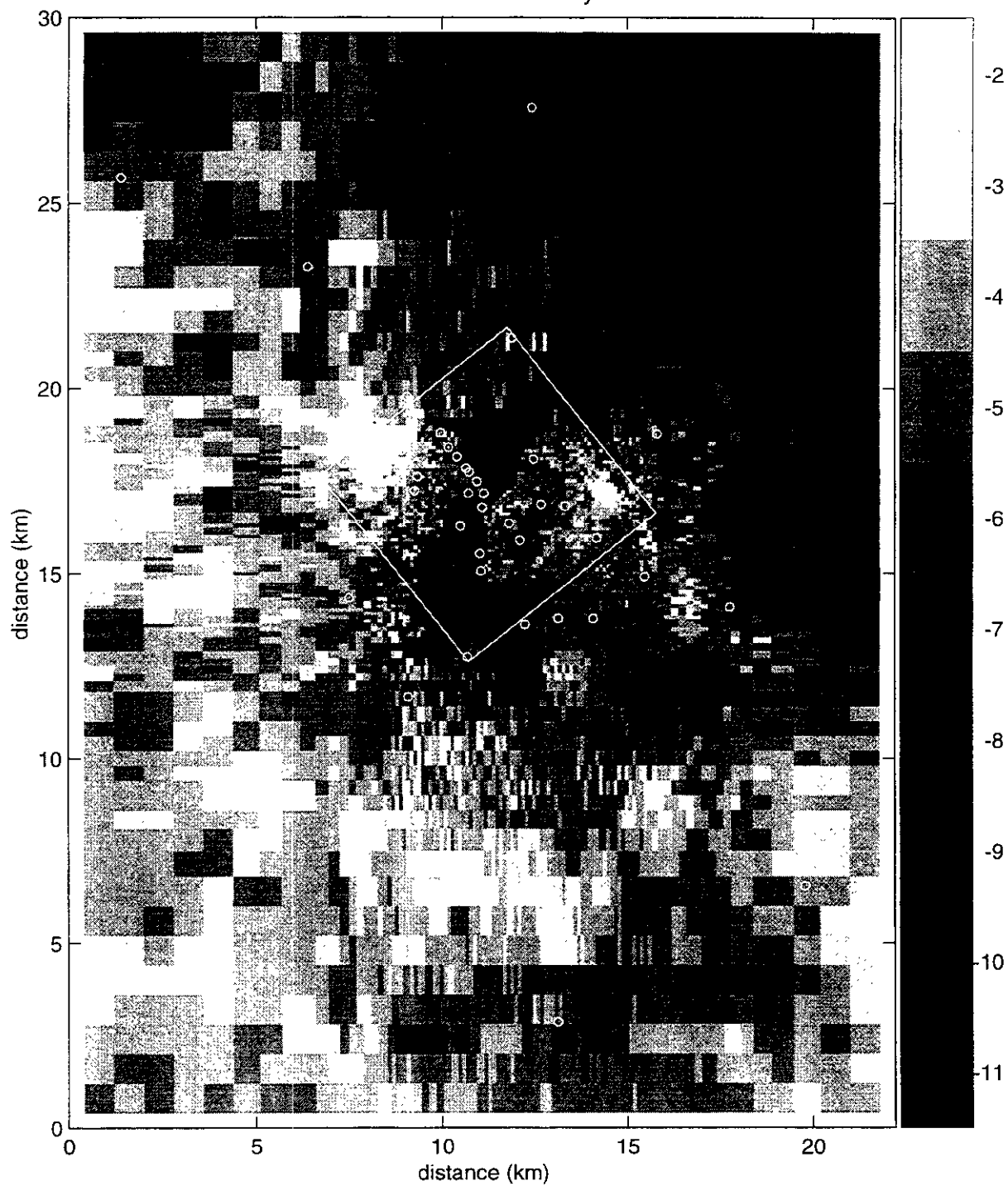
Figure TFIELD-A-21. Transient Calibrated Transmissivity Field no. 11, full-scale.
