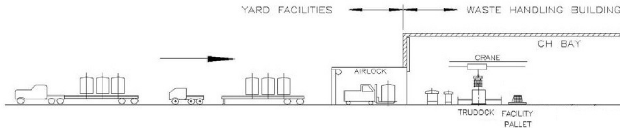
FIGURE 3-2. GENERAL WASTE HANDLING PROCESS FOR CH TRU MIXED WASTE OPERATIONS
