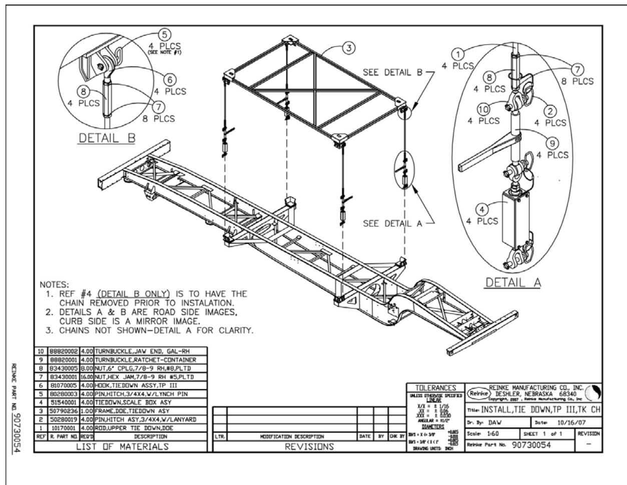
Figure 4.3.1-1 – TRUPACT-III Tiedown Frame
